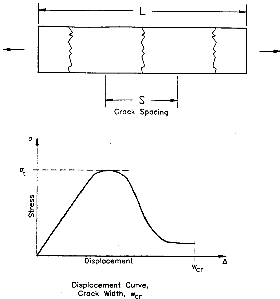
Figure 100. Unreinforced Tension Specimen Tests.
