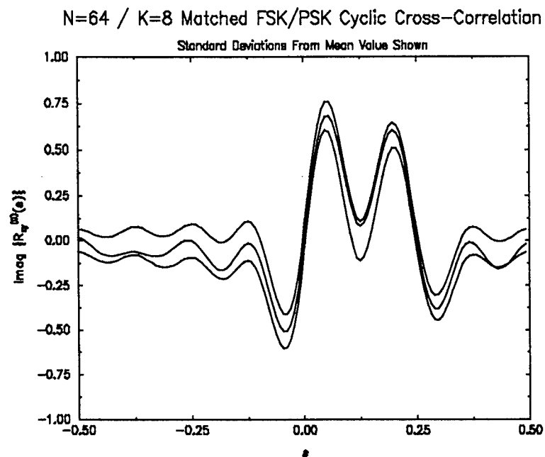
Figure 6.3.b. Imaginary Component of the Realized Matched FSK/PSK Cross-Ambiguity Function and Standard Deviations for N=64 and K=8.
