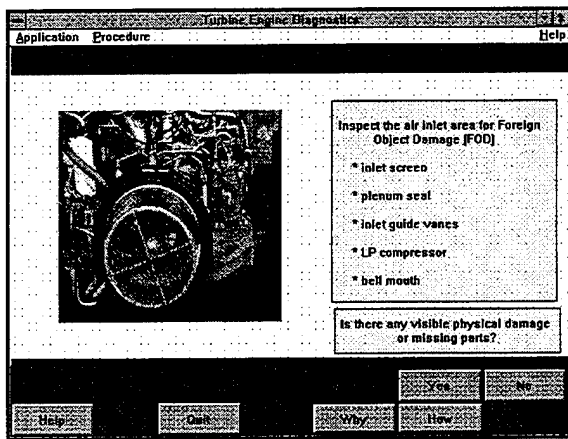
Figure 5: Preliminary Analysis Screen
