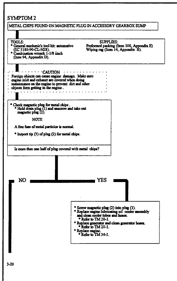
Figure 3: Sample page from TM
