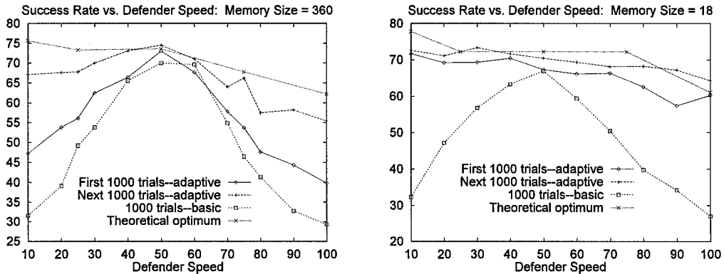
Figure 3: For all trials shown in these graphs, the agent began with a memory trained for a defender moving at constant speed 50. Adaptive memory outperforms basic memory for memories of size both 360 (left) and 18 (right). Since the basic memory does not change over time, the next 1000 trials produced the same results as the first 1000, and therefore are not plotted.
