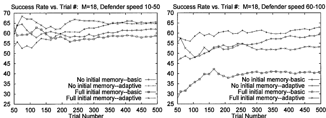
Figure 4: A comparison of the effectiveness of starting with an empty memory versus starting with a memory trained for a constant defender speed (50) different from the defender speed during testing. The performances of both adaptive and basic memories are plotted. Success rate is measured as goal percentage thus far.
