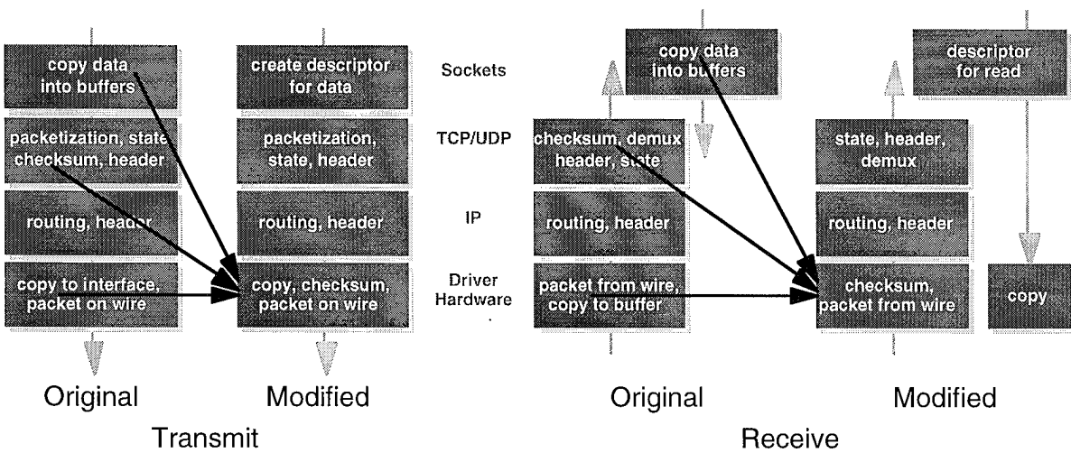
Figure 4: Software architecture
