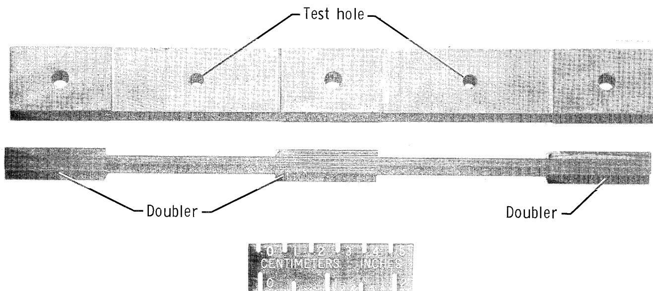
(b) Open-hole specimen.
