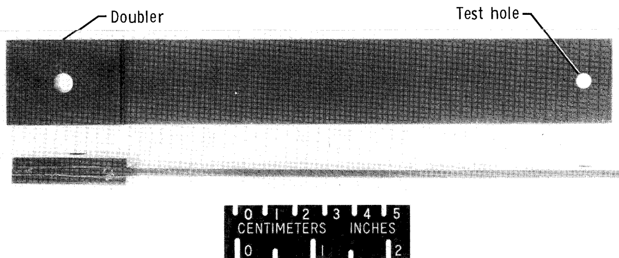
(b) Specimen for tests at low and elevated temperatures.
