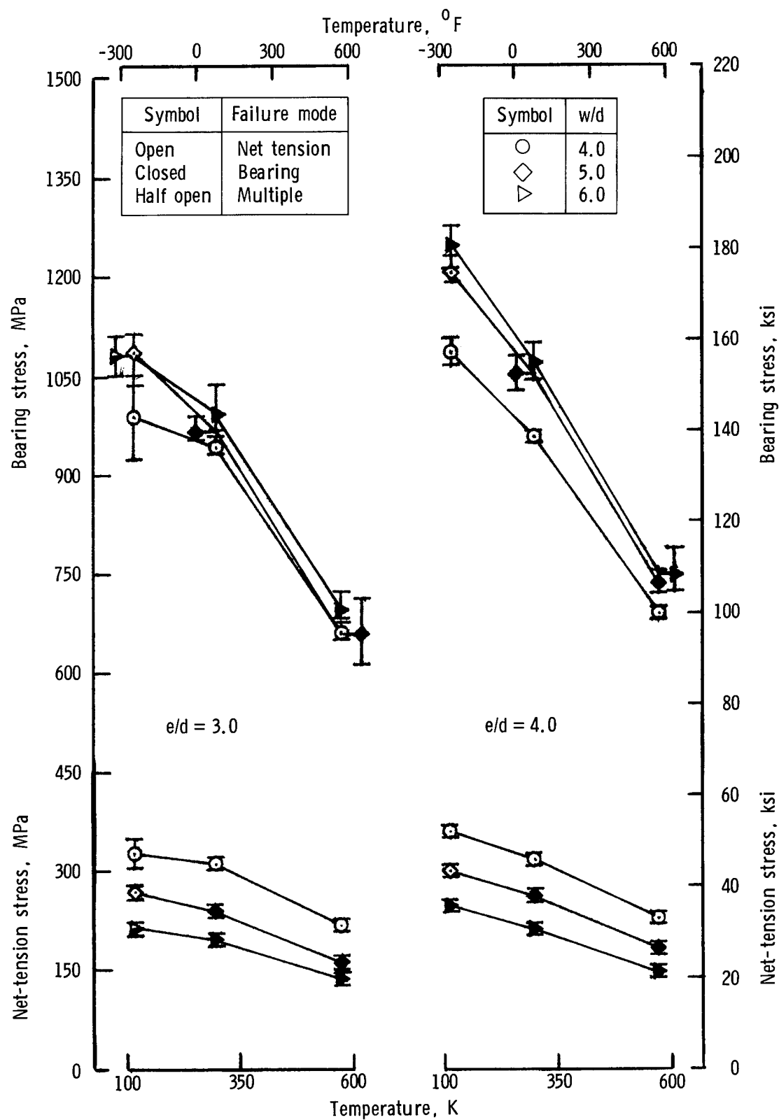
Figure 8.- Effect of joint geometry and temperature on net-tension and bearing stresses for Celion 6000/LARC-160 specimens.
