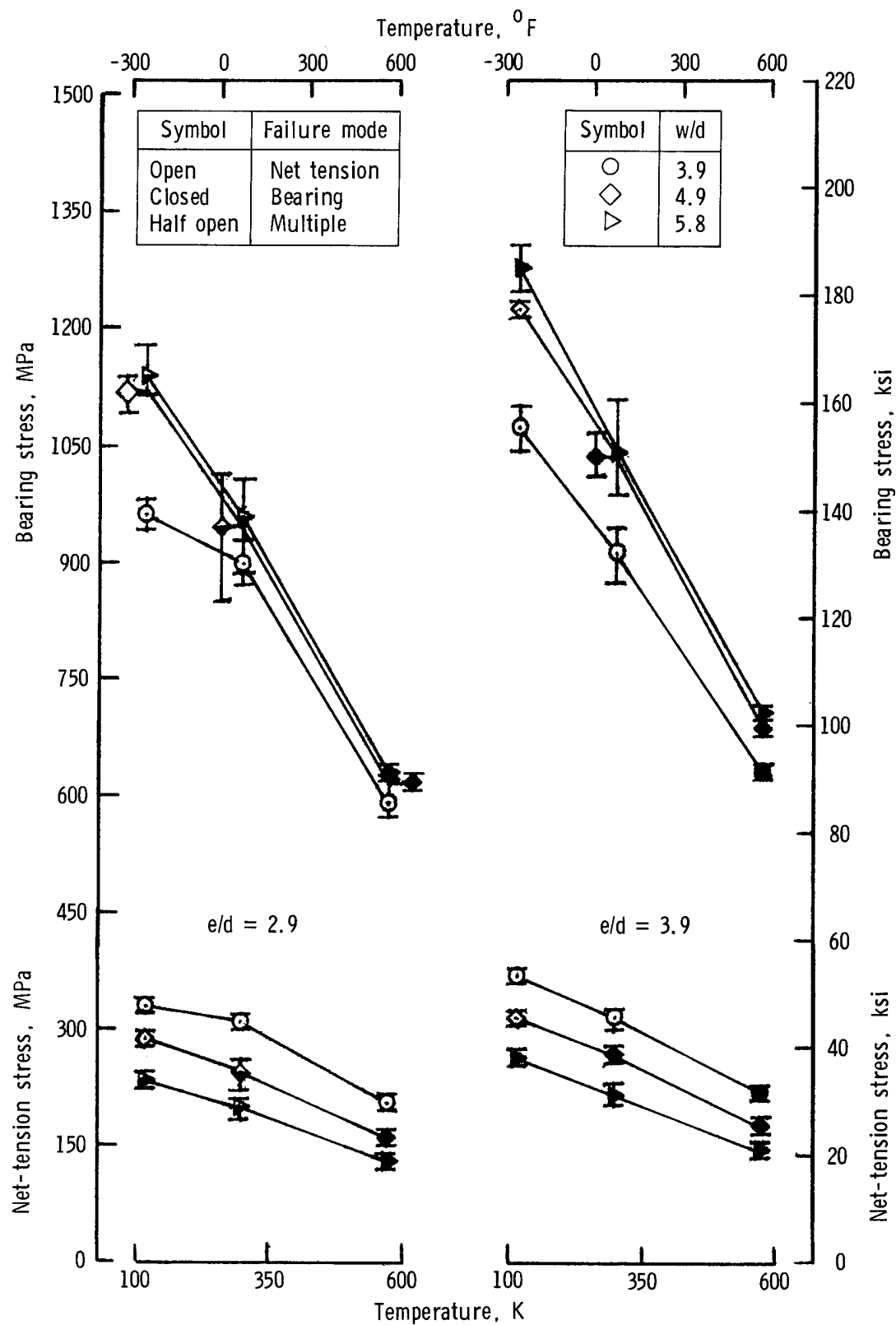
Figure 6.- Effect of joint geometry and temperature on net-tension and bearing stresses in-house for Celion 6000/PMR-15 specimens.
