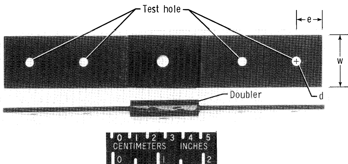
(a) Specimen for room-temperature tests.
