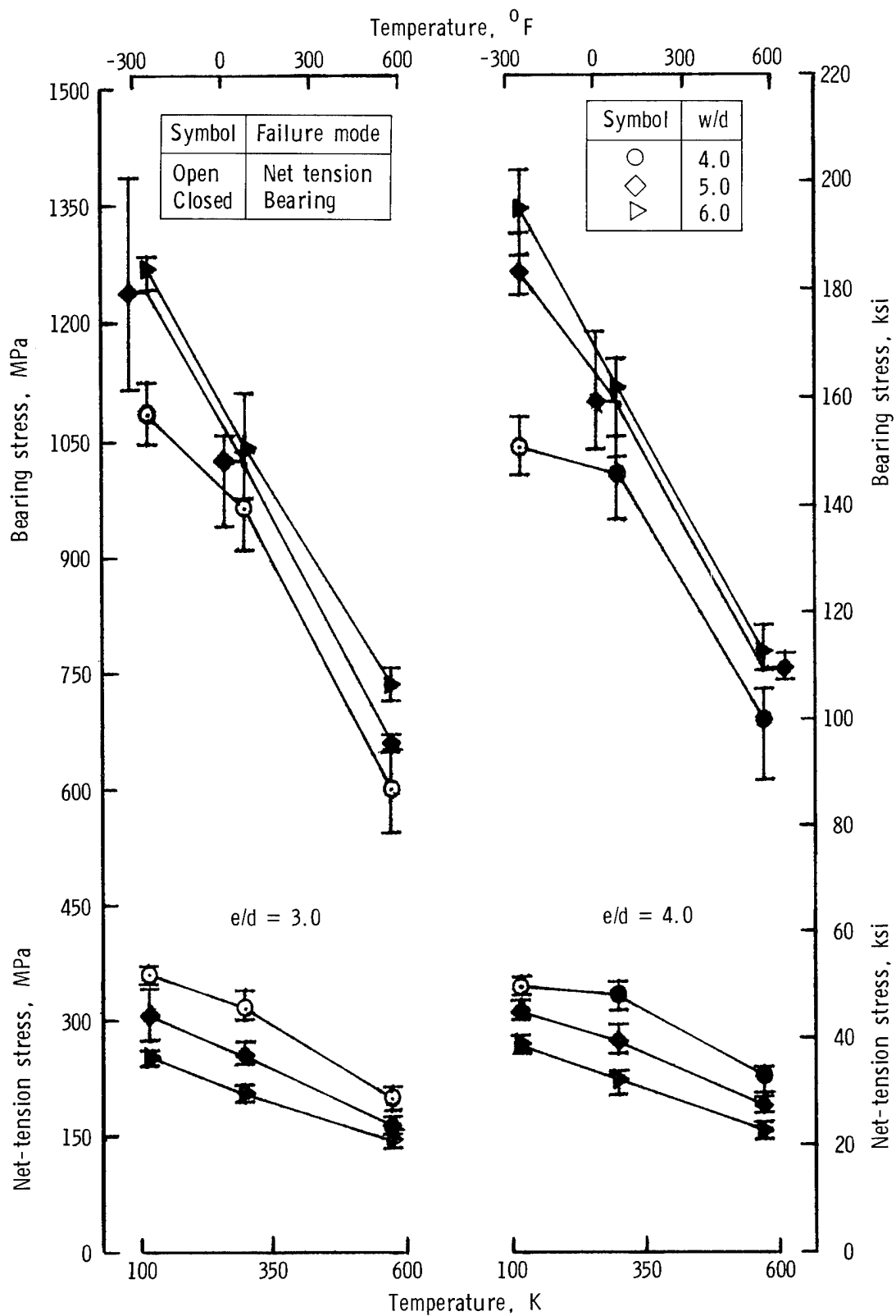
Figure 7.- Effect of joint geometry and temperature on net-tension and bearing stresses for contract Celion 6000/PMR-15 specimens.
