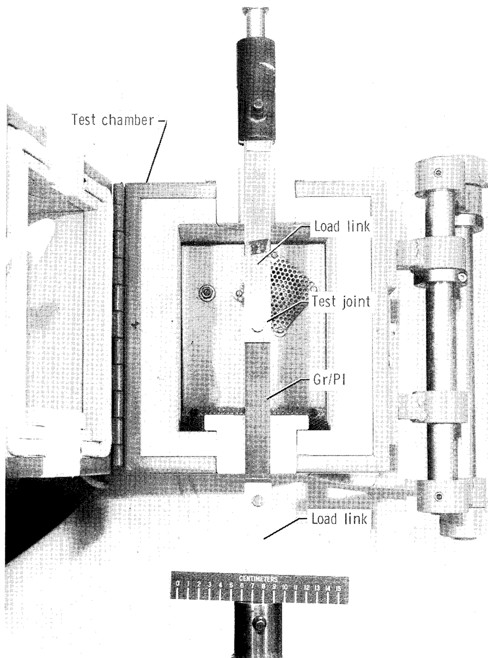
Figure 3.- Loading and heating apparatus for bolted-joint tests.
