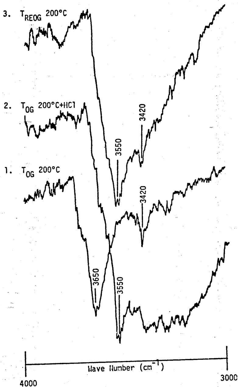
Figure 55. Infrared spectra ( 3000\text{--}4000\text{ cm}^{-1} ) of A2 Outgassed at 200^{\circ}\text{C} Before and After Hydrogen Chloride Adsorption
