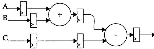
Figure 2: Data Flow Graph reduced to Synchronous Data Flow
