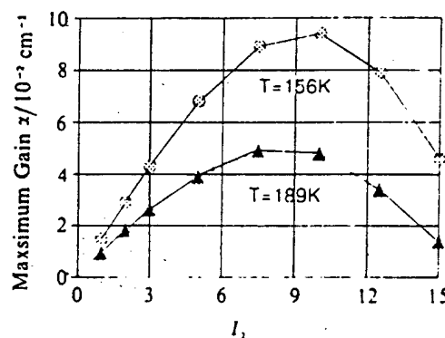
Fig. 3 Variation of gain coefficient vs percentage of I_2 under different cavity temperatures (partial pressure of O_2 in the cavity is 133Pa)
