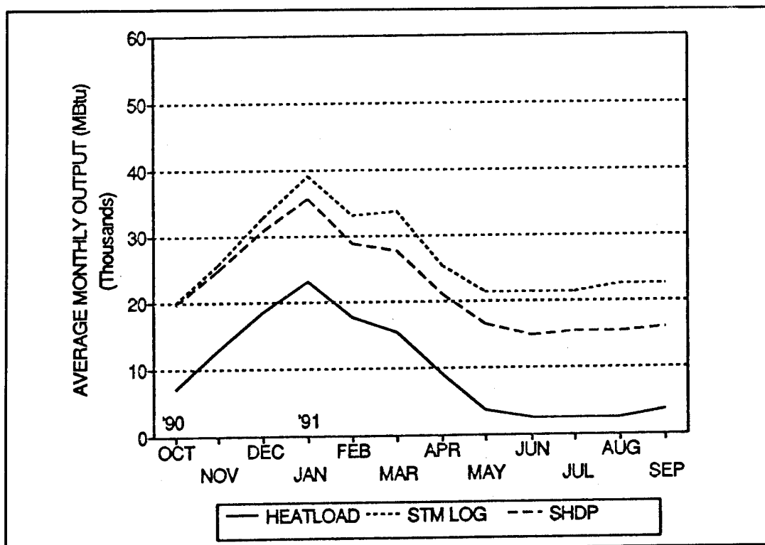
Figure 14. E3312 HEATLOAD with losses included.
