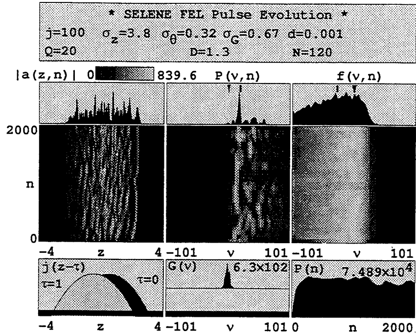
Figure 21. FEL output parameters after 2000 electron pulses for a two-section optical klystron oscillator.
