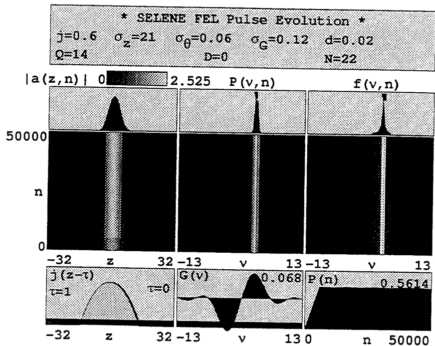
Figure 39. Optical pulse evolution during 50000 electron pulses for the one-piece undulator.
