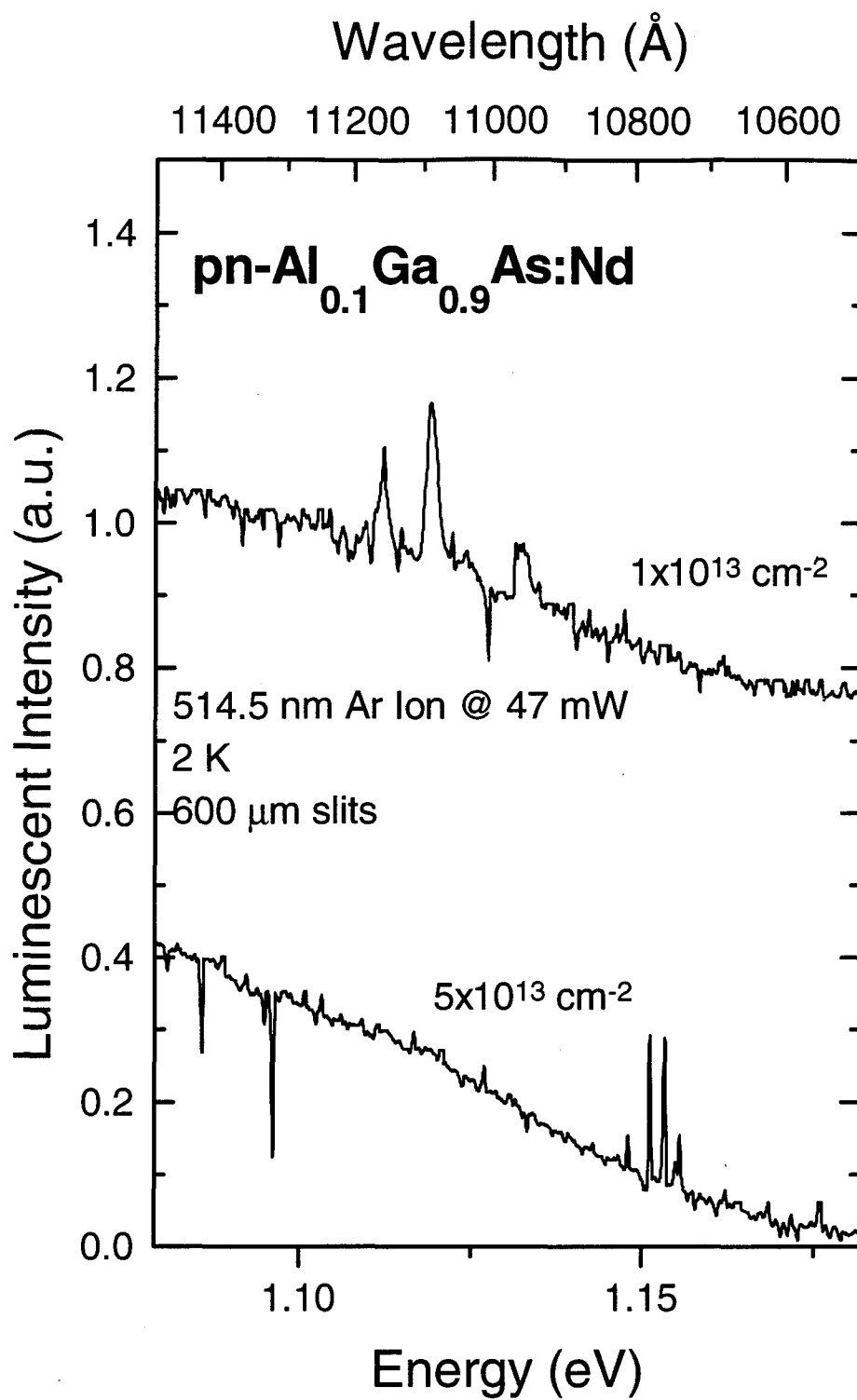
Figure 21. Photoluminescence measured from Nd implanted pn-type \text{Al}_{0.1}\text{Ga}_{0.9}\text{As} with doses of 1 \times 10^{13} \text{ cm}^{-2} and 5 \times 10^{13} \text{ cm}^{-2} .
