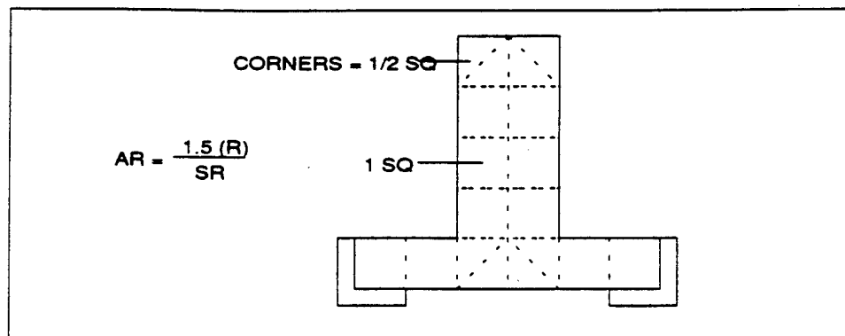
Figure 6.3.I Tophat Guidelines
