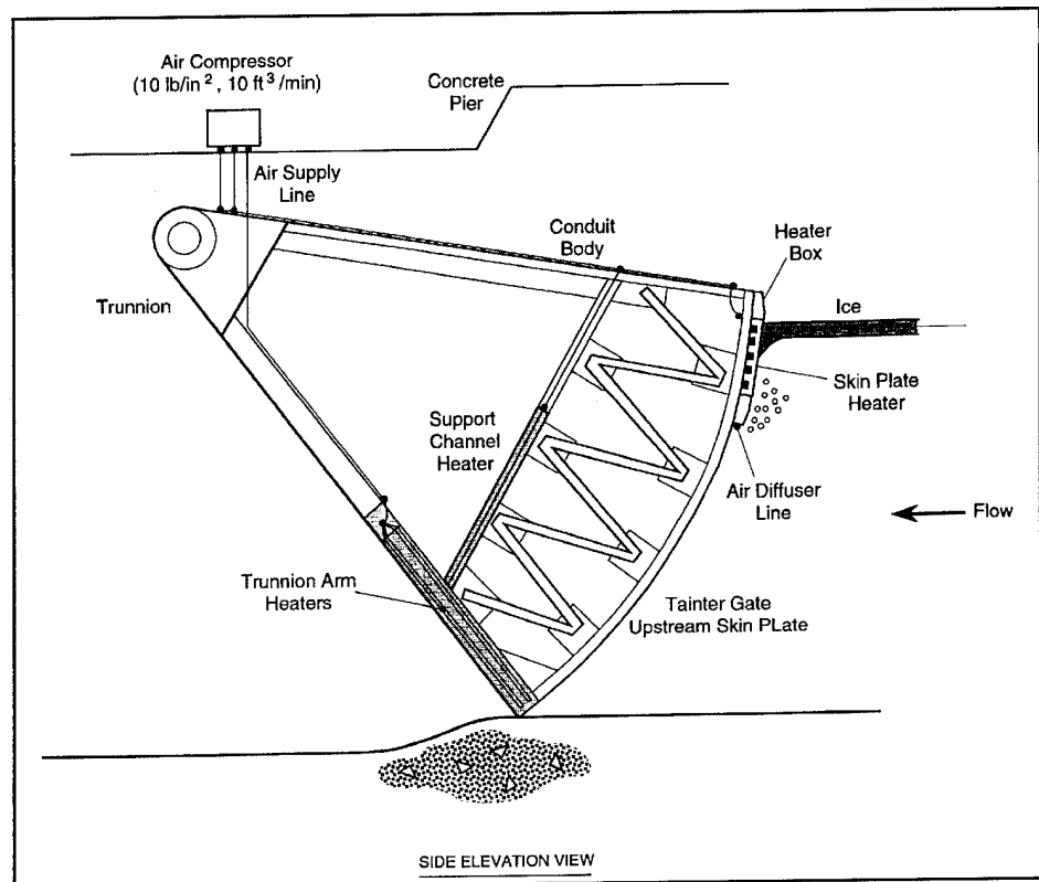
Figure 2. Tainter gate showing various heaters
