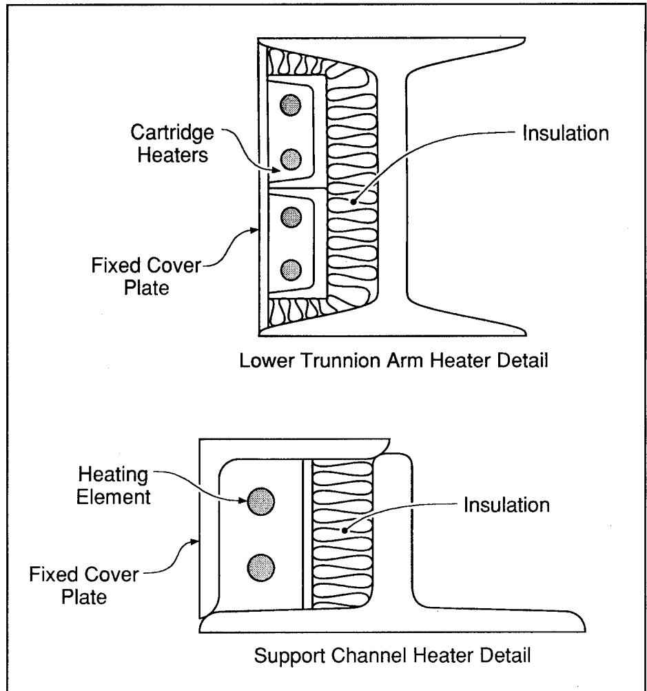
Figure 4. Cross section of lower trunnion arm and support channel heaters
