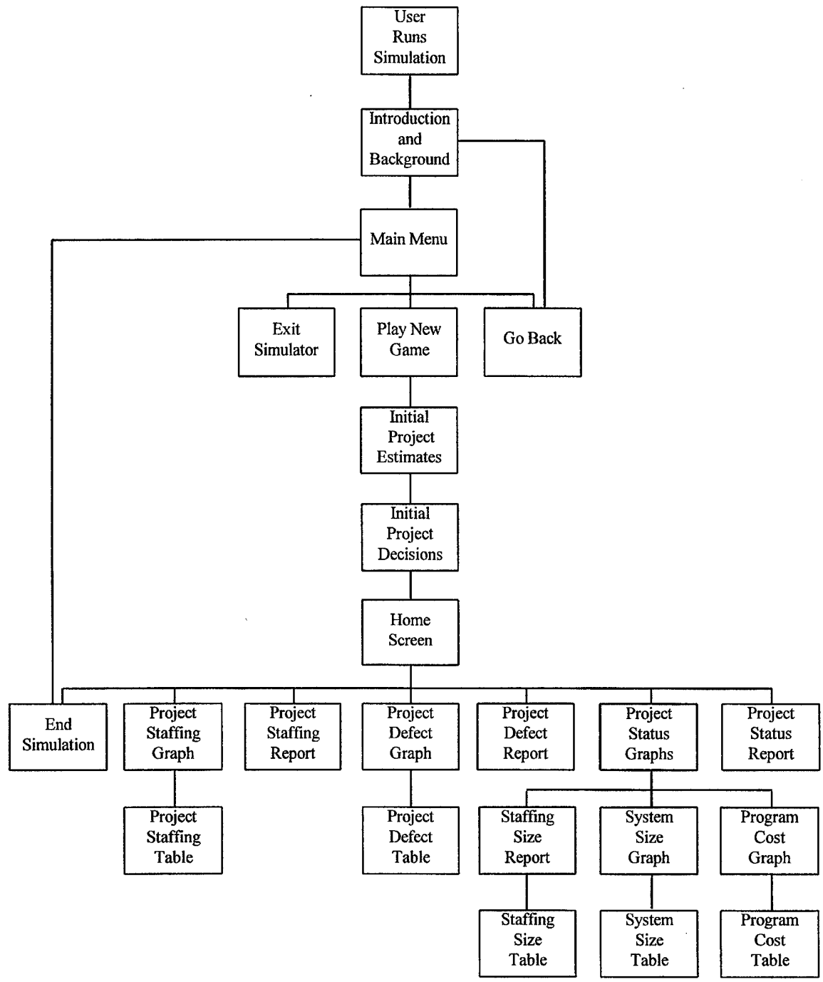
Figure 4. Simulation Model Menu Structure
