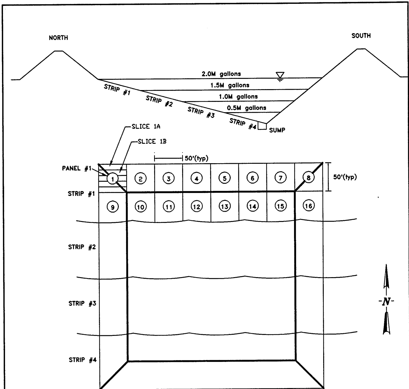
STRIP/PANEL LAYOUT
