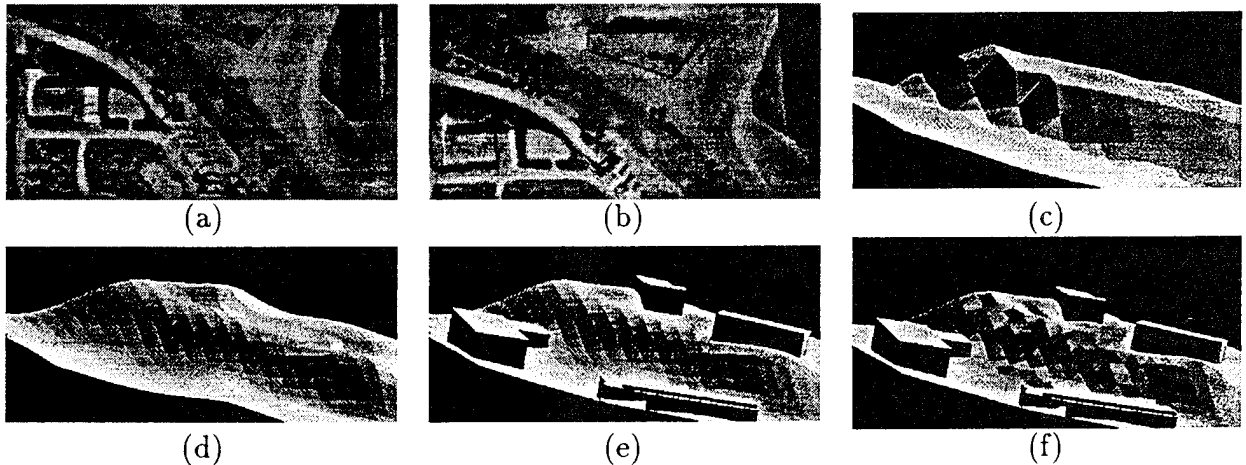
Figure 7: (a) (b) Two of a series of images of a semi-urban site. The images were taken with different light source directions. (c) A rough estimate of the ground-level surface (d) Surface after optimization using stereo alone. (e) Surface after optimization using both stereo and hand-entered buildings to mask occluded areas. (f) Surface after optimization using both stereo and shape from shading. In this case, the illuminations of the different images are different and there are very few bland, untextured areas. As a result, stereo alone performs better.
