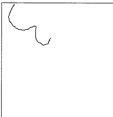
Extracted curve.
