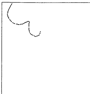
Random curve.
