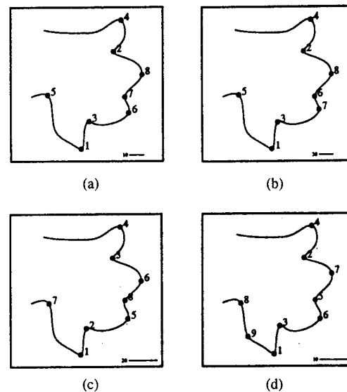
Fig. 6. Comparison of curve resolution versus change in operator size (stick length) on test curve 37f. Critpts are labeled with rank ordering of their scores. (The scaled curves are drawn to fit into a standard-size box.) (a) Scale 1; stick length 10. (b) Scale 2; stick length 20. (c) Scale 1; stick length 20. (d) Scale 0.5; stick length 10.
