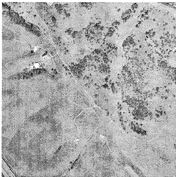
Grayscale image.
