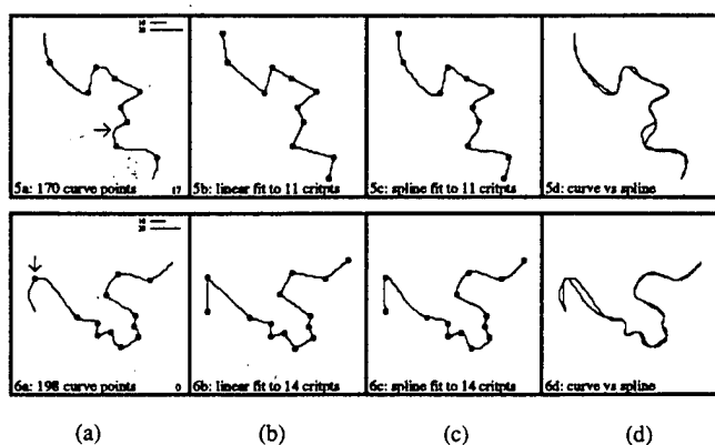
Fig. 10. Examples of curve reconstruction based on using straight line and spline interpolations of critpts. (a) Input curve showing SSS selected critpts. (b) Straight line interpolation of critpts. (c) Spline interpolation of critpts. (d) Comparison of original and reconstructed curves.
