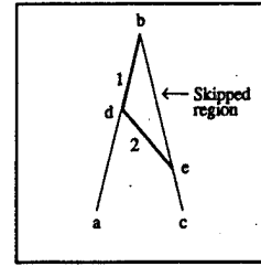
Fig. 16. Nonsymmetric scores for forward and backward movement along a curve produced by F/B-S employing a fixed Euclidean distance for stick size. Consider stick s , as shown in position 1. A slight movement clockwise will cause the stick to jump to position 2, skipping the indicated region. If the stick was scanning the curve in the reverse direction, a skipped region would occur on the opposite leg of the angle/curve.
