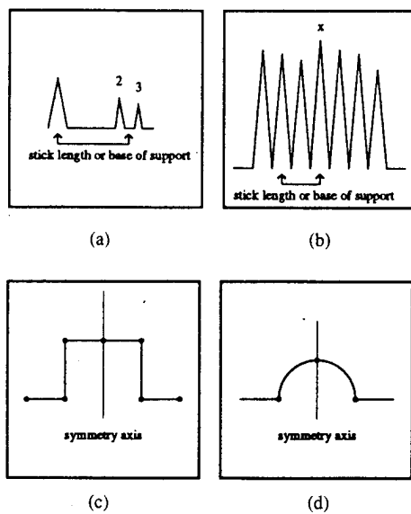
Fig. 7. Problem situations correctly handled by the SSS algorithm. The critpts at peaks 2 and 3 should be both accepted or both rejected in (a). In (b), the critpts at all peaks surrounding the peak at x are approximately equal in saliency; they should all be accepted or all rejected. The pattern of accepted critpts should be symmetric in (c) and (d).
