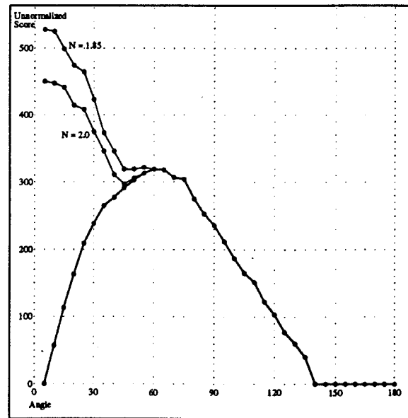
Fig. 13. Augmented and standard (unnormalized) SSS scores for angles at increments of 5^\circ (stick length 20). The bold curve shows the standard SSS scores. The thin curves show the augmented scores for two different values of N at which we alter the way distance is measured from a curve point to the stick (i.e., when the number of curve points between the end points of the stick is greater than N times the stick length, the distance from the curve point to the midpoint of the stick is used as the deviation of the curve from the stick).
