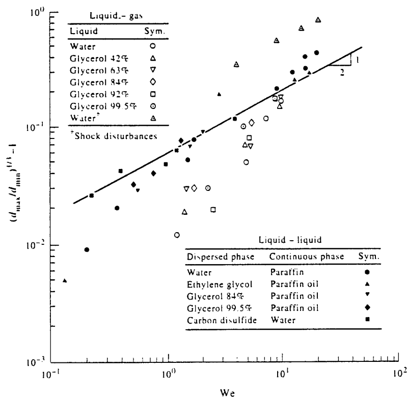
Figure 3. Drop deformation as a function of Weber number.
