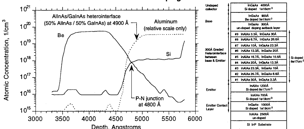
Figure 15: Doping profile of an SCHBT wafer with an improved base doping profile. Base doping was reduced to 5 \cdot 10^{19}/cm^3 , growth temperature reduced, and the base doping set back 300 Å. The base-emitter p-n junction is now correctly located.
