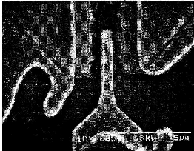
Figure 29: SEM of an antenna-coupled 0.1 μm • 0.5 μm THz detector diode.
