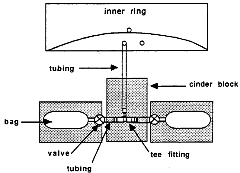
Figure 4. Arrangement Of Two Bags Connected To Inner Ring
