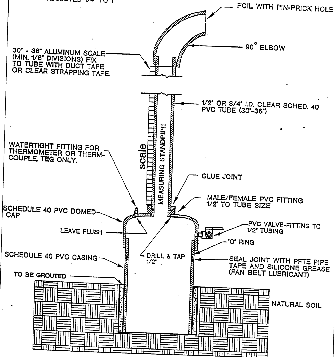
TYPICAL PERMEAMETER
