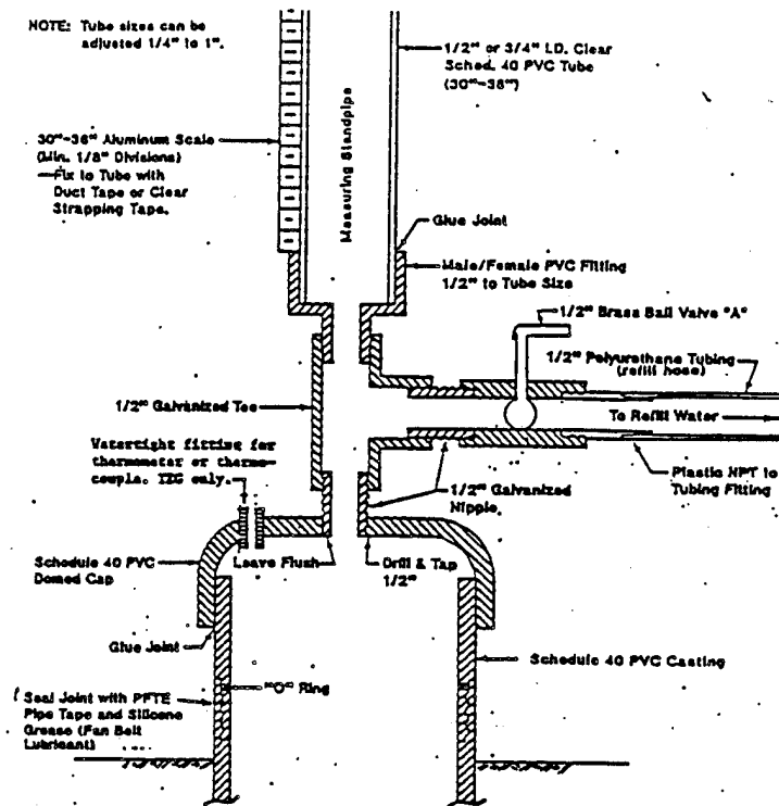
FIGURE 2 TYPICAL PERMEAMETER
