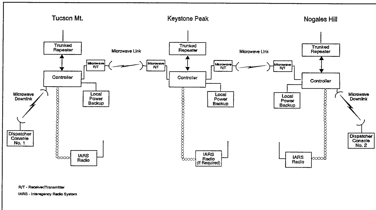
Figure 4. Corridor interagency communications system configuration.
