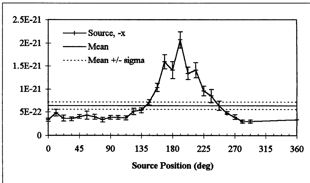
Figure I.2 Exposure (R/s/particle) at each source point for negative x source axis detector for CT in WPMC with 1/8" lead shielding, head scan.
