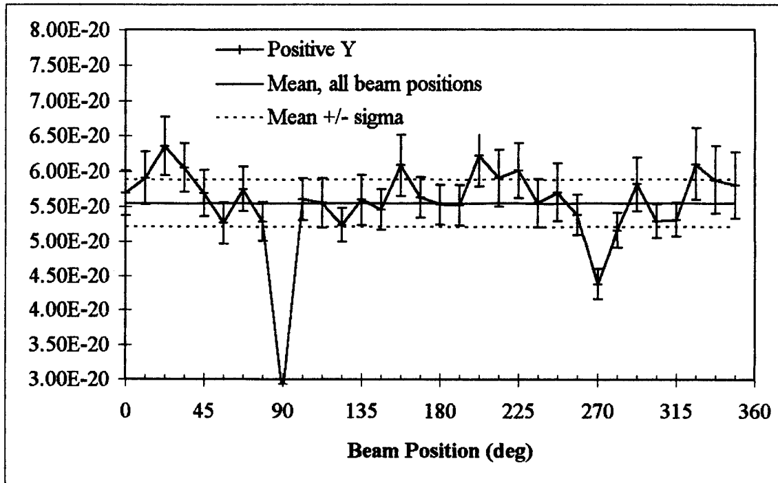
Figure D.5 Positive y exposure(R/s/particle) for CT in X-ray room. No direct beam position.
