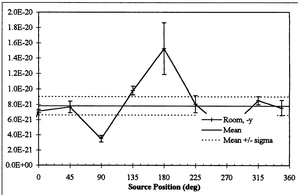
Figure K.8 Exposure (R/s/particle) at each source point for negative y room axis detector with with CT in GE minimum recommended room, 1/16" lead, head scan.
