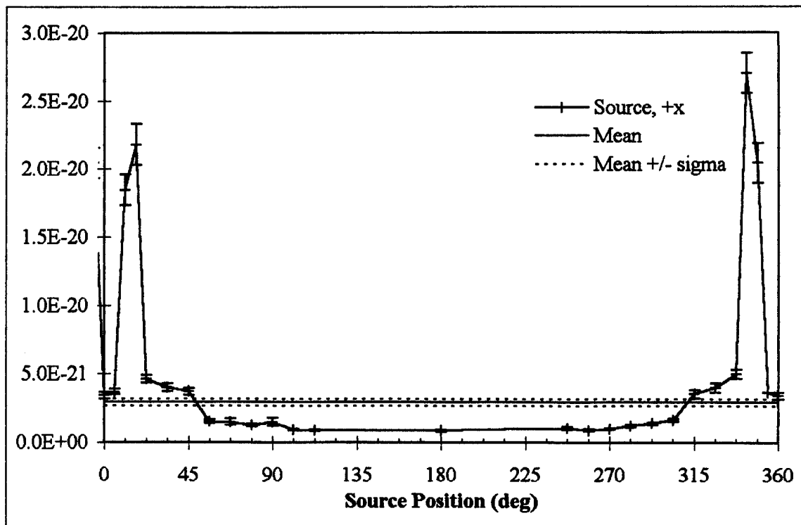
Figure H.1 Exposure (R/s/particle) at each source point for positive x source axis detector with CT in WPMC, 1/16" lead, abdomen scan.
