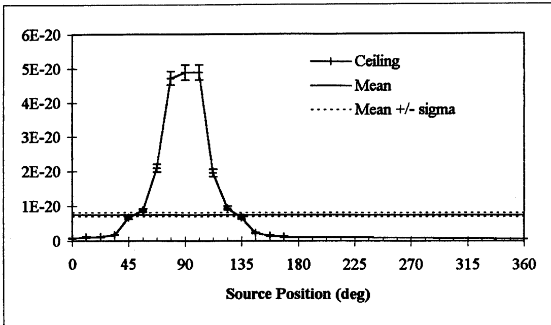
Figure I.9 Exposure (R/s/particle) at each source point for ceiling detector for CT in WPMC with 1/8" lead shielding, head scan.
