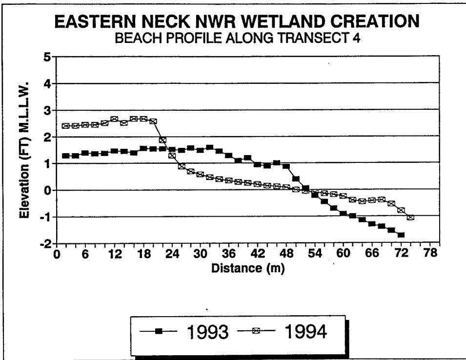
Figure A4. Beach profile along Transect 4
