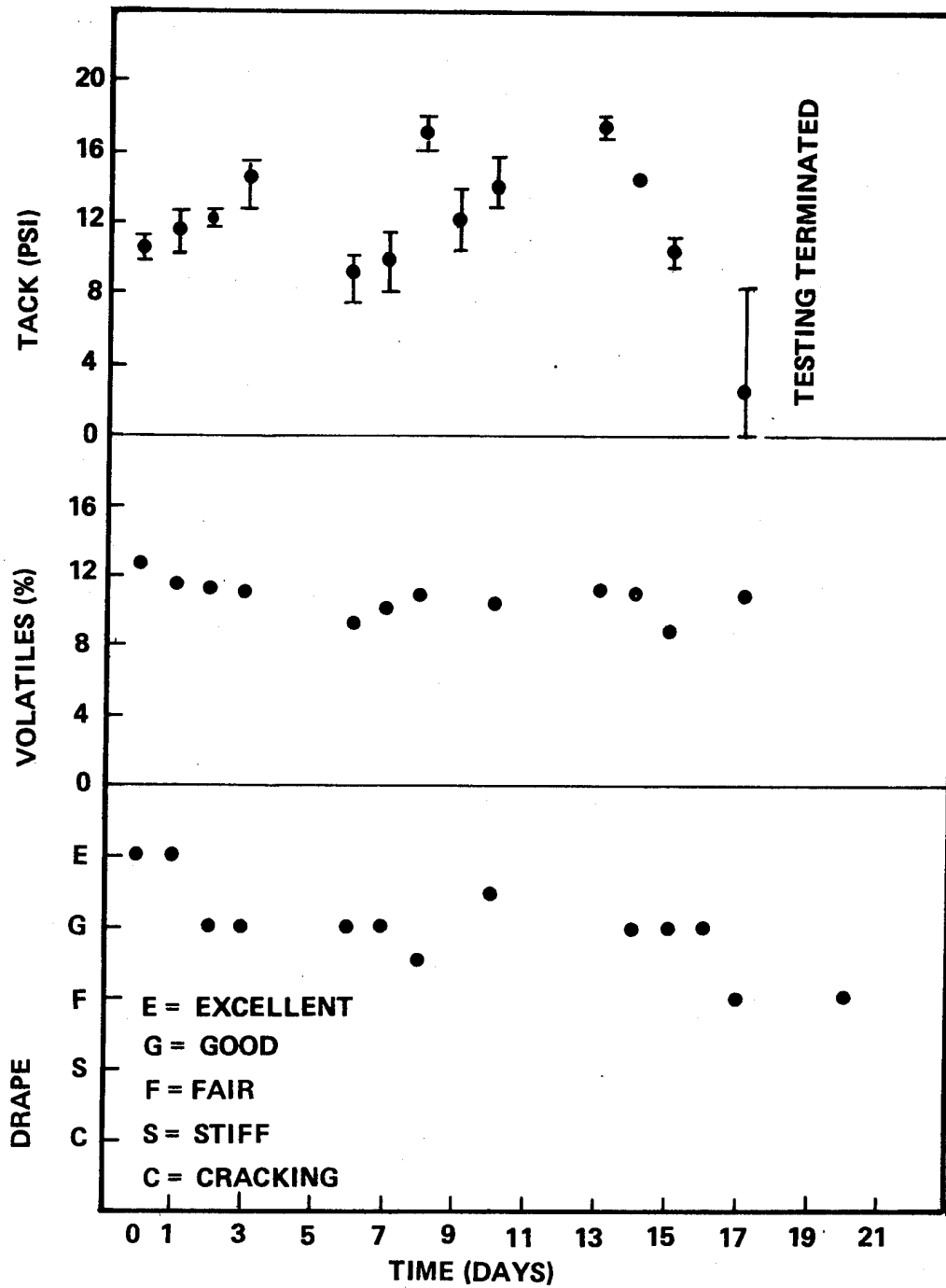
Figure 2. Change in Prepreg Characteristics with Time Formulation 2: Diglyme (20 w/o)
