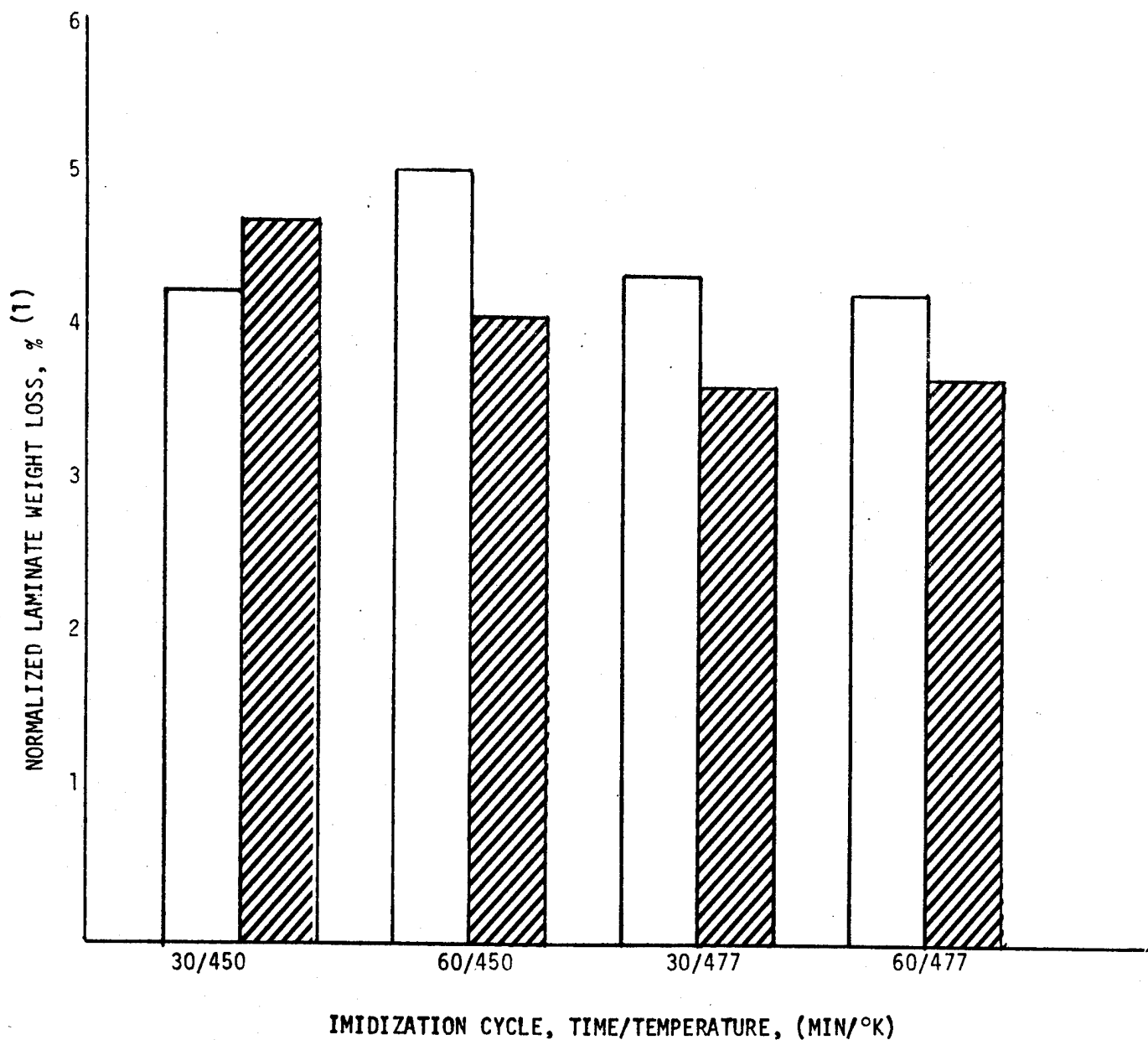
FIGURE 14. LAMINATE WEIGHT LOSS AFTER 600 HOURS EXPOSURE TO 589°K (600°F)
