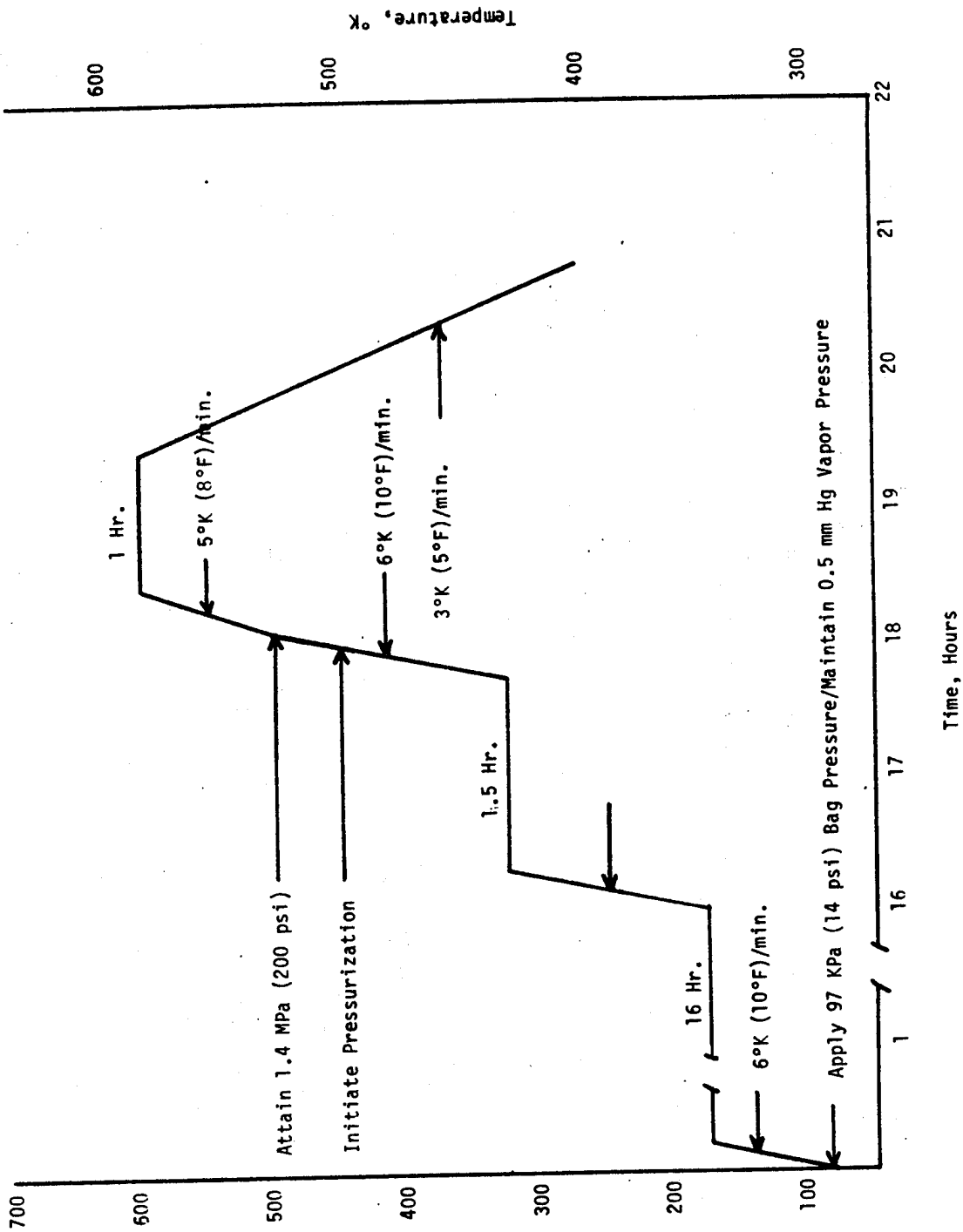
Figure 24 Autoclave Cure Cycle A-4.
