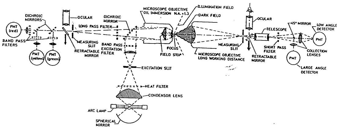
Fig. 1 Optical configuration of arc lamp-based flow cytometer with epi-illumination.
