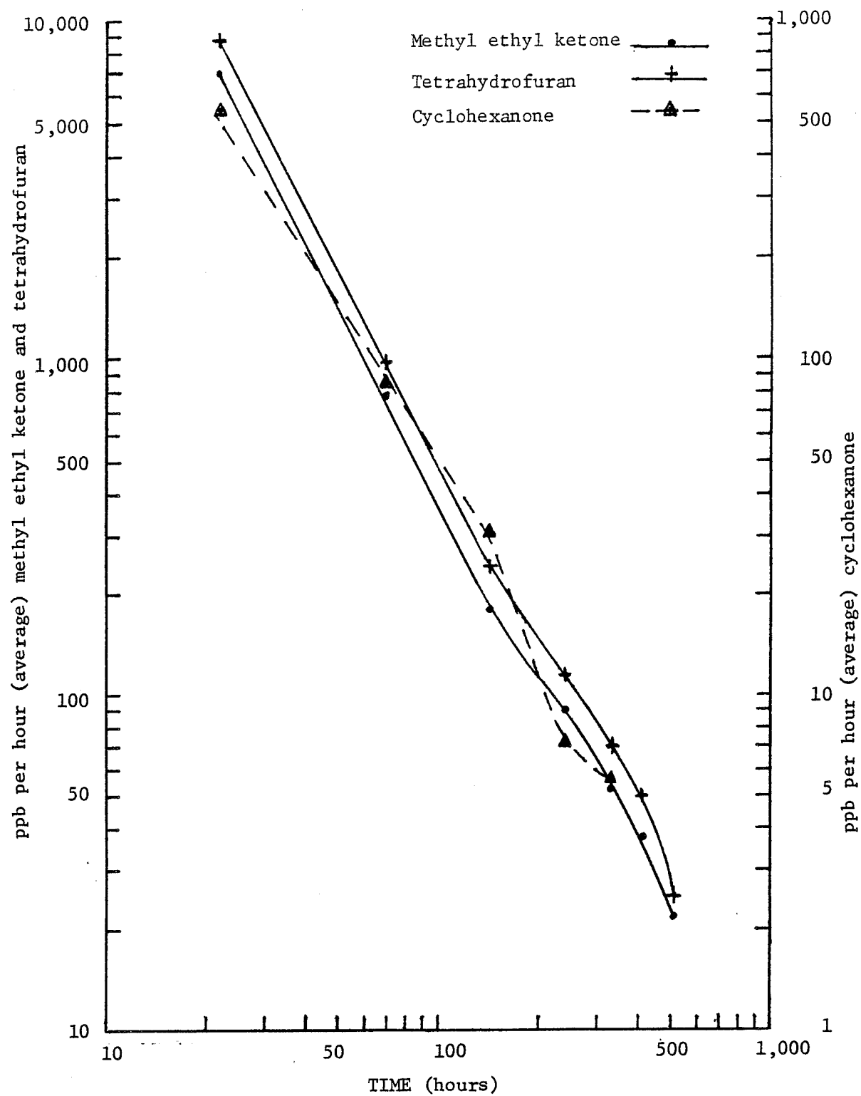
Figure 28. Standardized cement solvent concentrations observed in CPVC sample #14C pipe loop water samples.
