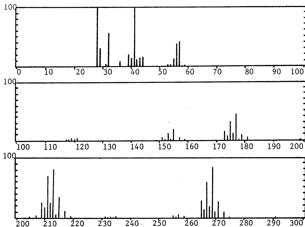
Figure A-8. Mass spectrum of tributyltin chloride.
