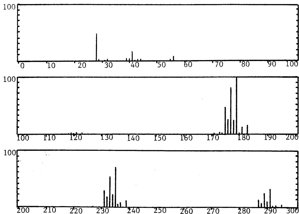
Figure A-15. Mass spectrum of tetrabutyl tin.
