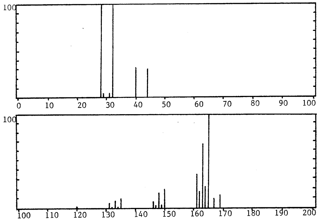
Figure A-14. Mass spectrum of tetramethyl tin.
