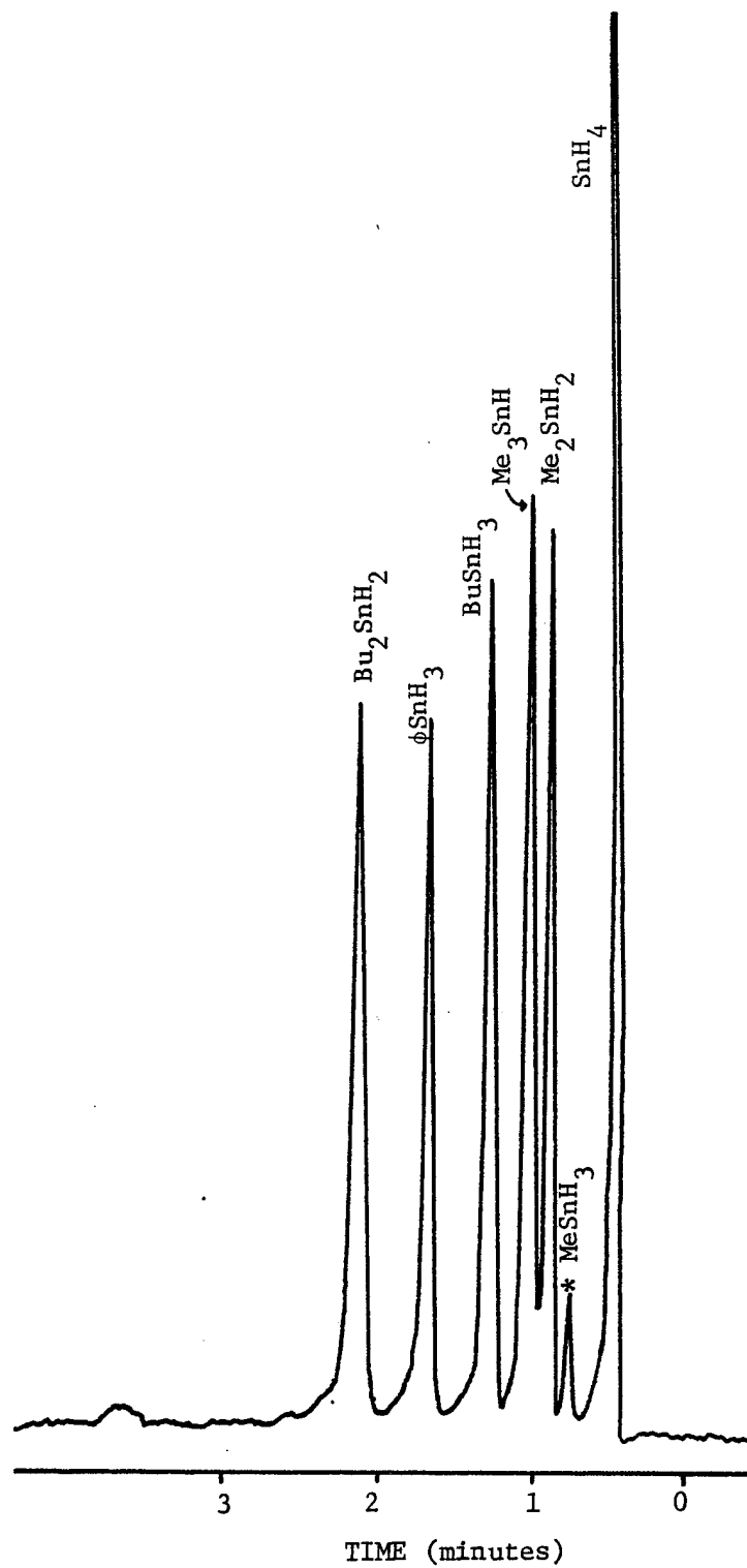
Figure 2. Separation of hydrides on glass beads. (* Me is methyl, Bu is n-butyl, \phi is phenyl)
