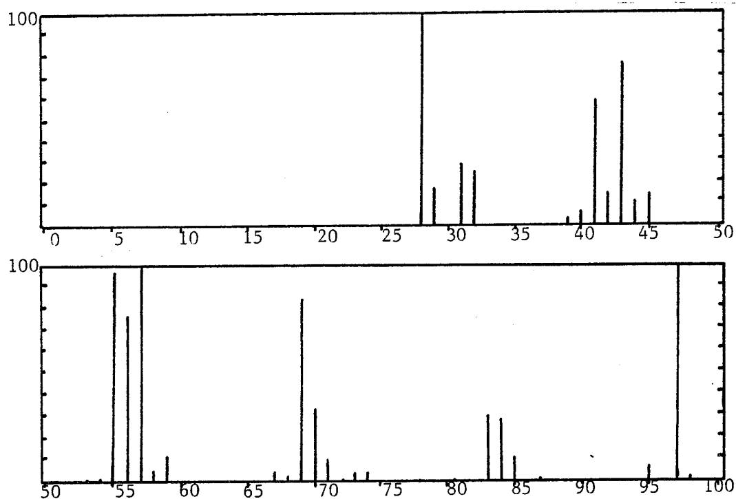
Figure 10. Mass spectrum of the 3.0-minute peak in the chromatogram of CPVC #6.
