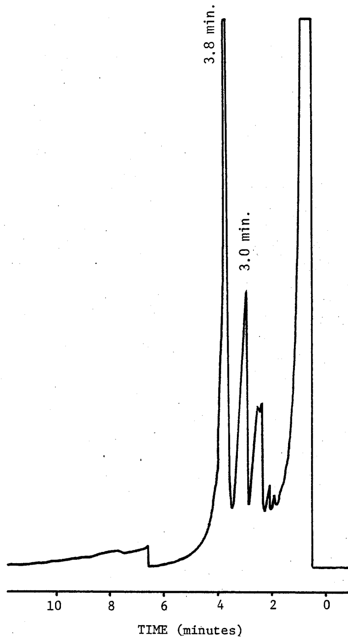
Figure 9. Chromatogram of compounds leached from CPVC #6, on 3% (w/w) OV-17, 90°C isothermal temperature.
