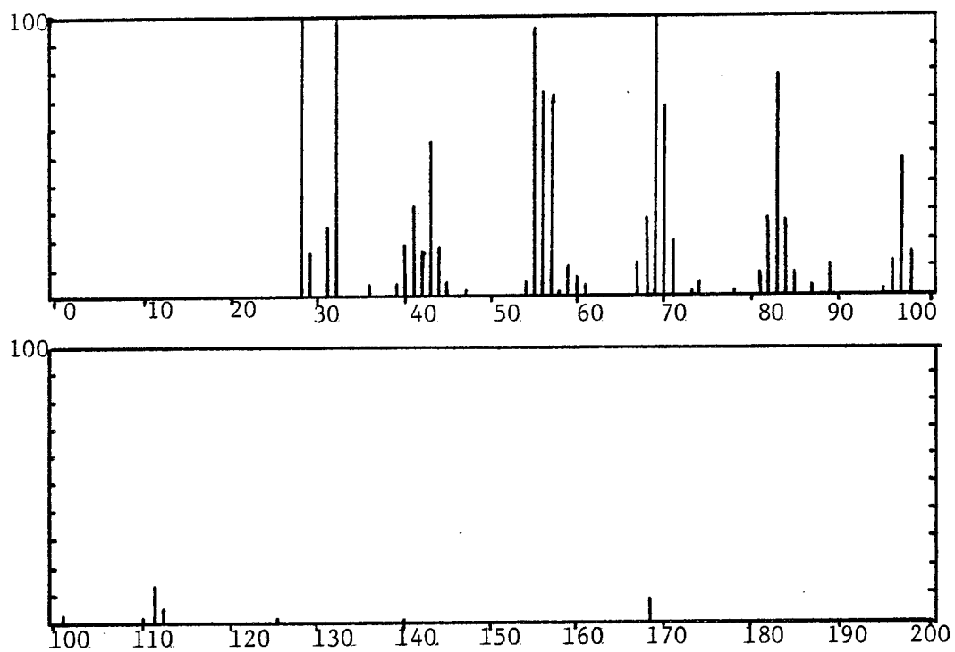
Figure A-3. Mass spectrum of dibutyltin-bis-laurylmercaptide extraction degradation product.
