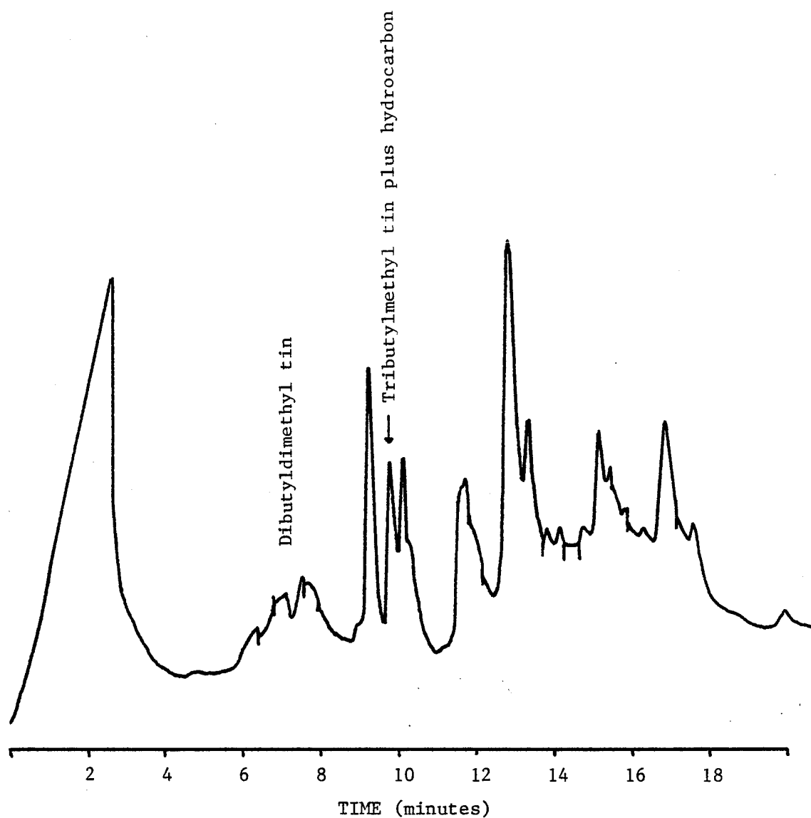
Figure 16. Total ion current chromatogram of the Grignard butylation products of sample #14A;
