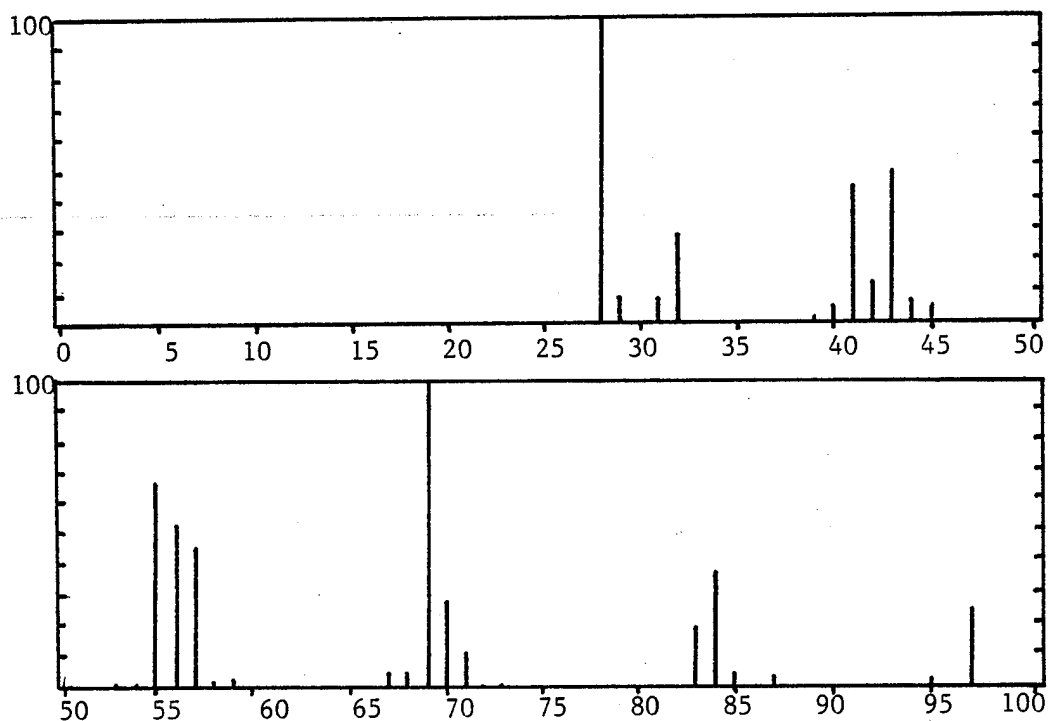
Figure 15. Mass spectrum of the 4.1-minute peak in Figure 13.
