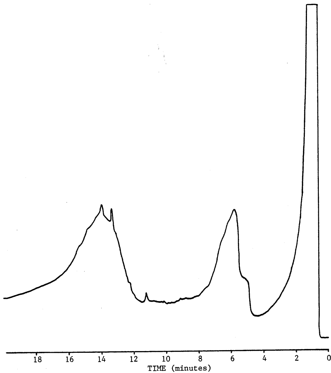
Figure A-4. Gas chromatogram of dibutyltin-bis-isooctylthioglycolate acetone stock solution.
