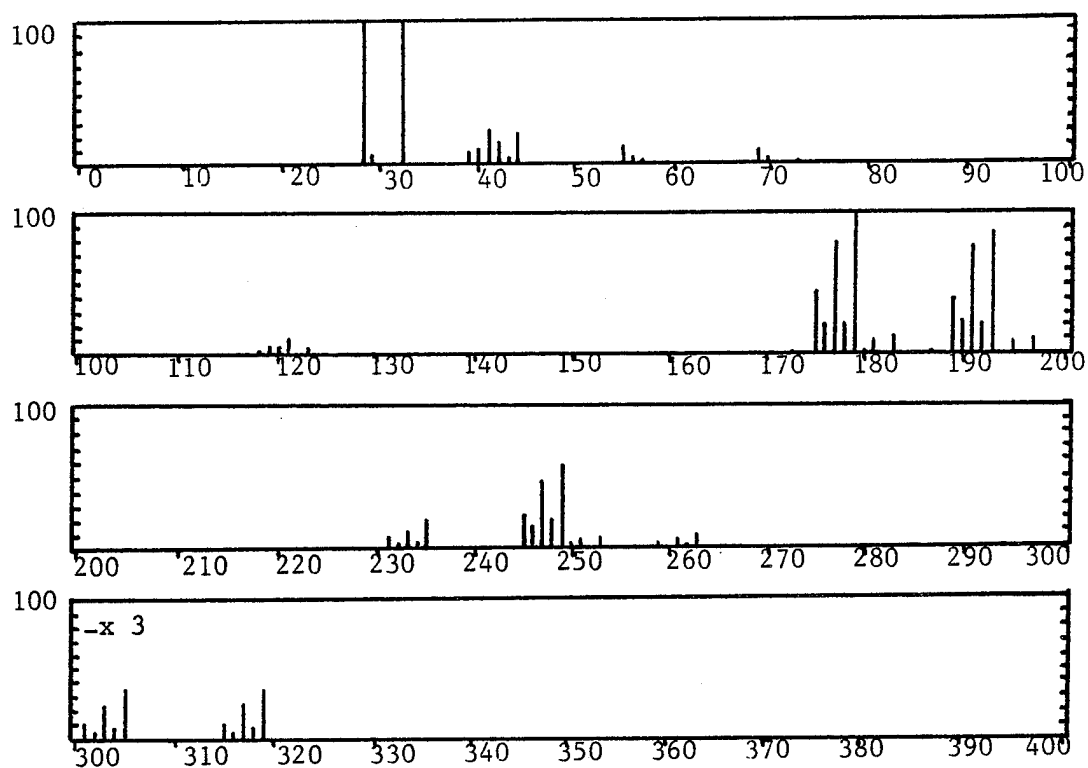
Figure 6. Mass spectrum of dibutyldipentyl tin.
