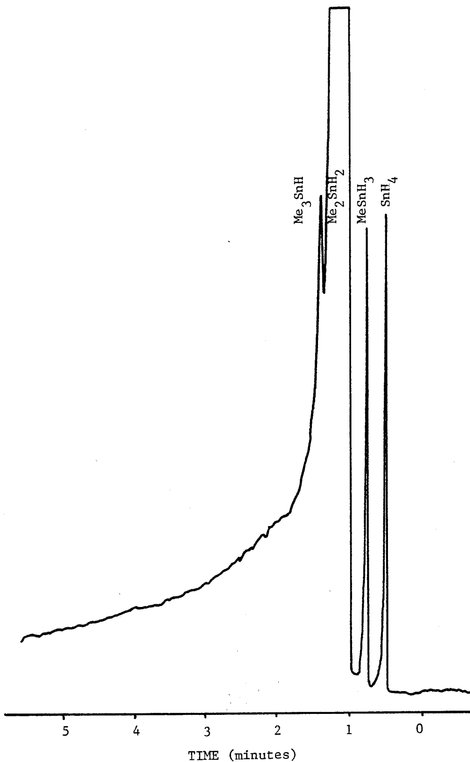
Figure 21. Analysis of extractant water digest of PVC sample #14A by hydride-generation atomic absorption (10 mL sample in 100 mL). Me is methyl.
