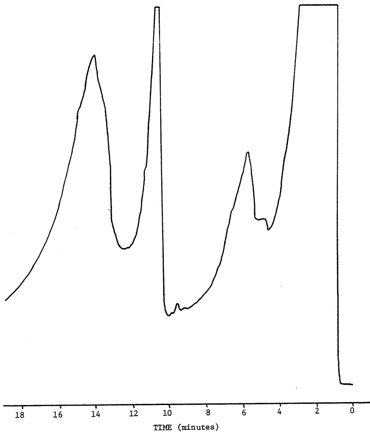
Figure A-5. Gas chromatogram of a concentrated hydrobromic acid/benzene extract of a dibutyltin-bis-isooctylthioglycolate water solution.
