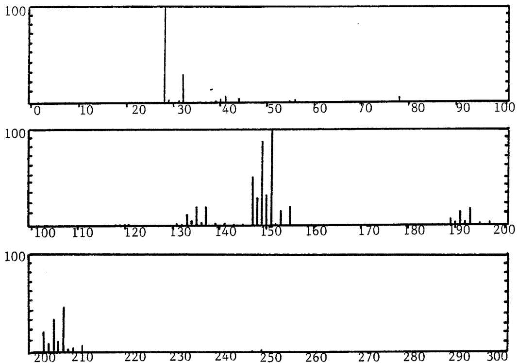
Figure A-12. Mass spectrum of dibutyldimethyl tin.
