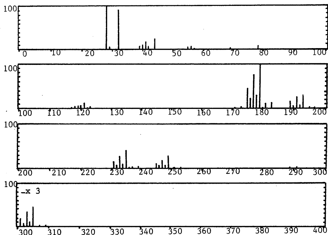
Figure 5. Mass spectrum of tributylpentyl tin.
