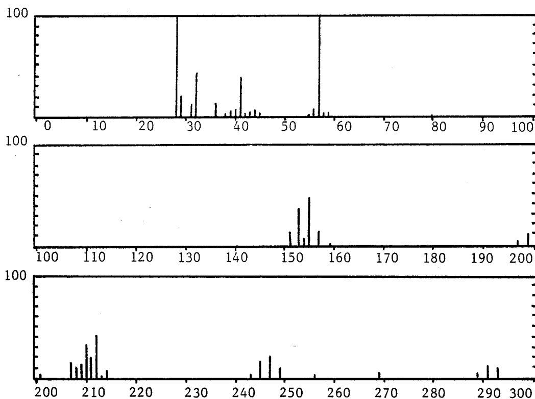
Figure A-7. Mass spectrum of dibutyltin dichloride.
