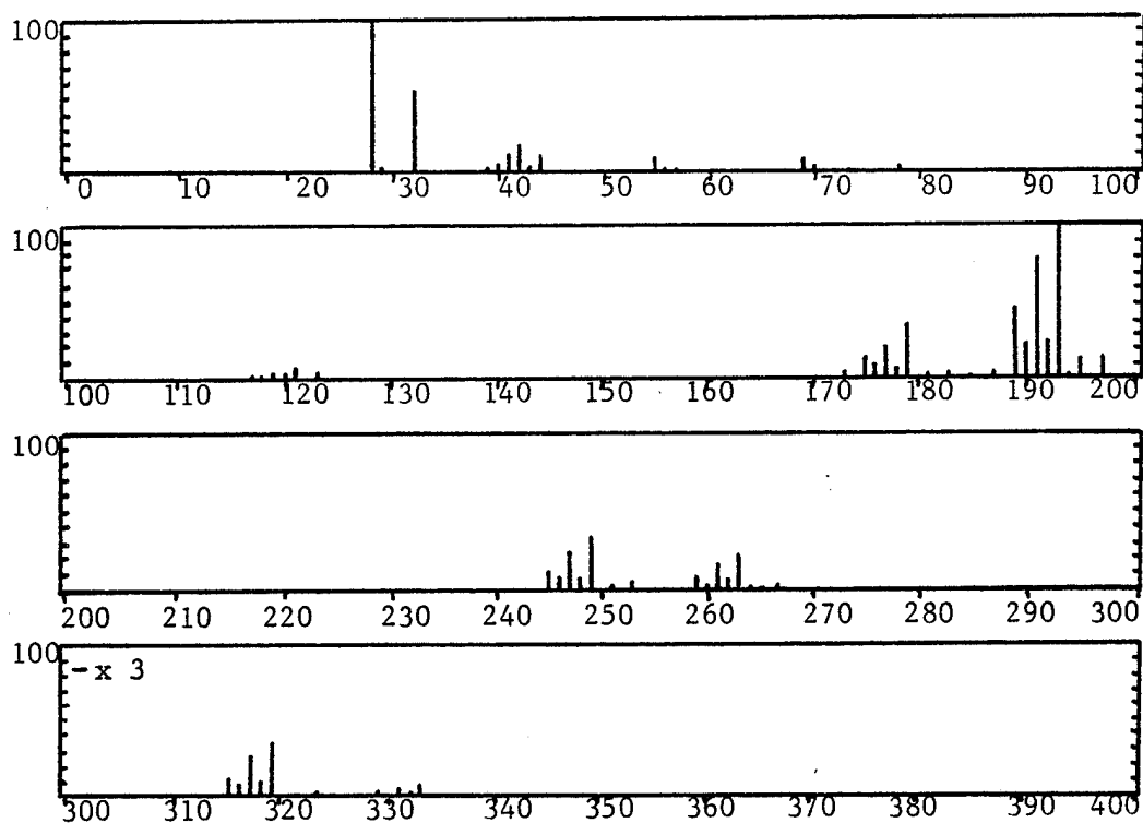
Figure 7. Mass spectrum of butyltripentyl tin.
