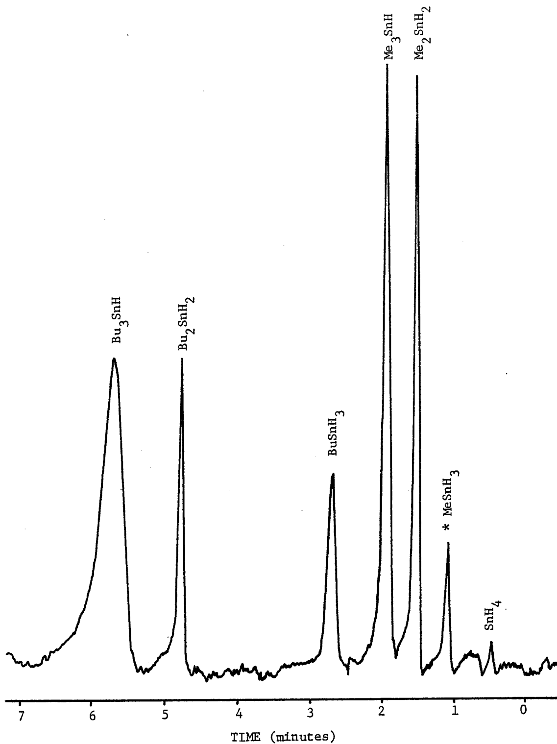
Figure 3. Separation of hydrides on OV-1. (* Me is methyl, Bu is n-butyl)
