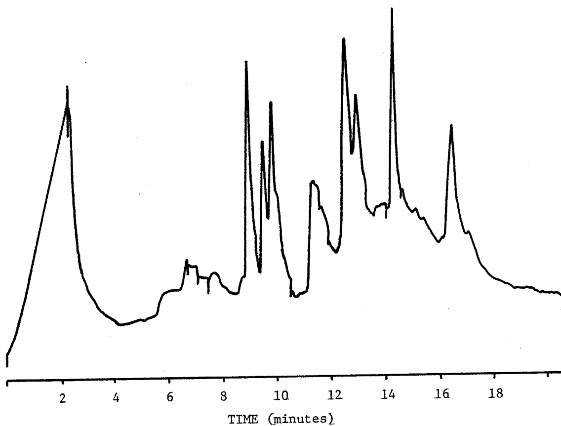
Figure 18. Total ion current chromatogram of Grignard butylation products of blank sample.
