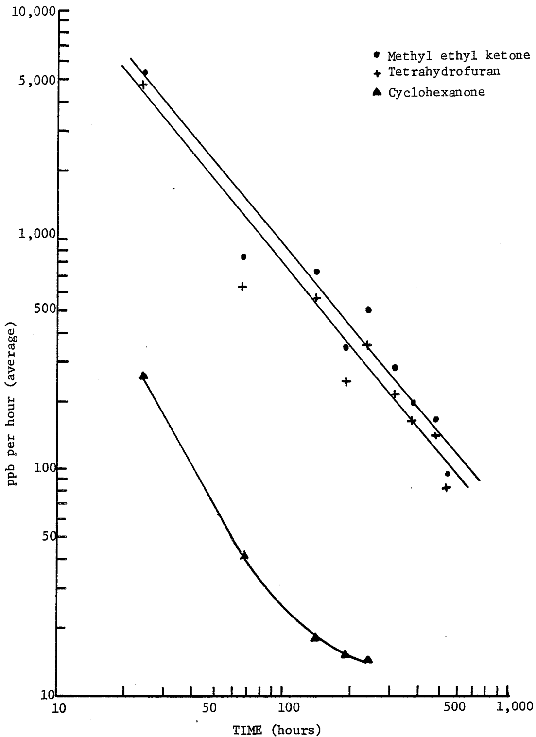
Figure 26. Standardized cement solvent concentrations observed in PVC sample #14A pipe loop water samples.
