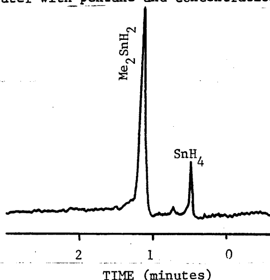
Figure 20. Analysis of extractant water digest of PVC sample #14A by hydride-generation atomic absorption (0.1 mL sample in 100 mL). Me is methyl.
