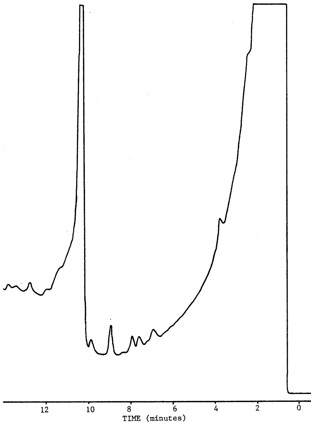
Figure A-2. Gas chromatogram of a concentrated hydrobromic acid/benzene extract of a dibutyltin-bis-laurylmercaptide water solution.
