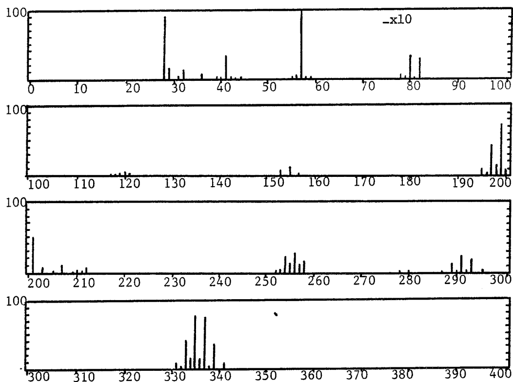
Figure A-1. Mass spectrum of dibutyltin bromide chloride and dibutyltin dibromide from hydrobromic acid/benzene extraction of a dibutyltin dichloride water standard.
