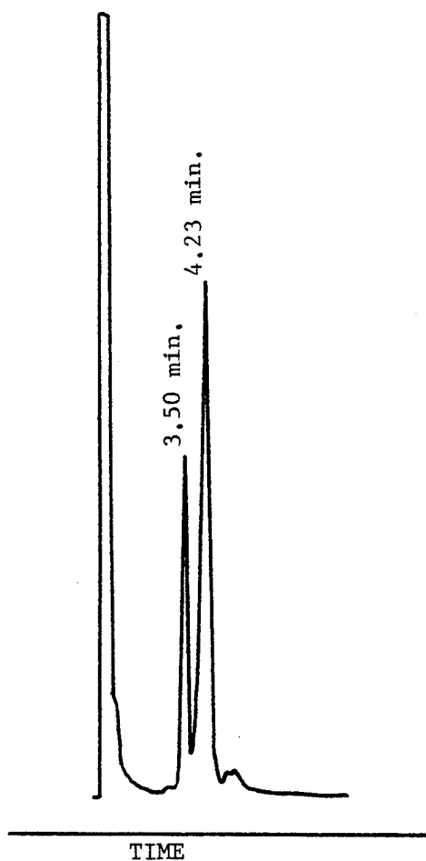
Figure 22. Gas chromatogram of isooctyl thioglycolate on 10% (w/w) OV-1, 160°C isothermal temperature (0.5 \mu L/mL in pentane).
