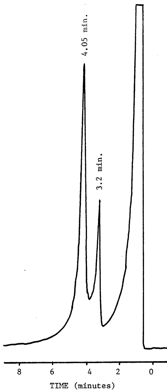
Figure 13. Chromatogram of dibutyltin-bis-isooctylthioglycolate ester saponification products, on 3% (w/w) OV-17, 90°C isothermal temperature.
