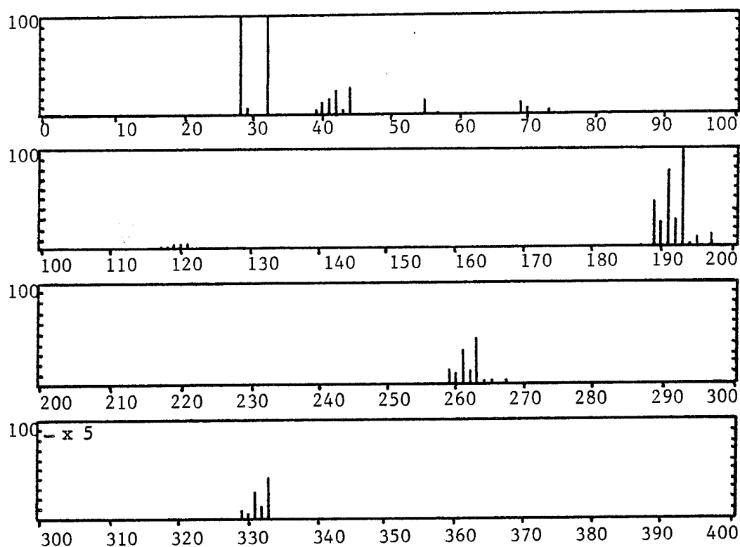
Figure 8. Mass spectrum of tetrapentyl tin.
