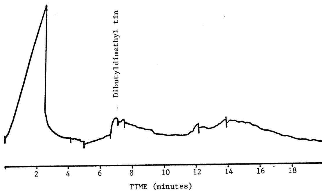
Figure 19. Total ion current chromatogram of Grignard methylation products of sample #14C.
