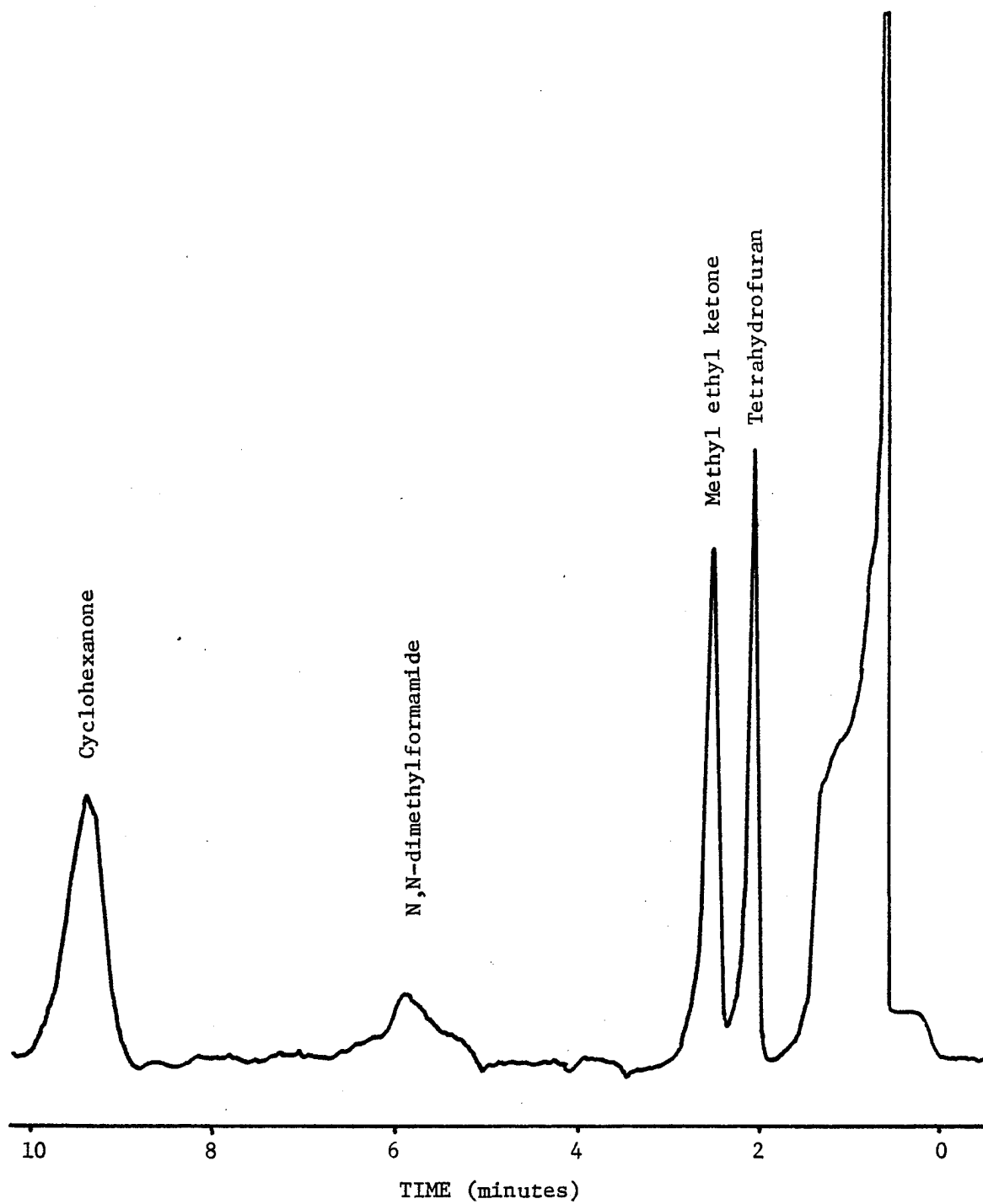
Figure 23. Gas chromatogram of aqueous cement solvent standard on a column of 1% SP-1000 on 60/80 Carbopack B at 170°C.
