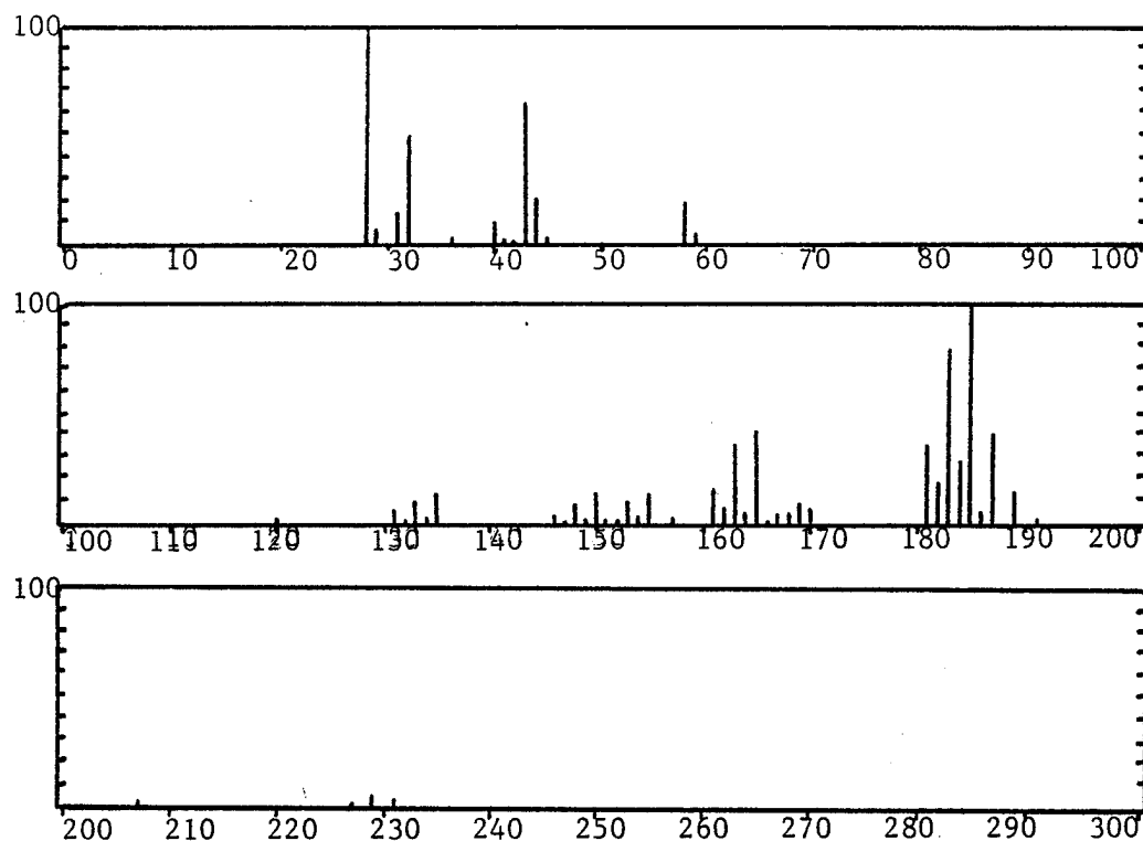
Figure A-9. Mass spectrum of trimethyltin chloride.
