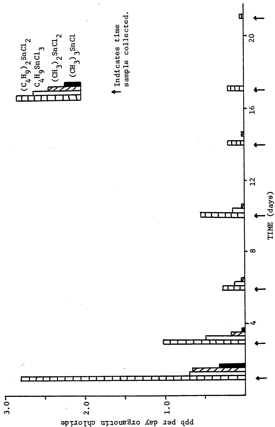
Figure 27. Standardized organotin chloride concentrations observed in CPVC #14C pipe loop water samples.
