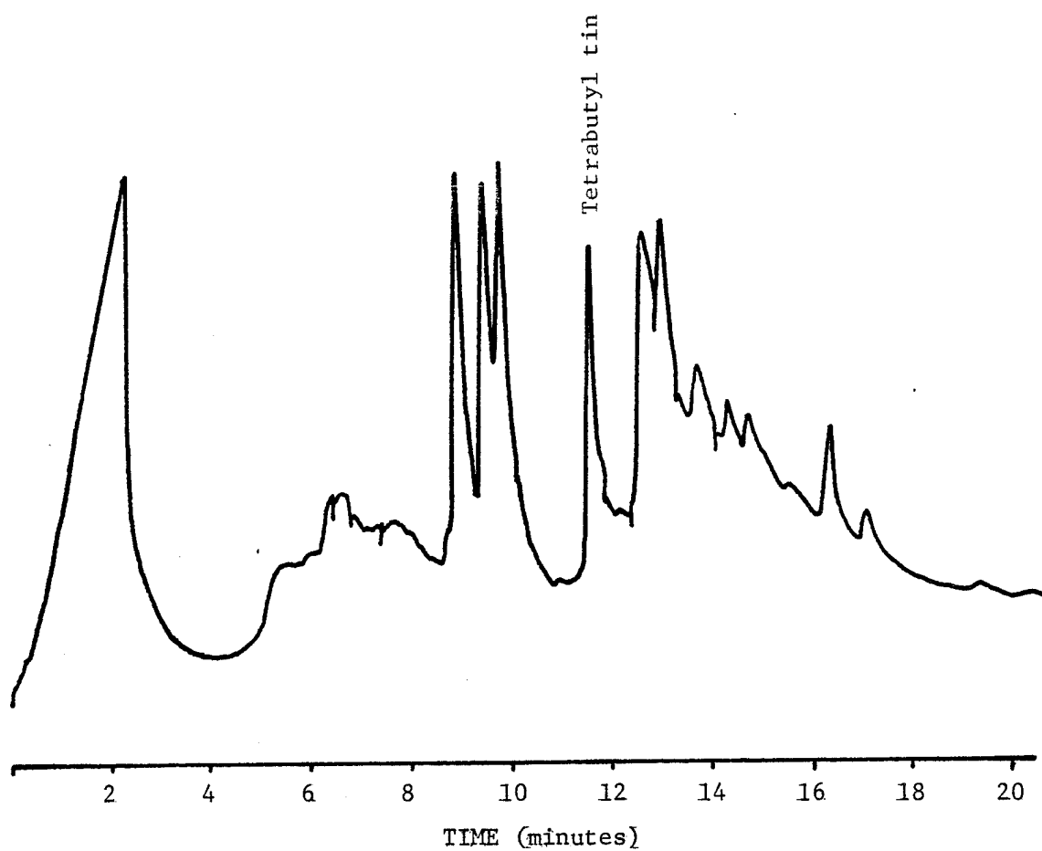
Figure 17. Total ion current chromatogram of Grignard butylation products of sample #14C.
