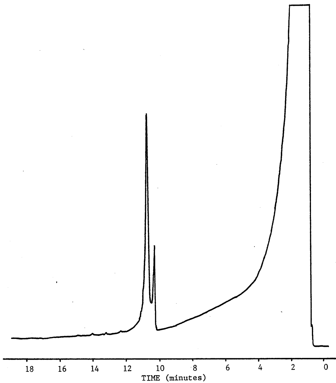
Figure A-6. Gas chromatogram of isooctyl thioglycolate.
