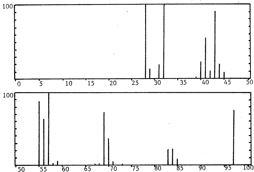
Figure 14. Mass spectrum of the 3.2-minute peak in Figure 13.
