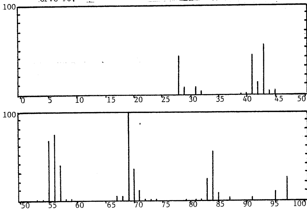
Figure 11. Mass spectrum of the 3.8-minute peak in the chromatogram of CPVC #6.
