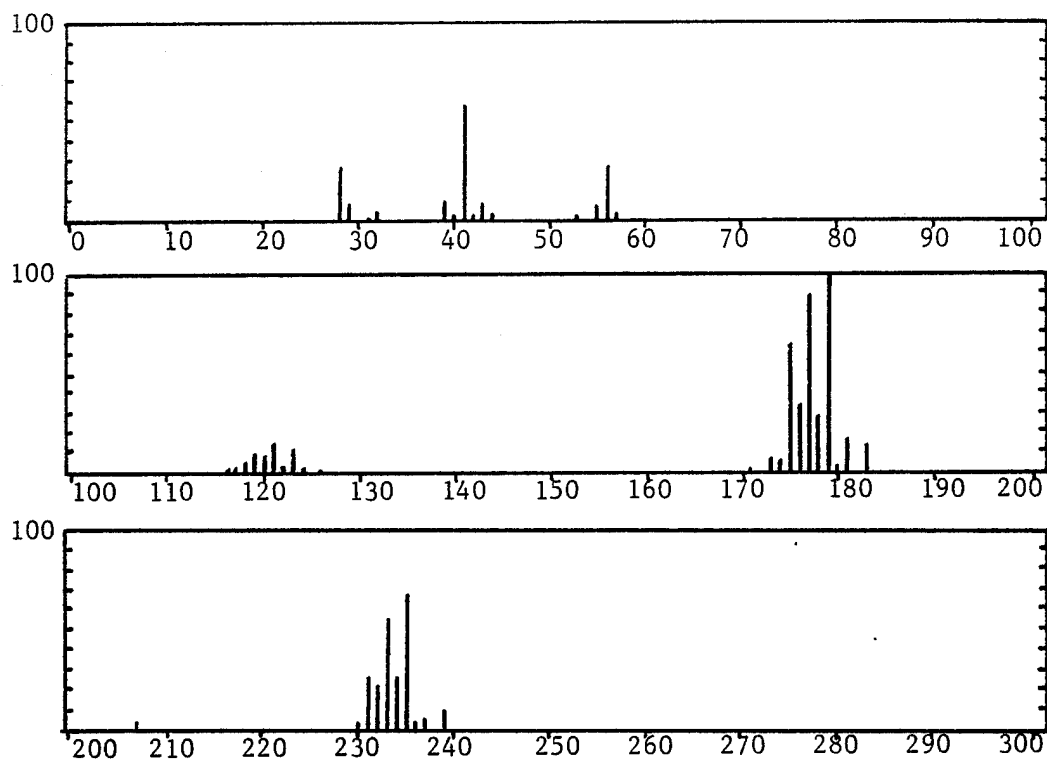
Figure A-11. Mass spectrum of tributyltin hydride.
