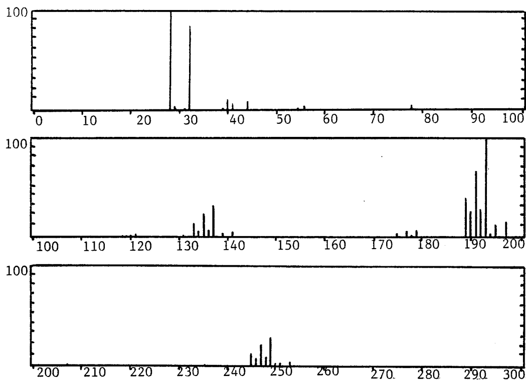
Figure A-13. Mass spectrum of tributylmethyl tin.
