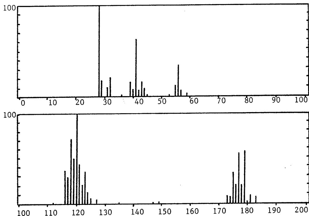
Figure A-10. Mass spectrum of dibutyltin dihydride.
