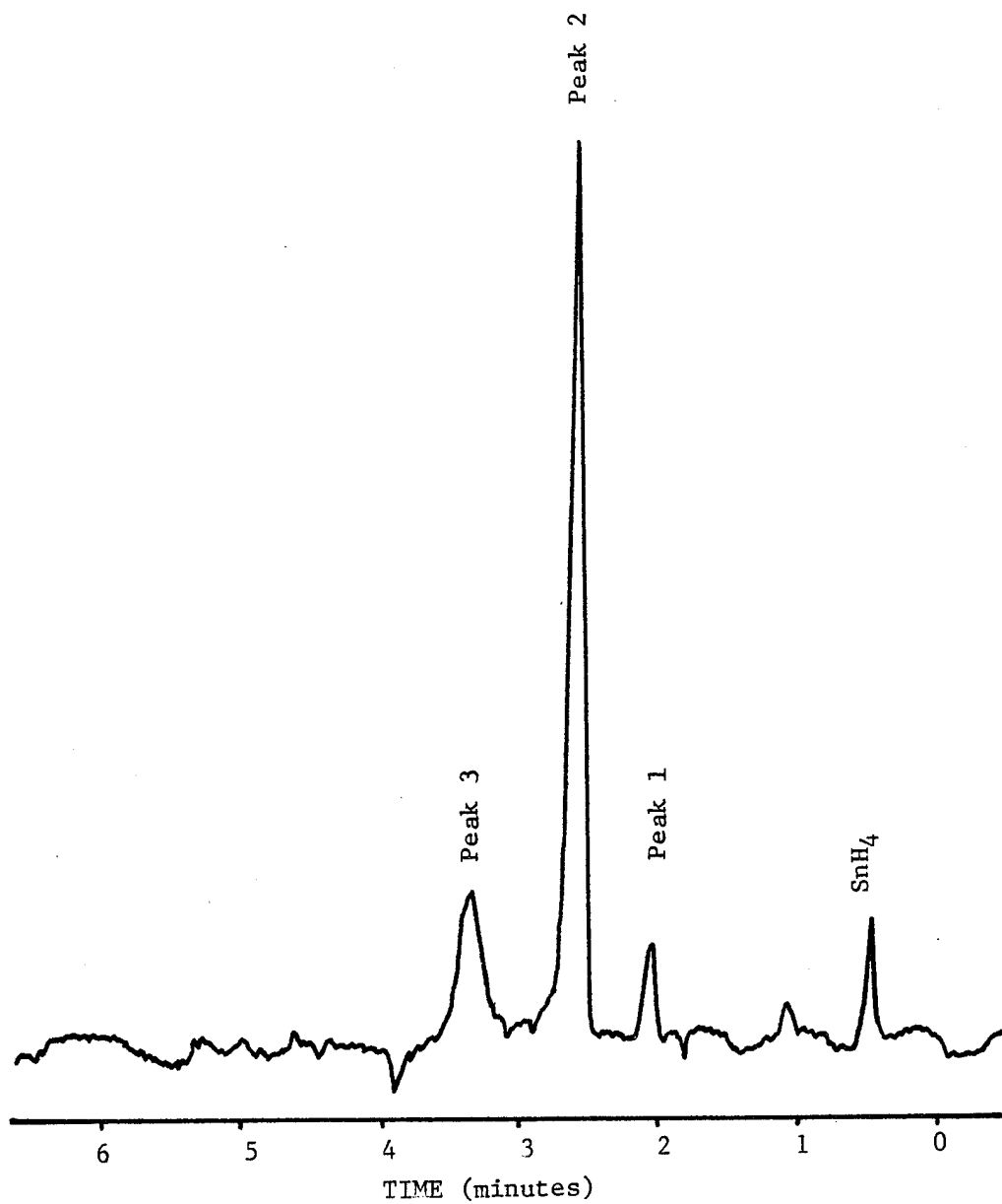
Figure 24. Hydride-generation atomic absorption analysis of tap water blank, showing three unidentified organotin species.
