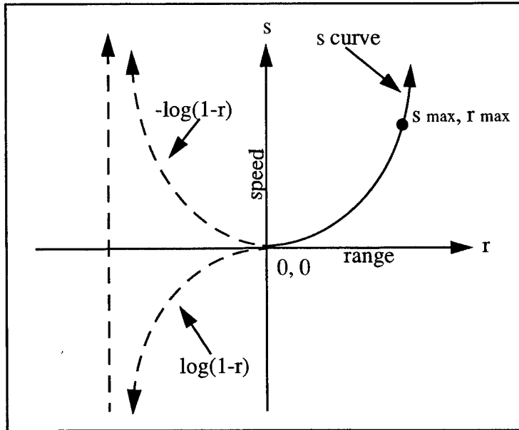
Figure 22: Rocket approximation
