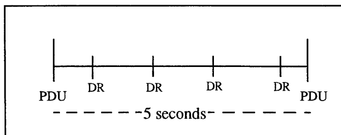
Figure 4: PDU and DR time
