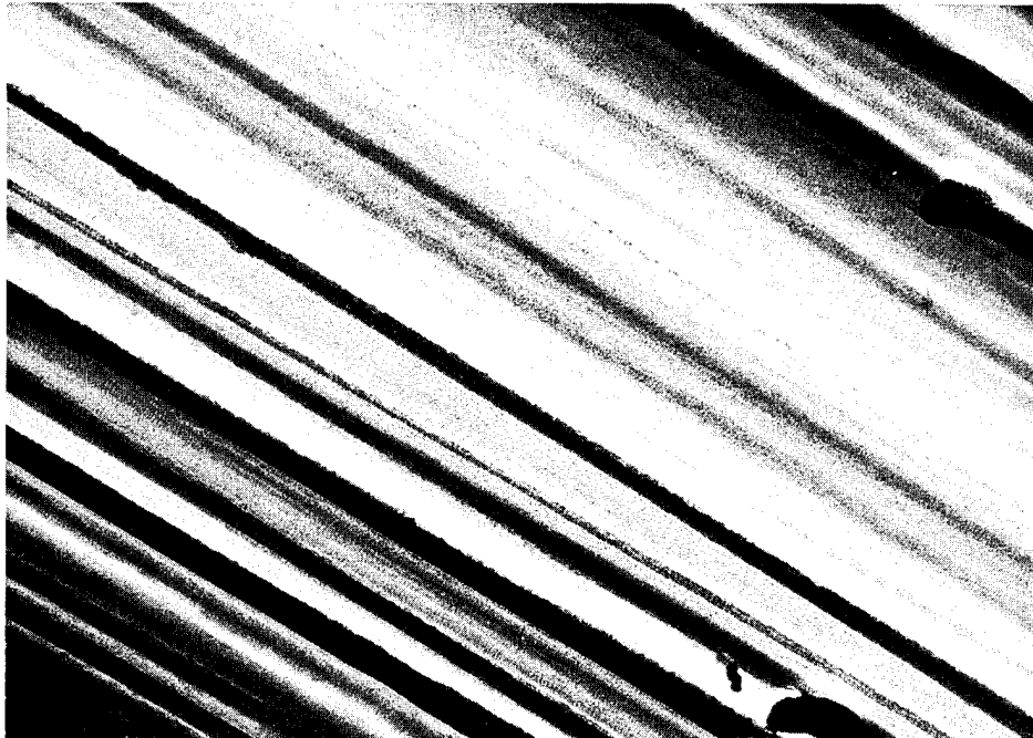
Figure 7. Photomicrograph of HT Graphite Fiber.
