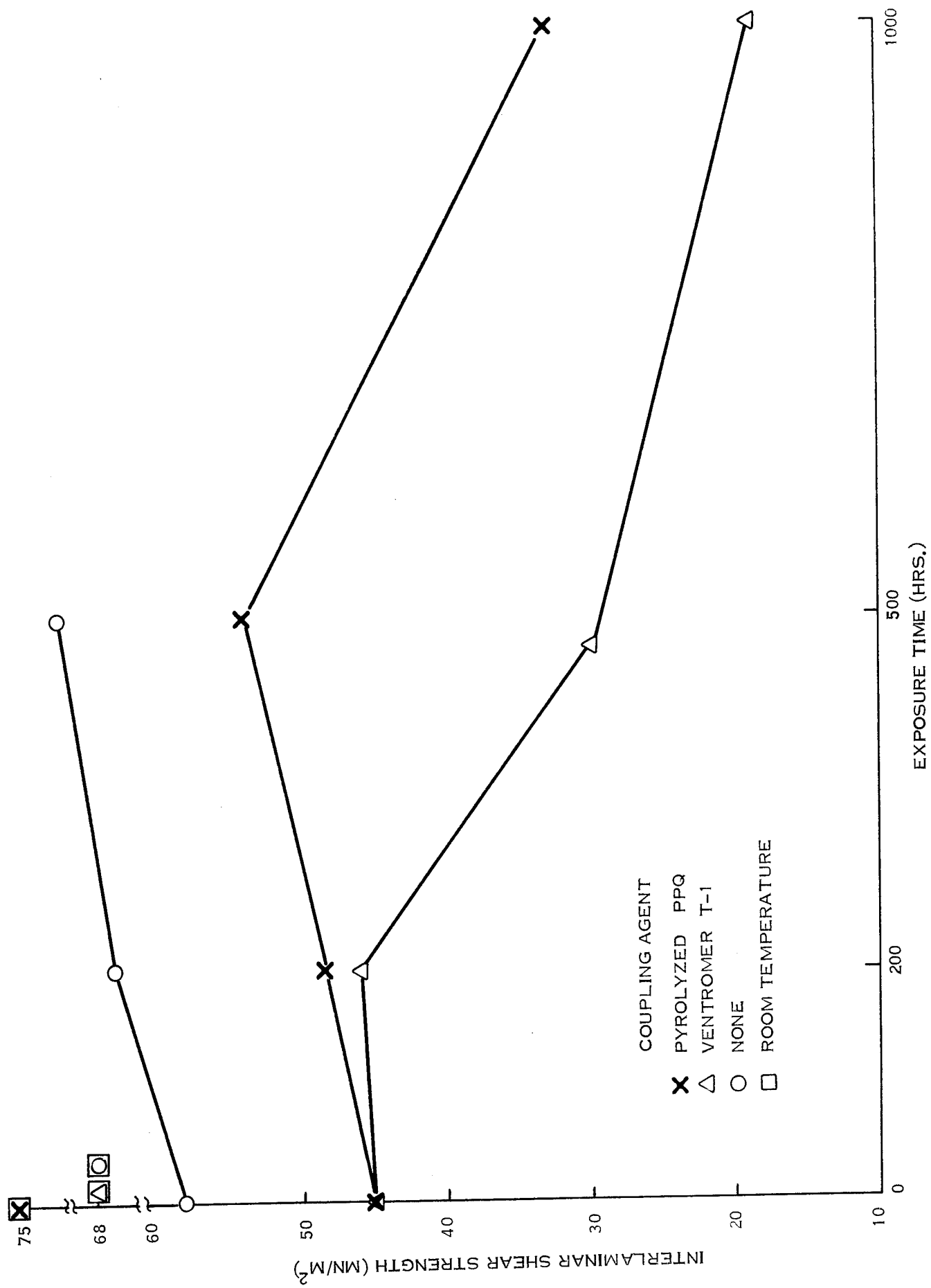
Figure 32. Interlaminar Shear Strength of Polyphenylquinoxaline Composites Aged and Tested at 533K.
