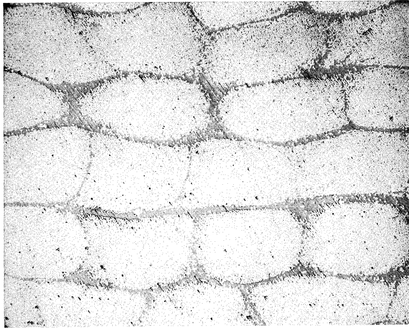
Figure 17. PPQ/Graphite Fiber Composite as Made.
