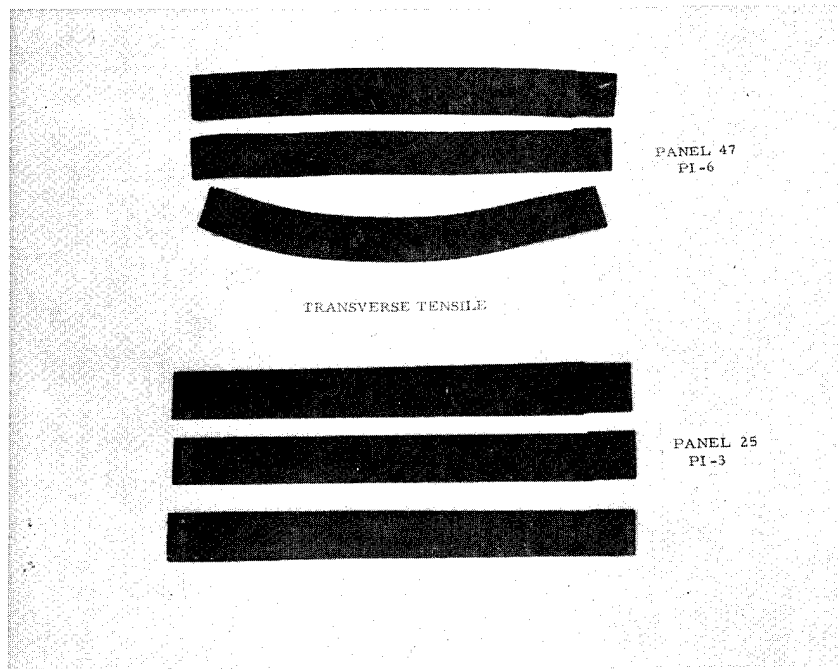
Figure 45. Polyimide Transverse Tensile Specimens After 1000 Hours at 588K.
