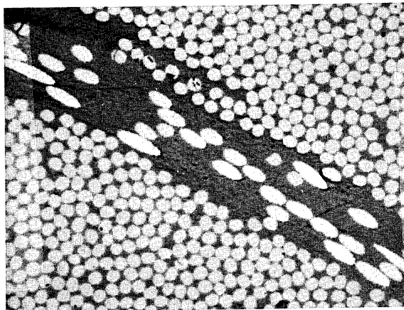
Figure 14. Photomicrograph of the Space Between Tows in a PPQ/Graphite Fiber Composite.
