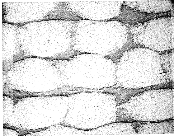
Figure 13. Photomicrograph of a PPQ/Graphite Fiber Composite.
