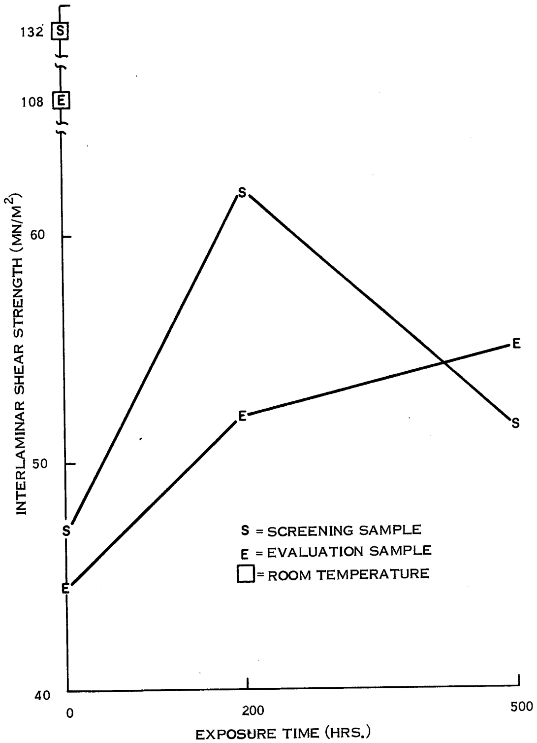
Figure 23. Interlaminar Shear Strength of Screening and Evaluation Polyimide Composites Made With Pyrolyzed PPQ Coupling Agent, Aged and Tested at 588K.
