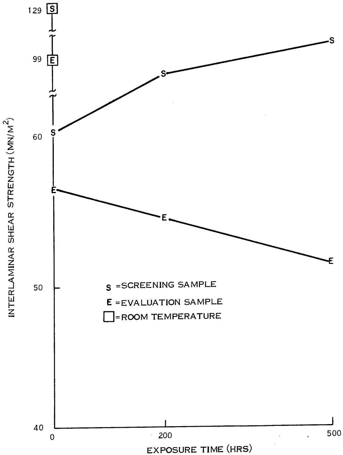
Figure 22. Interlaminar Shear Strength of Screening and Evaluation Polyimide Composites Made With Ventromer T-1 Coupling Agent, Aged and Tested at 588K.
