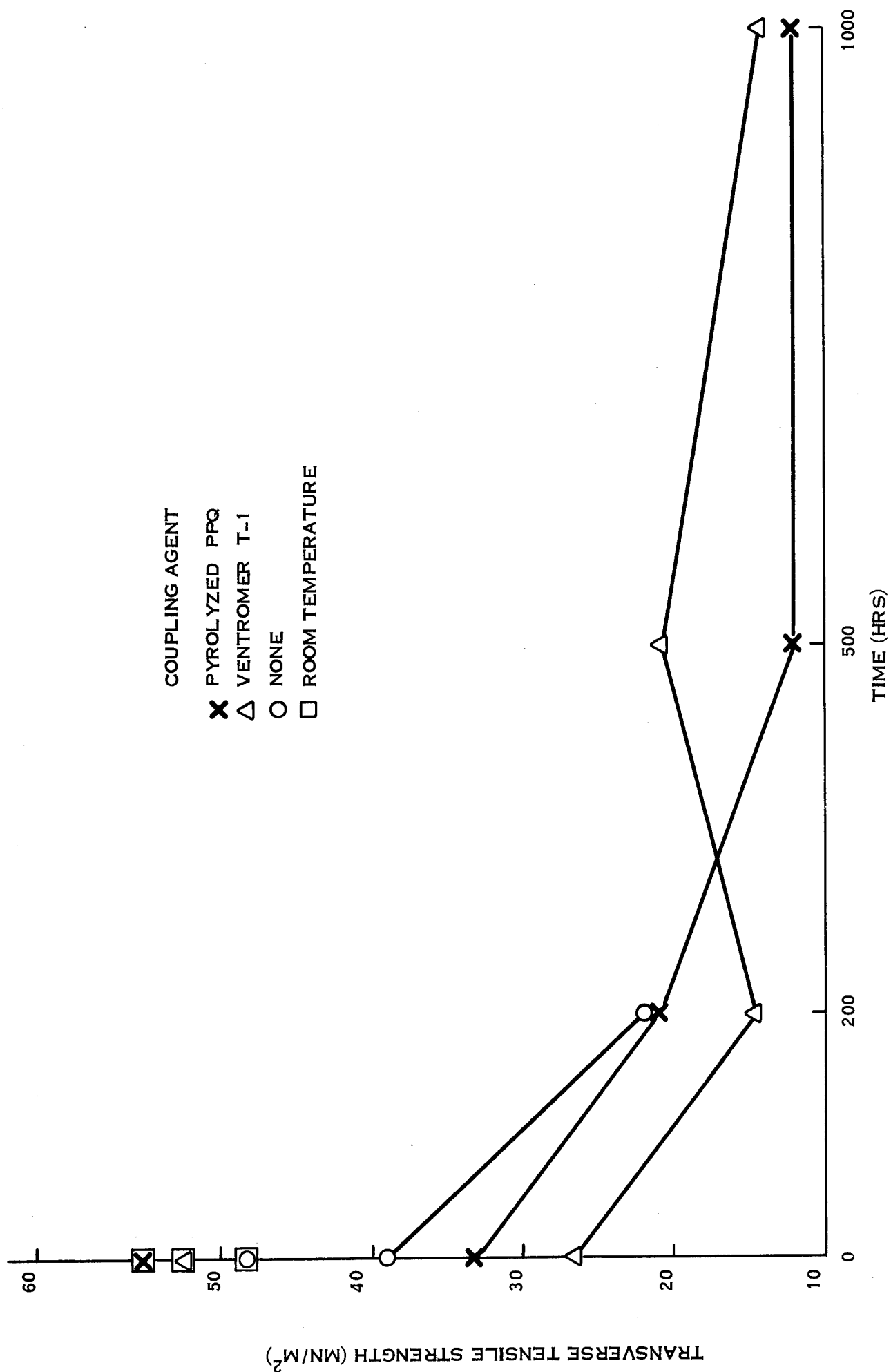
Figure 42. Transverse Tensile Strength of Polyimide Composites Aged and Tested at 533K.
