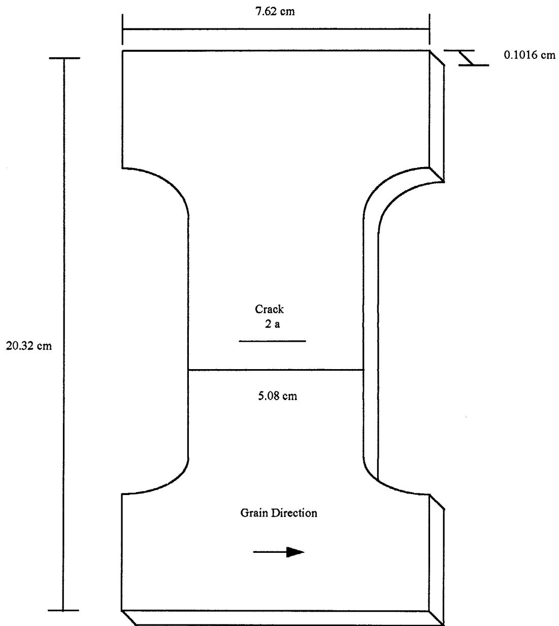
Figure 2. MT Specimen
