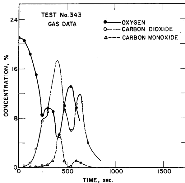
Figure 22. Results of continuous \text{CO} , \text{CO}_2 , and \text{O}_2 measurement from wool carpet.
