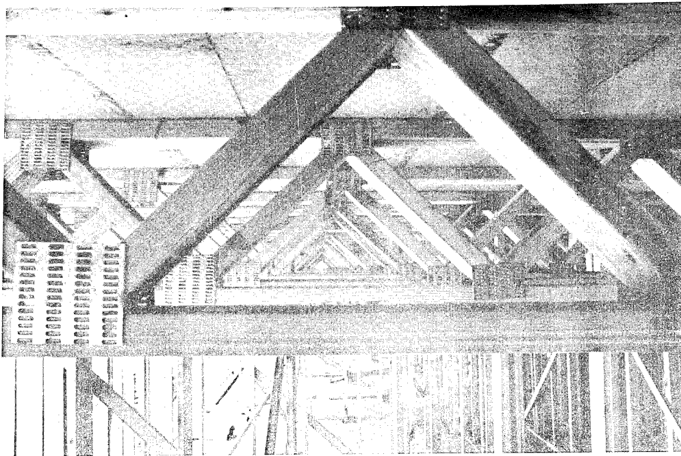
Figure 7. These trussed floors permit a combustible void over and under the four apartments on a floor. Vertical channels may interconnect the several voids. In such a structure it is possible to envision collapse not long after fire penetrates the void.
