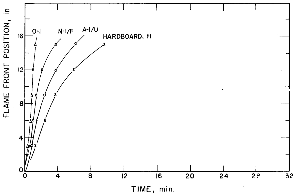
Figure 12. E-162 flame spread results.
