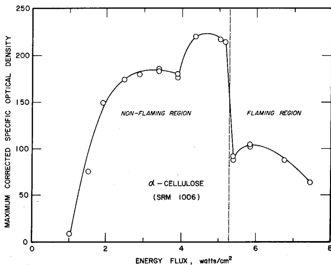
Figure 6. Effect of energy flux on maximum corrected specific optical density of \alpha -cellulose (SRM 1006).
