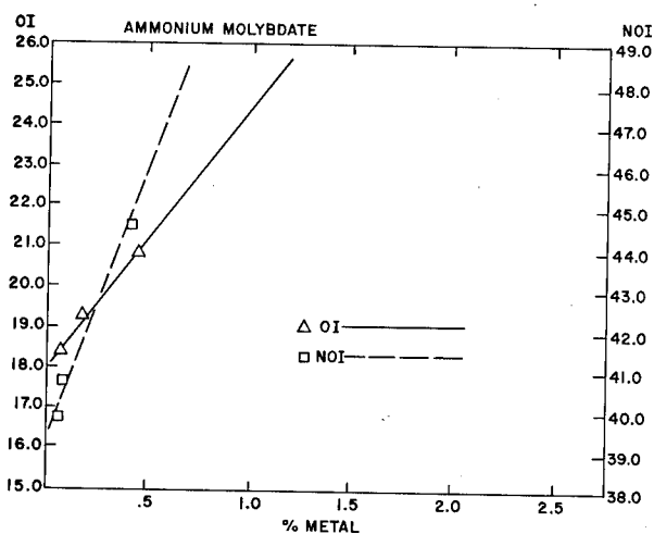
Figure 10. Cotton fabric treated with ammonium molybdate.
