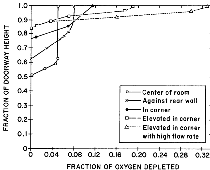
Figure 8. Vertical oxygen depletion profiles in the model for different burner locations and gas flow rates. See figure 9 for position of burner with respect to floor plan.
