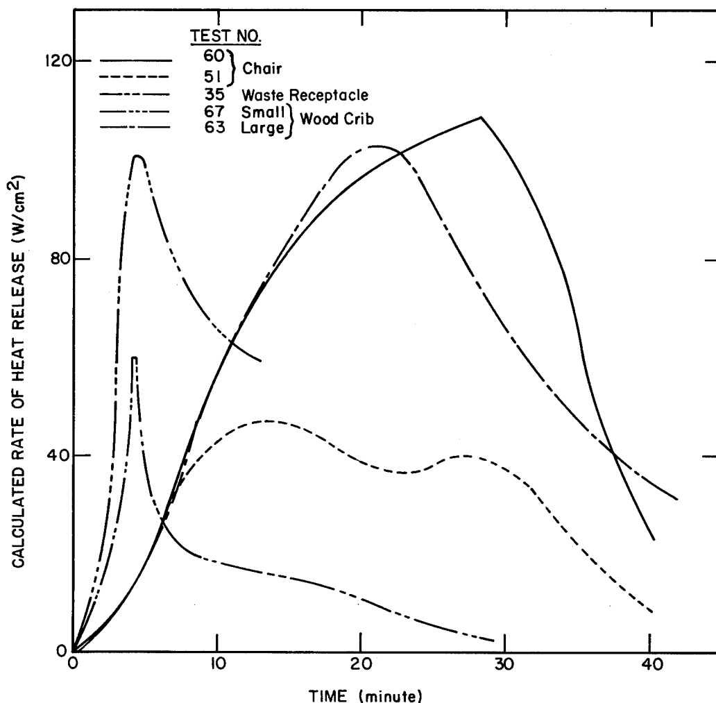
Figure 4. Comparison of calculated rate of heat release for furniture, wood crib and waste receptacle fires.
