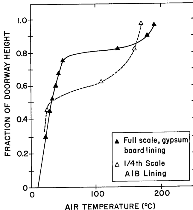
Figure 3. Temperature profile at doorway at 10 minutes for full and quarter scale enclosures.
