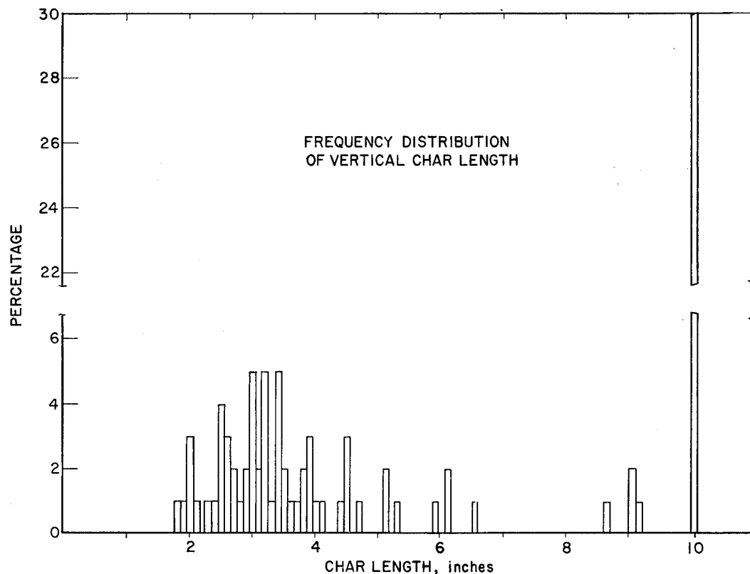
Figure 5. A histogram showing the distribution of average char length for a group of fabrics tested in the vertical test.
