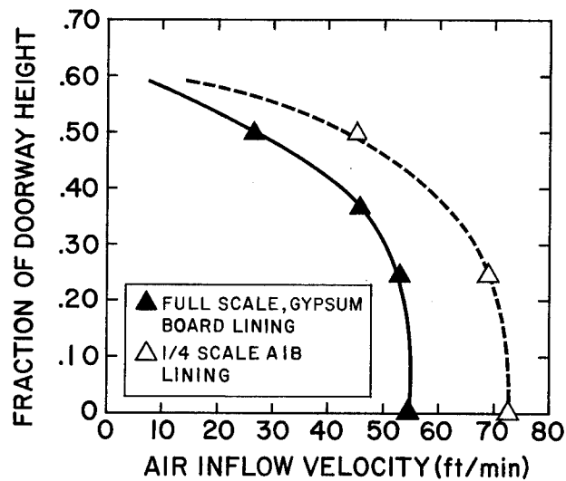
Figure 2. Velocity profile in doorway at 10 minutes for full and quarter scale enclosures. The velocity data for the full-scale test is scaled down by the square root of the ratio of the doorway heights.
