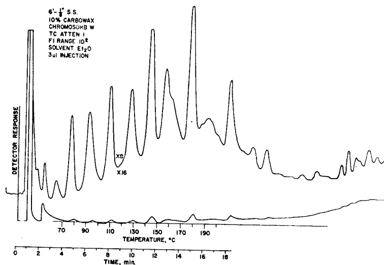
Figure 9. Gas chromatographic separation of smoke components.
