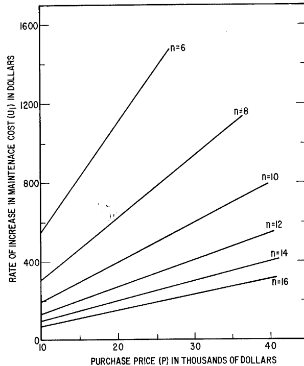
Figure 1. Contours of the optimum engine life.
