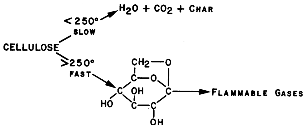
Figure 2. Decomposition of cellulose by two competing pathways.
