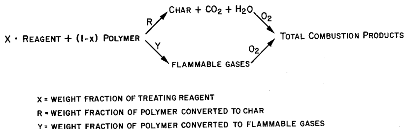
Figure 22. Thermo-decomposition pathways.
