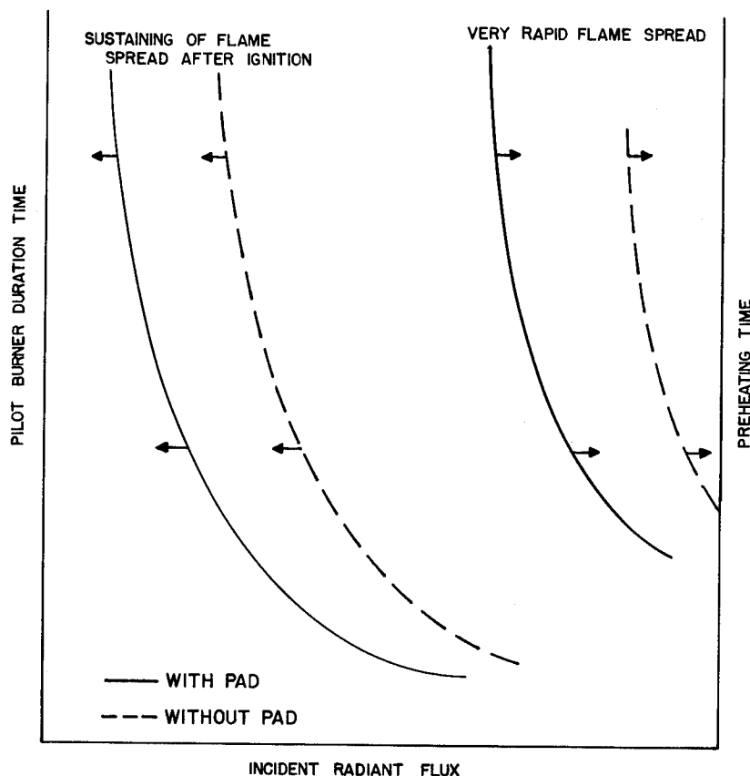
Figure 4. Qualitative relations between ignition and incident radiant flux and between flame spread velocity and incident radiant flux under variable preheating time.
