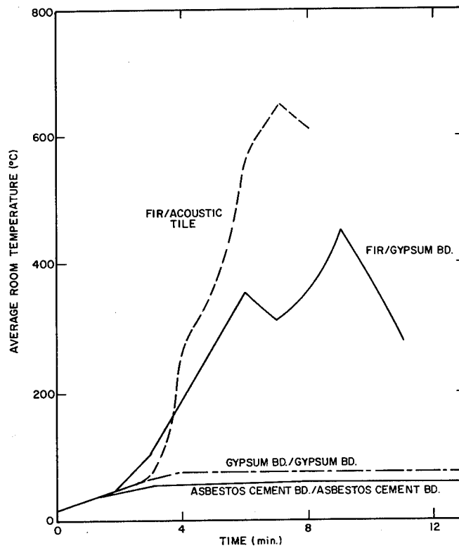
Figure 5. Effect of material combination of wall and ceiling linings on average room air temperature. Legends on curves indicate wall/ceiling material.
