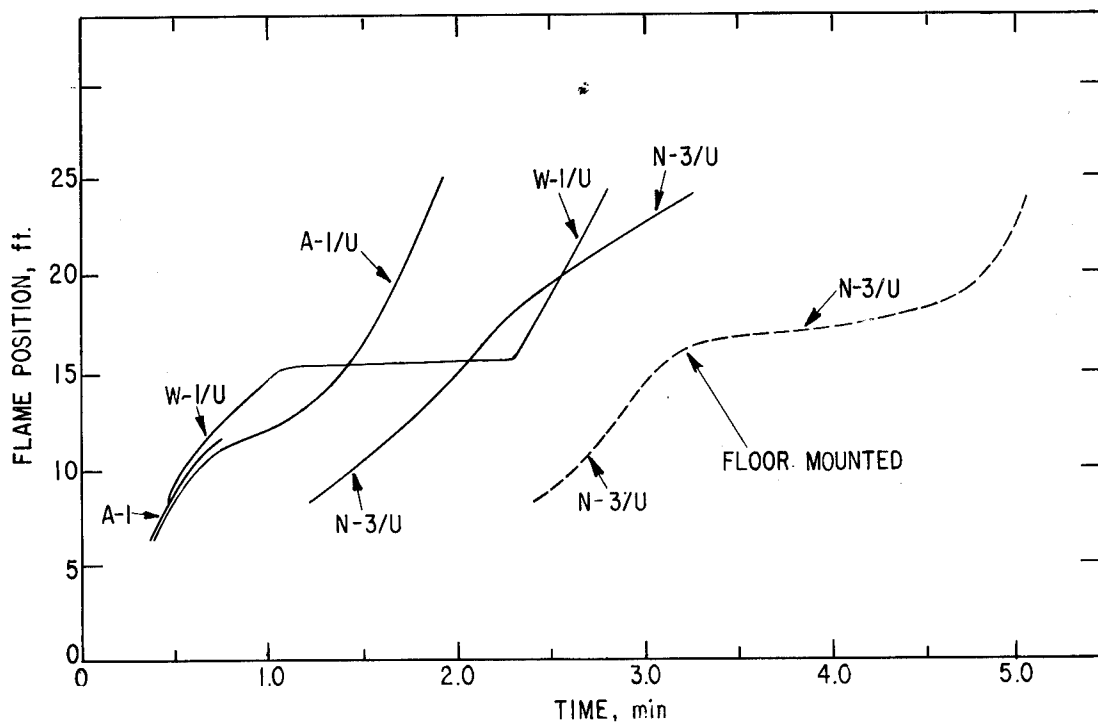
Figure 11. E-84 flame Spread results.
