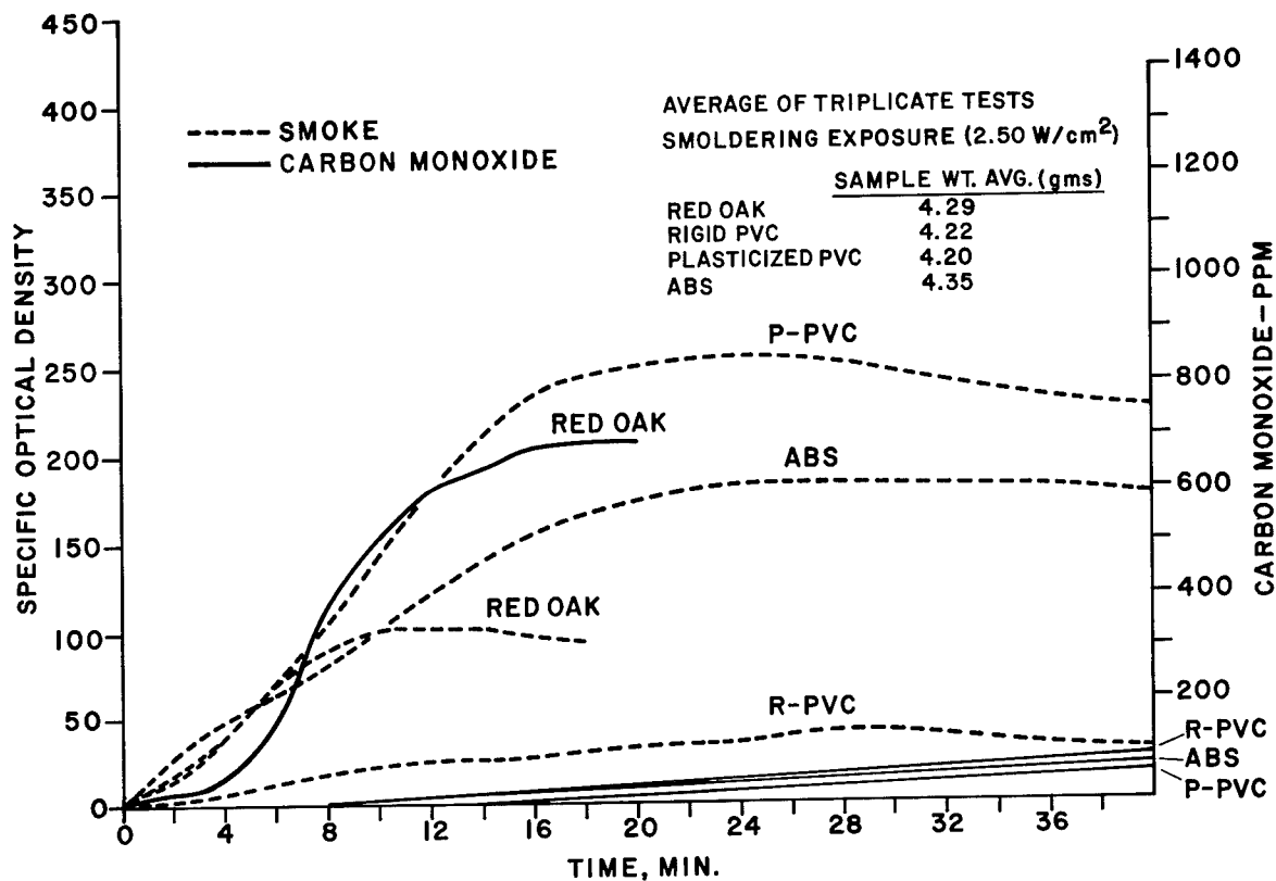
Figure 2. Smoke and carbon monoxide concentration for various materials.
