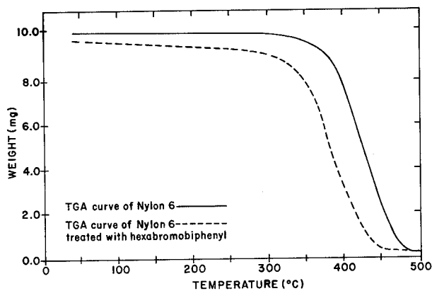
Figure 19. Plot of the thermo-gravimetric analysis (TGA) curve of Nylon 6 compared to the TGA curve of Nylon 6 treated with Hexabromobiphenyl. Samples were decomposed at a heating rate of 6°C per minute.
