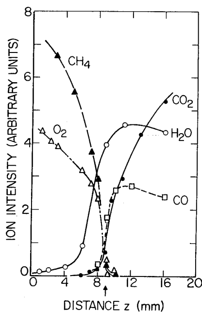
Figure 3. Concentration profiles for major reactants and products in a 1 Atm fuel-rich \text{CH}_4 - \text{O}_2 flame.
