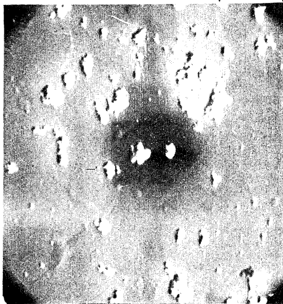
Figure 8. Plasticized PVC "flaming exposure" smoke particulate, scanning electron microphotograph.
