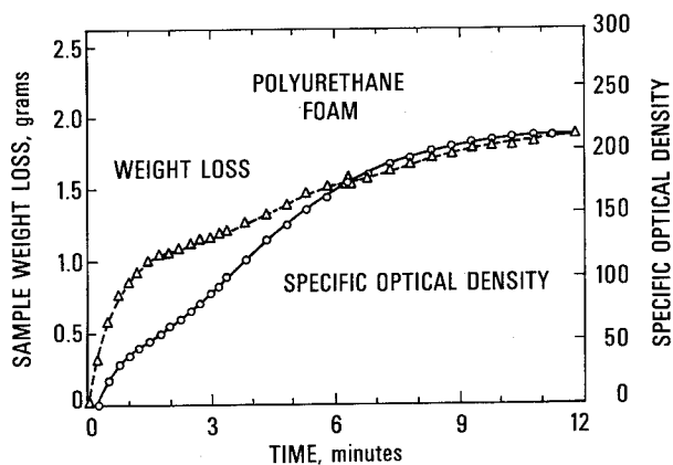
Figure 4. Specific optical density and sample weight loss curves for polyurethane foam (TDI-type).
