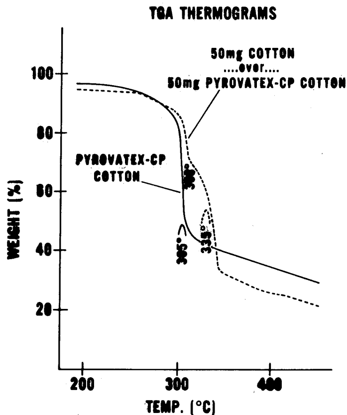
Figure 6. Weight losses on heating in air at 15°/min: Pyrovatex-CP treated cotton and untreated cotton.
