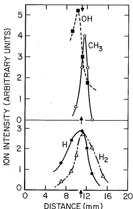
Figure 4. Concentration profiles for the main radical species in a fuel-rich \text{CH}_4 - \text{O}_2 flame.
