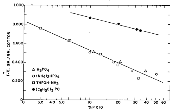
Figure 23. Estimated tar formation for treated cotton.
