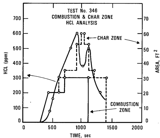
Figure 24. Results of continuous HCl measurement.
