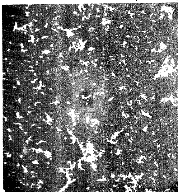
Figure 10. ABS "flaming exposure" smoke particulate, scanning electron microphotograph.
