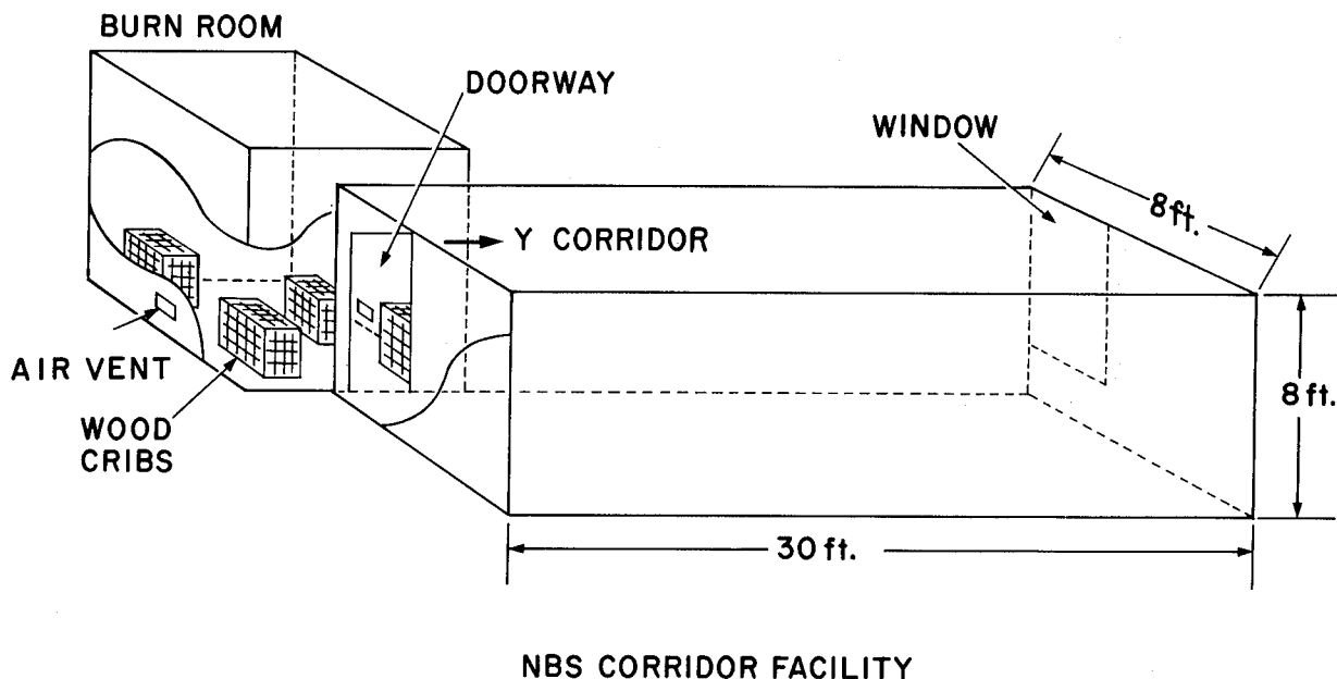
Figure 1. NBS corridor facility.
