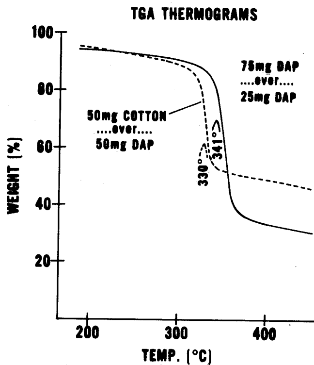
Figure 4. Weight losses on heating in air at 15°/min: Cotton/DAP two-layer systems.
