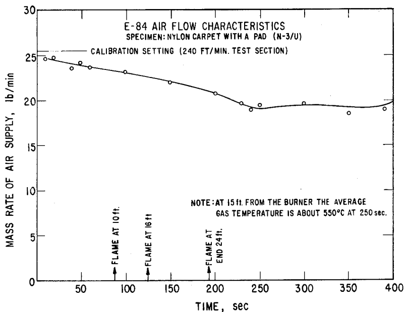
Figure 10. E-84 air flow characteristics.
