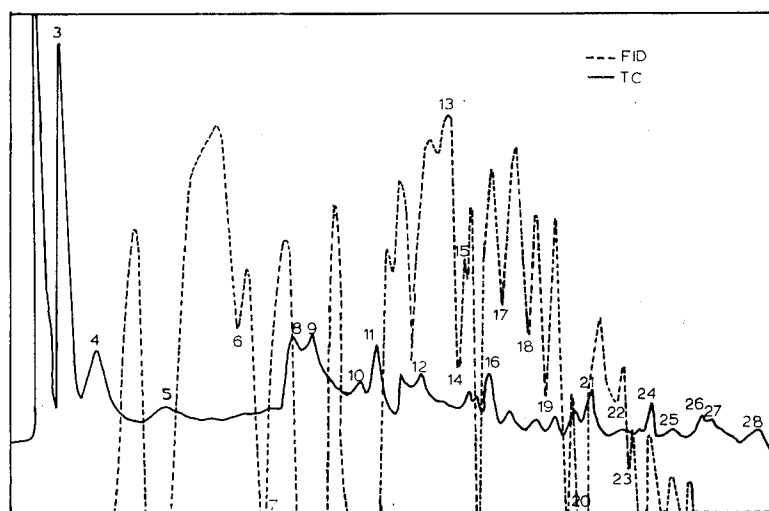
Figure 10. Dual detector chromatogram - combustion of flexible-urethane foam
