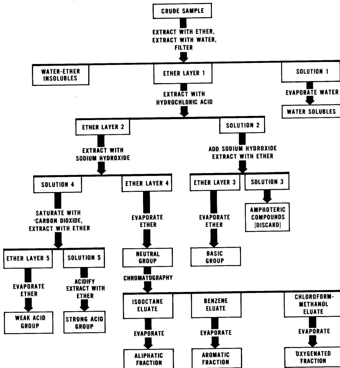
Figure 8. Schematic for separation of smoke into compound classes.
