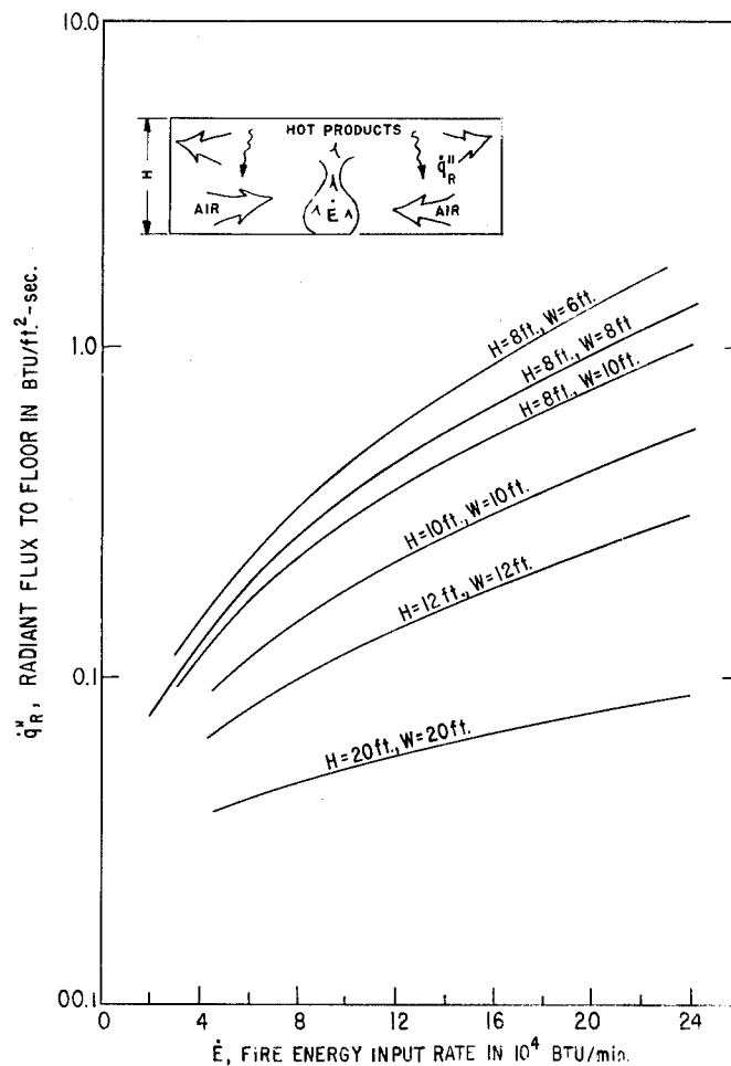
Figure 15. Estimated radiant flux to floors in building corridor fires.
