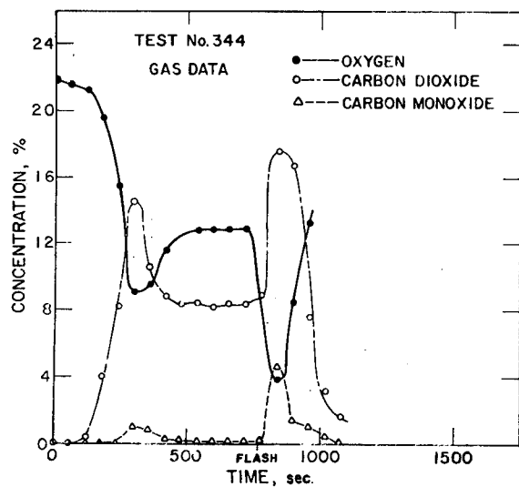
Figure 23. Results of continuous \text{CO} , \text{CO}_2 and \text{O}_2 measurement from nylon carpet.
