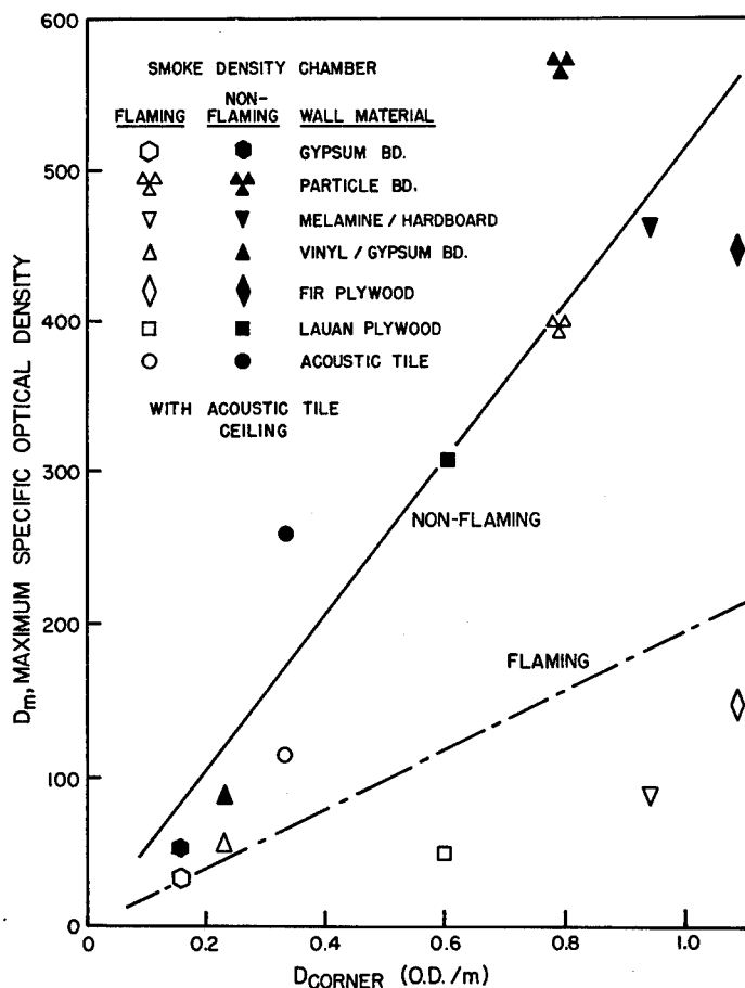
Figure 10. Comparison of the results of accumulated smoke measurement by smoke density chamber and maximum observed smoke level in the room during a corner fire test.
