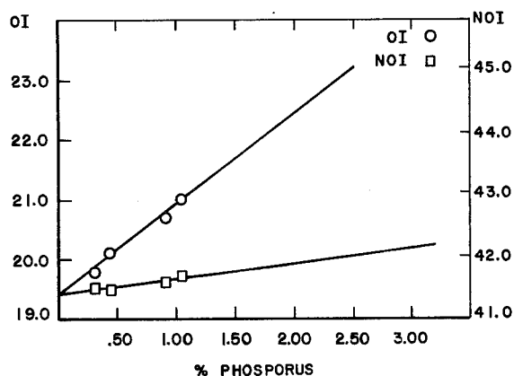
Figure 13. Plot of Oxygen Index (OI) and Nitrous Oxide Index (NOI) versus percent phosphorus for triphenylphosphine oxide.
