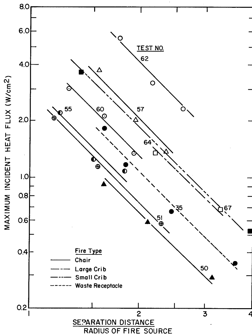
Figure 3. Relationship between incident heat flux at various locations and dimensionless separation distance.
