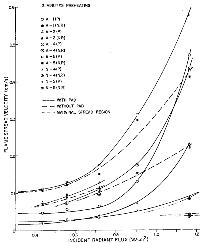
Figure 3. Relation between flame spread velocity and incident radiant flux.
