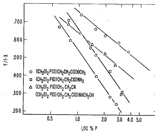
Figure 26. Flammable gas production from cotton treated with aliphatic phosphonates.
