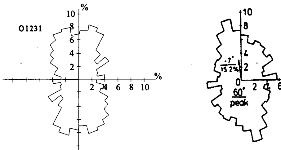
Figure 87. Frequency distribution of contact normals for numerical (left) and physical samples with a/b = 1.1 , \theta = 60^\circ and \phi_\mu = 52^\circ at peak strength.
