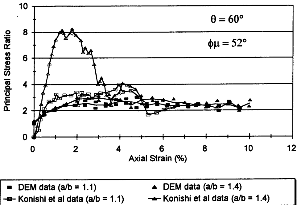
Figure 60. Comparison of DEM and Konishi et al results for samples with 60° bedding and interparticle sliding friction angle \phi_\mu of 52°.
