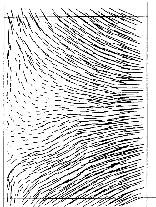
Figure 165. Particle displacements for a DEM sample with a/b = 3.0 and 0^\circ bedding at 10% axial strain.
