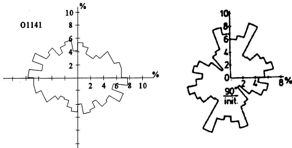
Figure 76. Frequency distribution of contact normals for numerical (left) and physical samples with a/b = 1.1 , \theta = 90^\circ and \phi_\mu = 26^\circ prior to shear.
