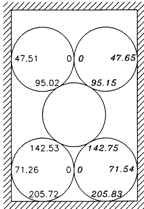
Figure 9. Comparison of theoretical and computed ( italicized ) normal contact forces for a symmetric frictionless, close-packed five disk system subjected to gravity loading. Values in kN.
