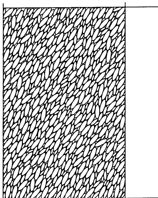
Figure 172. System plot of DEM sample with a/b = 3.0 and 60^\circ bedding prior to biaxial shear.
