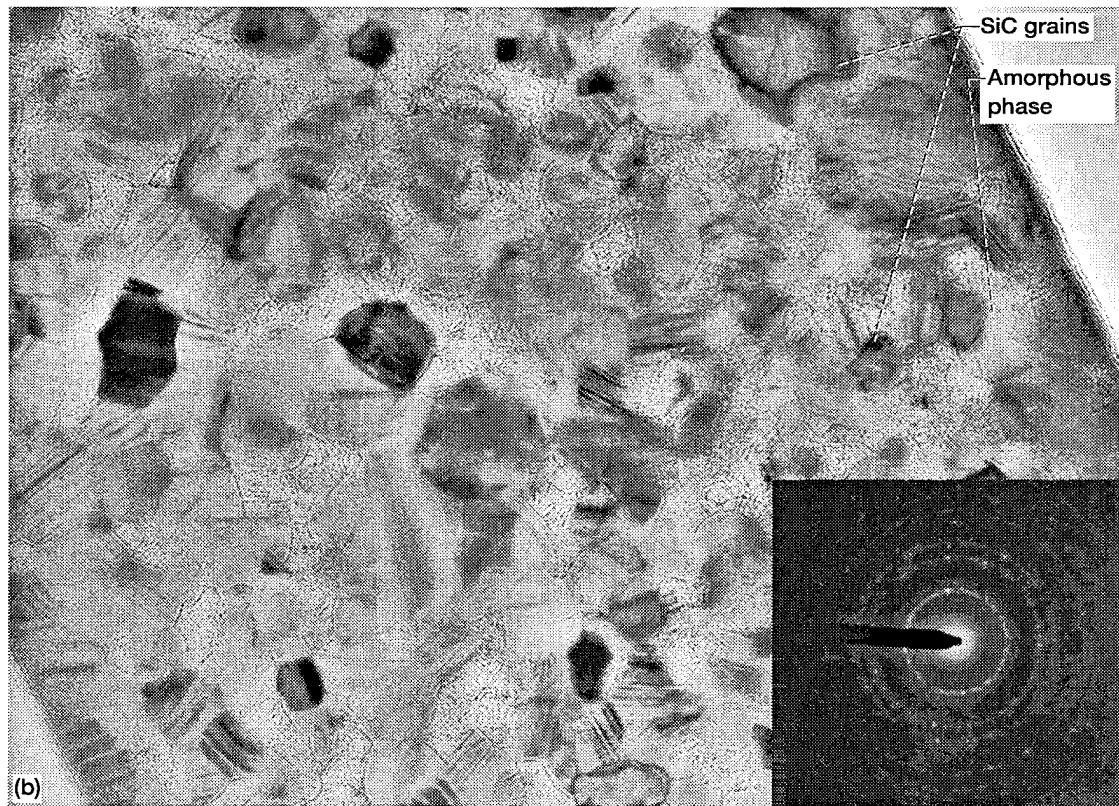
Figure 6.—TEM micrographs showing microstructure of the longitudinal sections of uncoated Hi-Nicalon SiC fibers. (a) As-received (dark field image). (b) After heat treatment in nitrogen at 1800 °C for 100 hr (bright field image).
