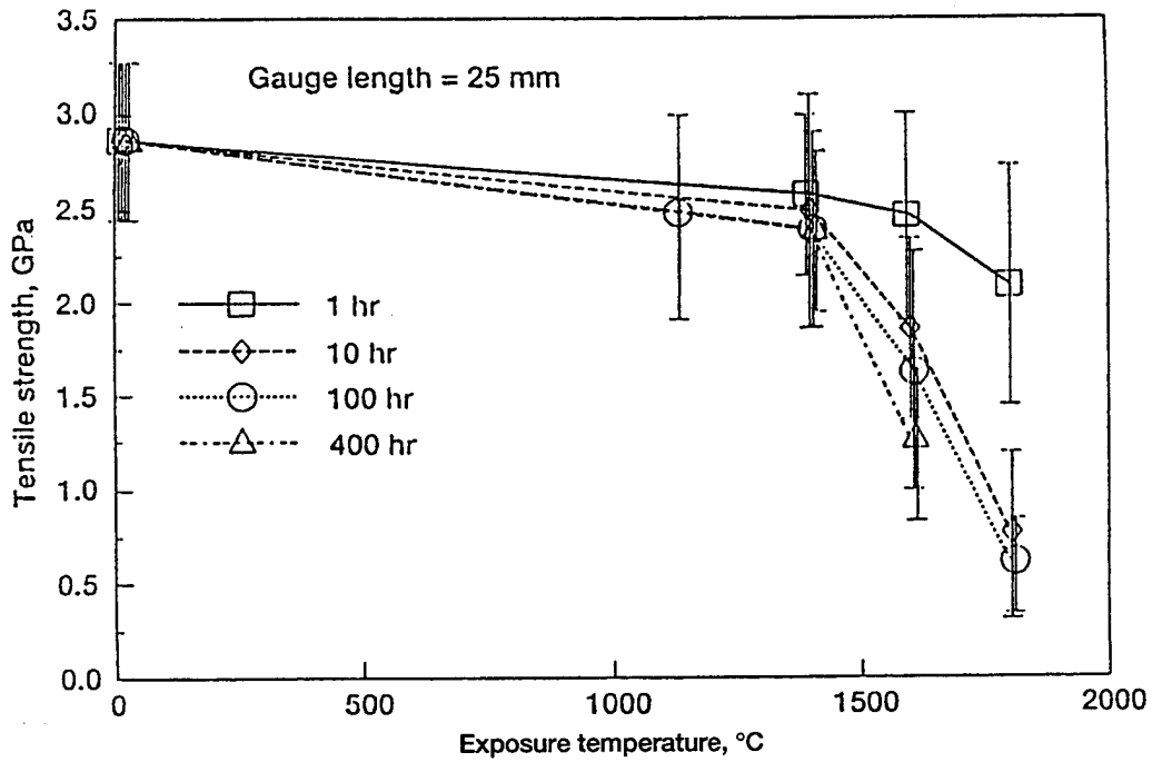
Figure 1.—Time and temperature effects on room temperature tensile strength of uncoated Hi-Nicalon SiC fibers heat treated in 0.1 MPa in nitrogen.
