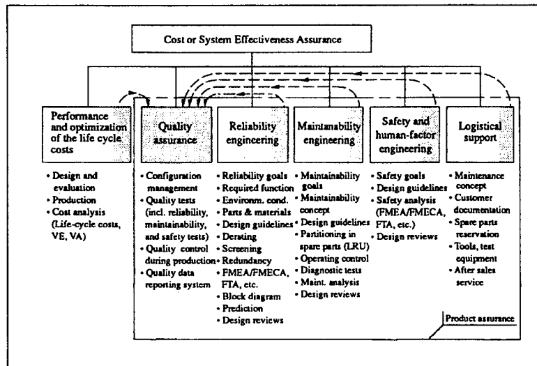
Figure 2. Cost or System Effectiveness Assurance Structure [Ref. 2]
