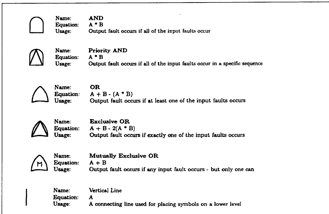
Figure 16. Fault Tree Logical Operator Symbology [Ref. 9]
