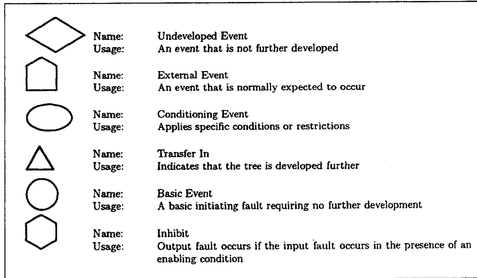
Figure 15. Fault Tree Event Symbology [Ref. 9]
