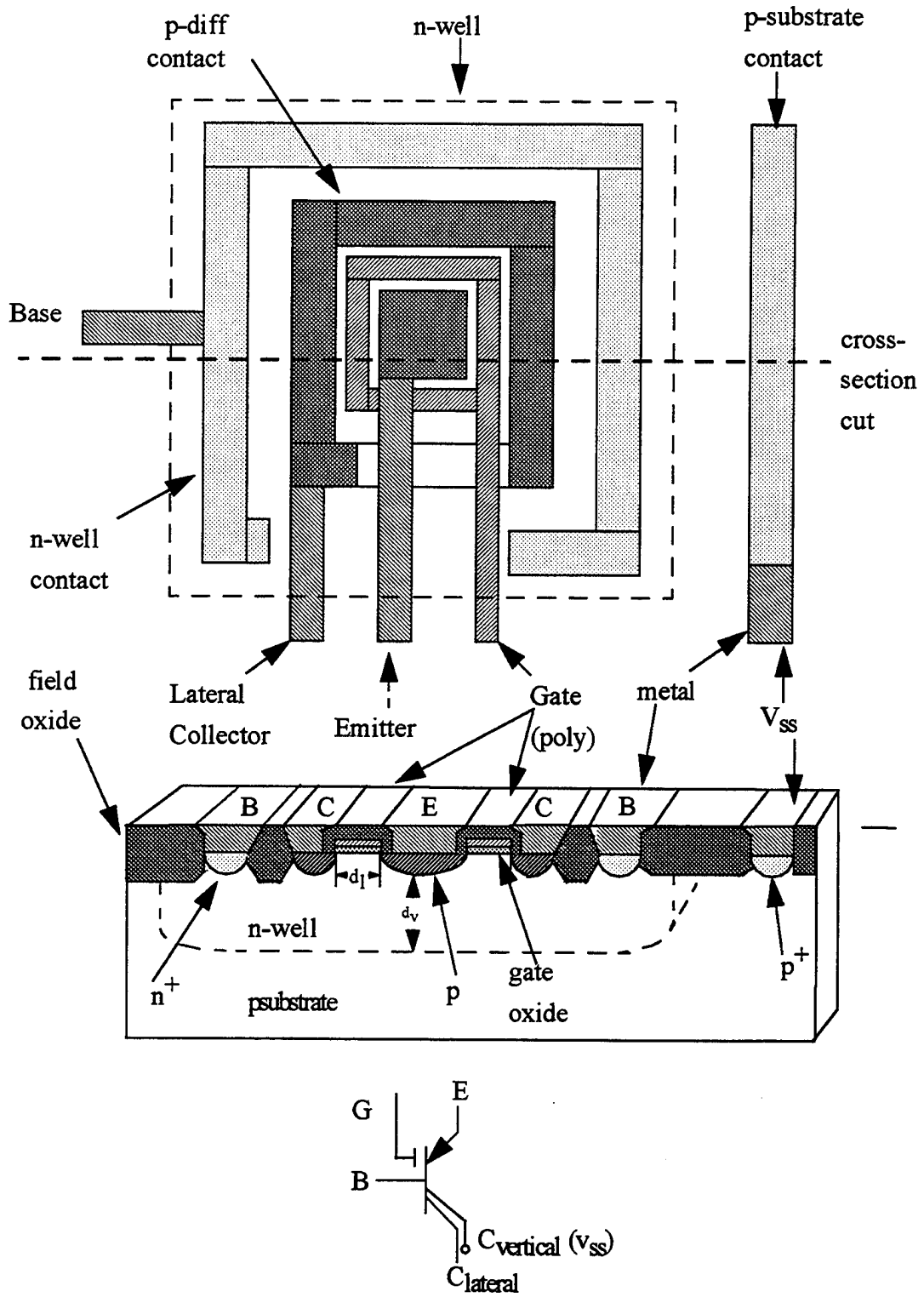
Figure 7: The layout of a single emitter dot lateral pnp bipolar transistor
