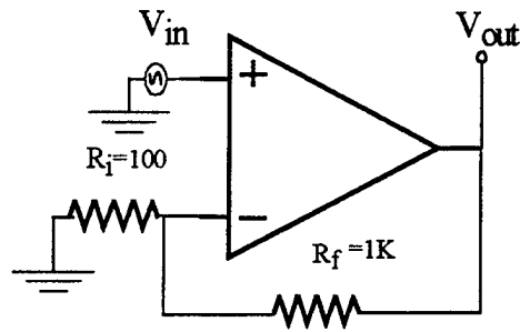
Figure 37: Non-inverting gain configuration
