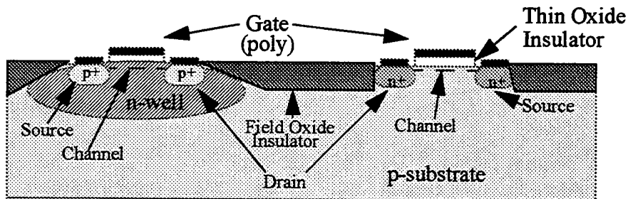
Figure 2: The CMOS n-well process
