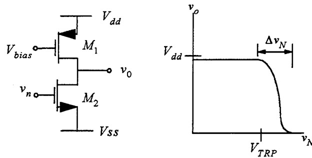
Figure 16: A simple inverting comparator and its dc transfer curve [Ref. 8 p. 327]
