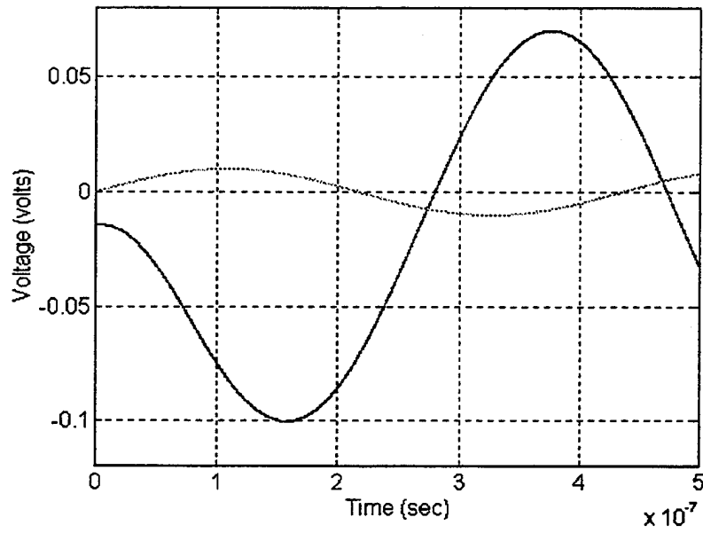
Figure 40: Inverting transient response (Frequency = 2.3 Mhz)
