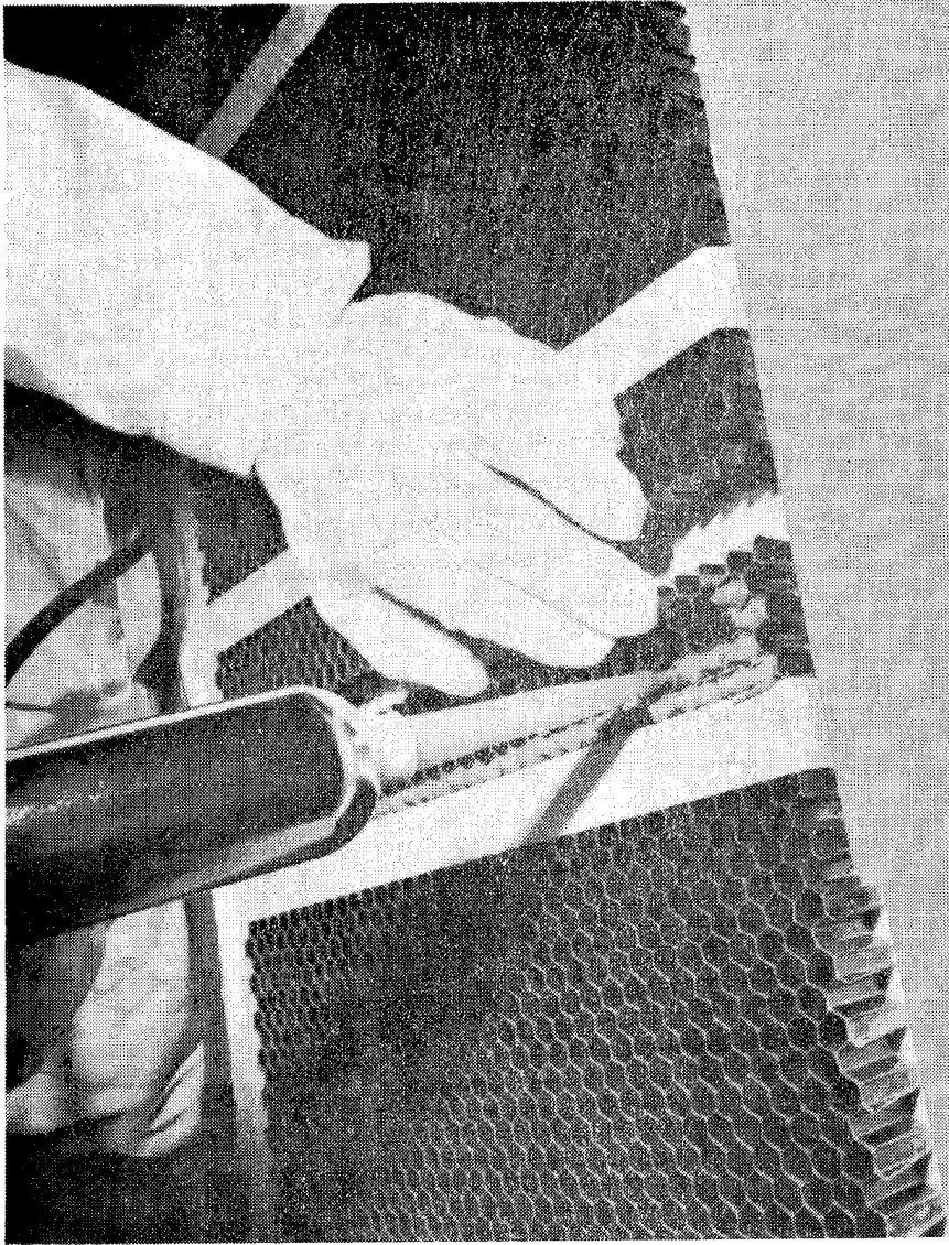
Figure 37.- Potting ends of honeycomb core with Br-34 polyimide adhesive.
