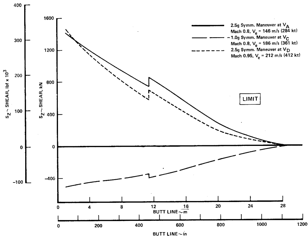
Figure 26. Design Wing Shears
