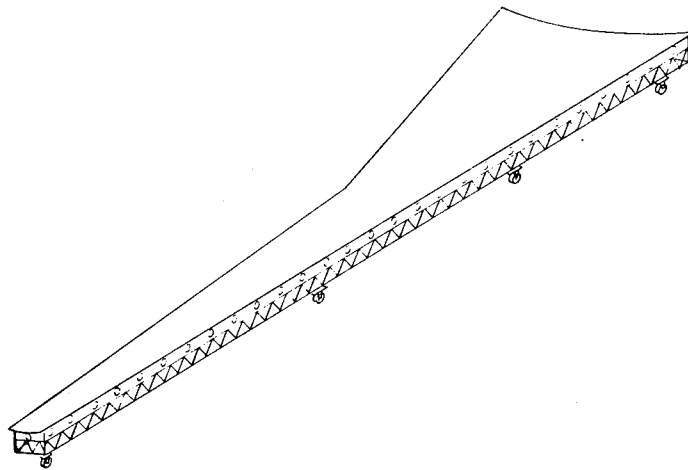
Figure 47. Skin Layup Tool
