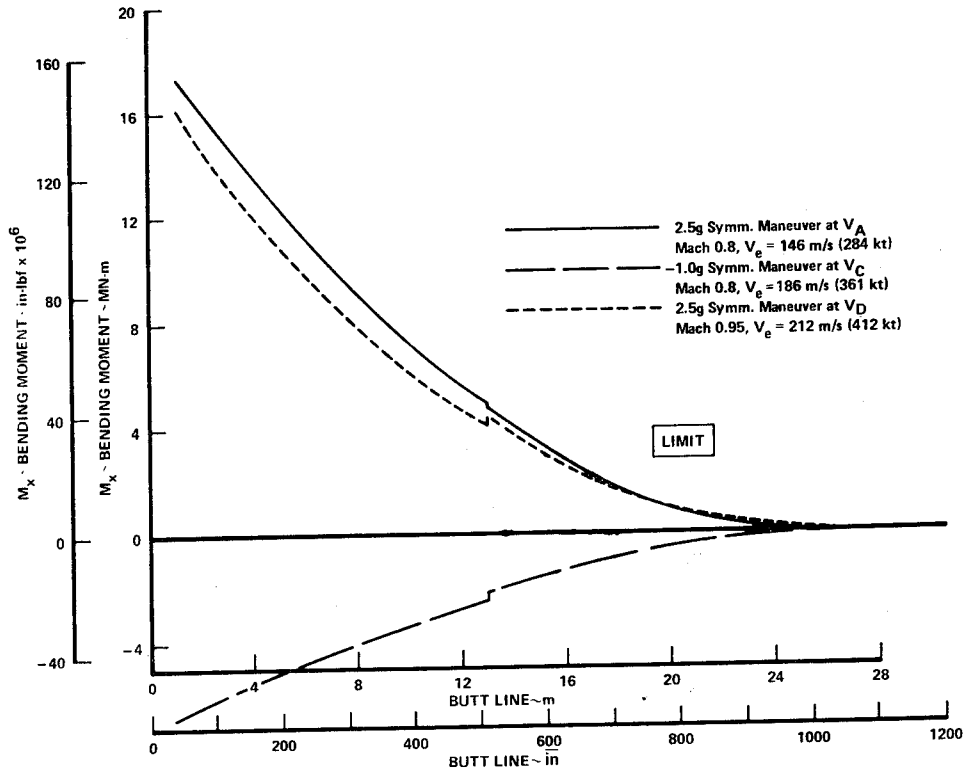
Figure 27. Design Wing Bending Moments
