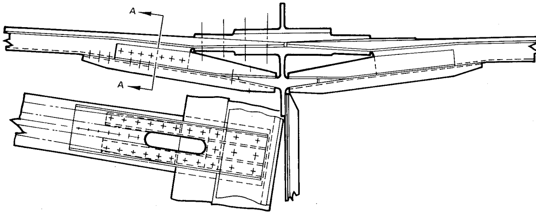
Figure 70. Composite Wing Production Joint Concept - BL118, Upper, for Hat-Stiffened Covers
