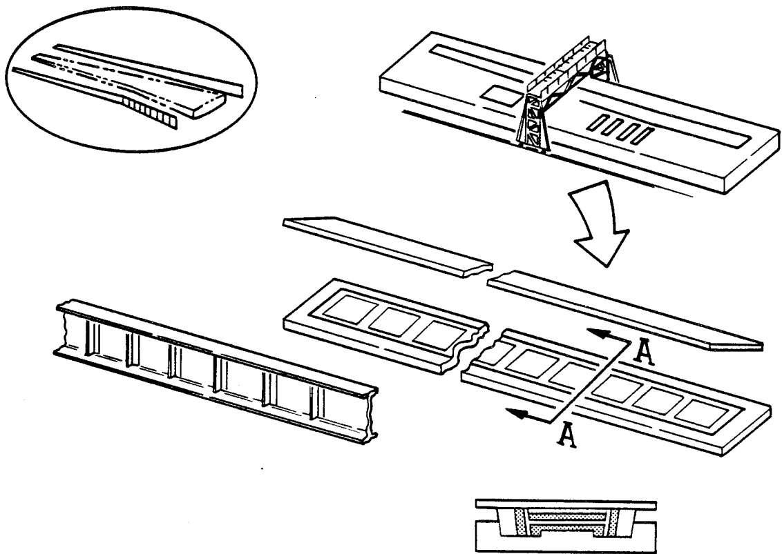
Figure 53. Wing Spar Manufacturing Approach
