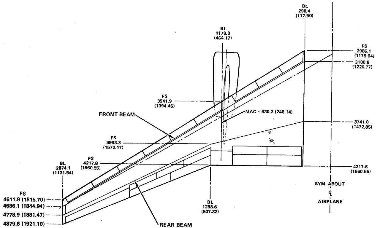
Figure 7. Wing Characteristics of Baseline Airplane
