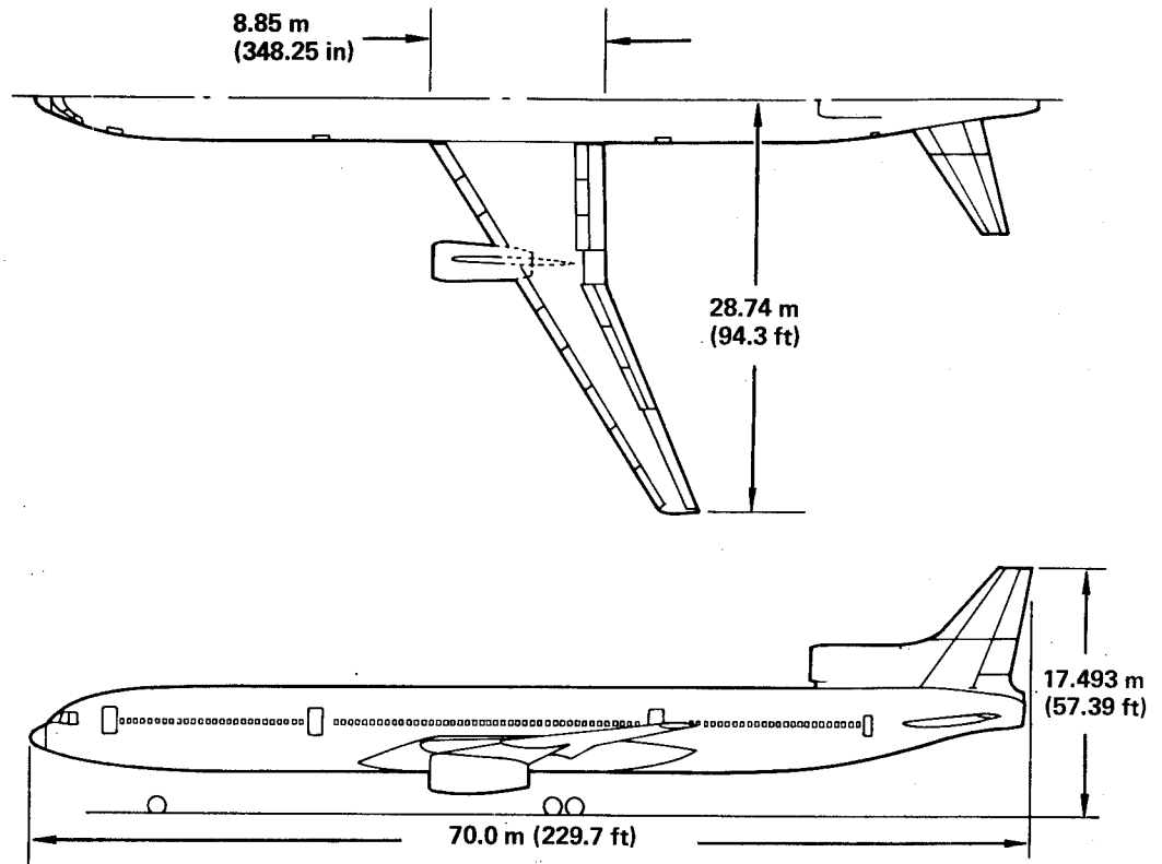
Figure 6. General Arrangement - Baseline Airplane
