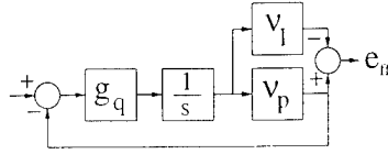
Fig. 14. Feedforward Interconnection
