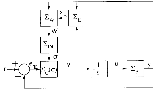
Fig. 15. Supervisory Control System Using Dwell-Time/Cyclic Switching
