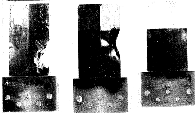
Figure 29 Results of Spin Impact Testing of Hybrid Composite and Titanium Alloy Simulated Blades
