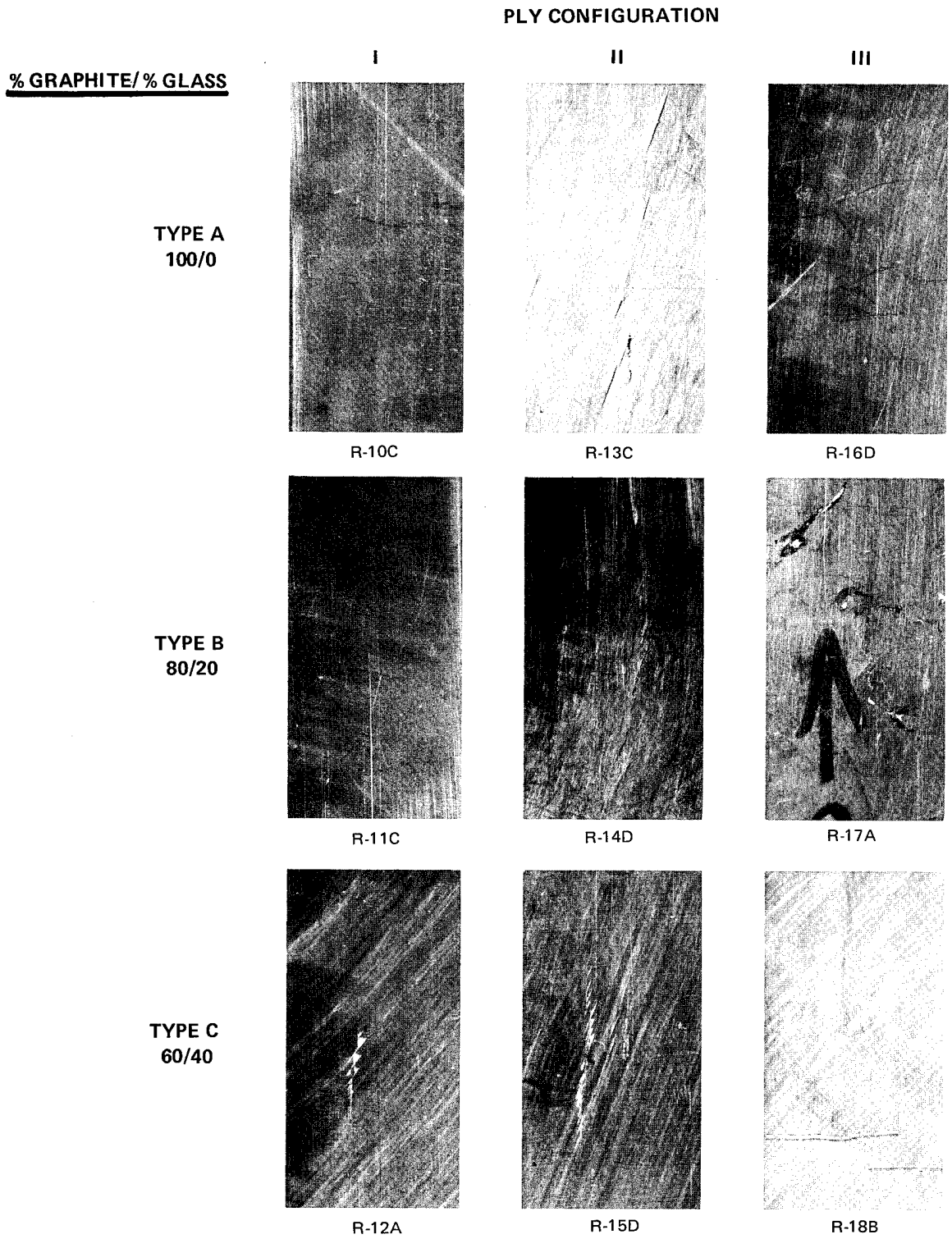
Figure 2 Damage to the Back Face of 5 x 23 cm Flat Panels When Impacted with 1.27 cm Diameter Gelatin Balls at a Velocity of 215 m/sec
