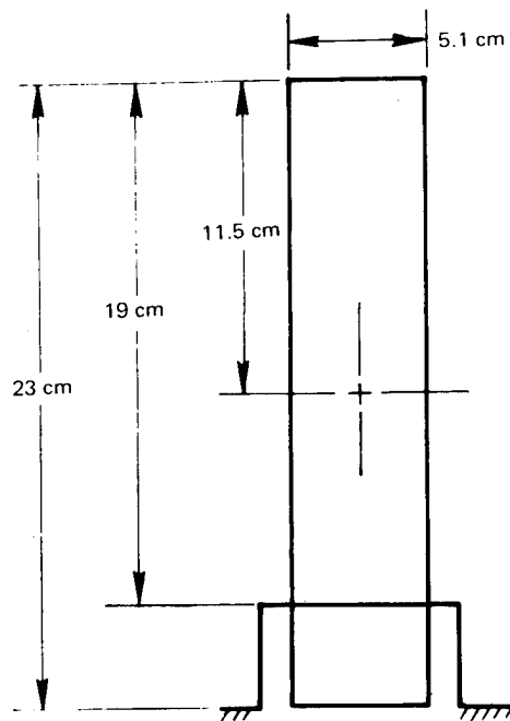
(b) HOLDER
