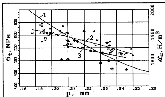
Fig. 1. Unit weight \alpha_c (1) and actual tension failure stress \sigma_t of unnotched specimens cut from sheets (2, small points) and from helicopter rotor blade spars (3, large points) versus per ply thickness of glass/epoxy.
