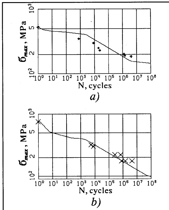
Fig. 18. The experimental results and analytical fatigue curves for carbon/glass/epoxy composite under tension-tension cycle. \dot{\sigma} = 4000 MPa/s;
