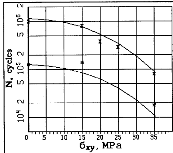
Fig. 19. The dependence of fatigue life on the minimum tangential cycle stress for the unnotched glass/epoxy tubular specimens and carbon/glass/epoxy specimens for conditions of in-phase compression and torsion ( r = -\infty ): 1) glass/epoxy: layup [0]8, \sigma_{min} = -355 MPa 2) carbon/glass/epoxy: layup [O_{gl}/O_{gr}/O_{gl}/O_{gr}]_s , \sigma_{min} = -390 MPa *) stress corresponds to the nominal values of the per ply thickness 0.3 mm for all plies.
