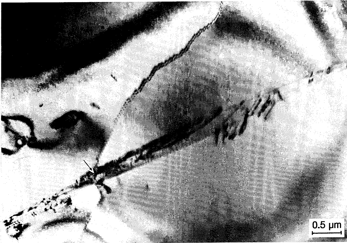
Figure 54. Slip band pileup at GB (arrow), nucleating slip band in adjacent (left) grain.
