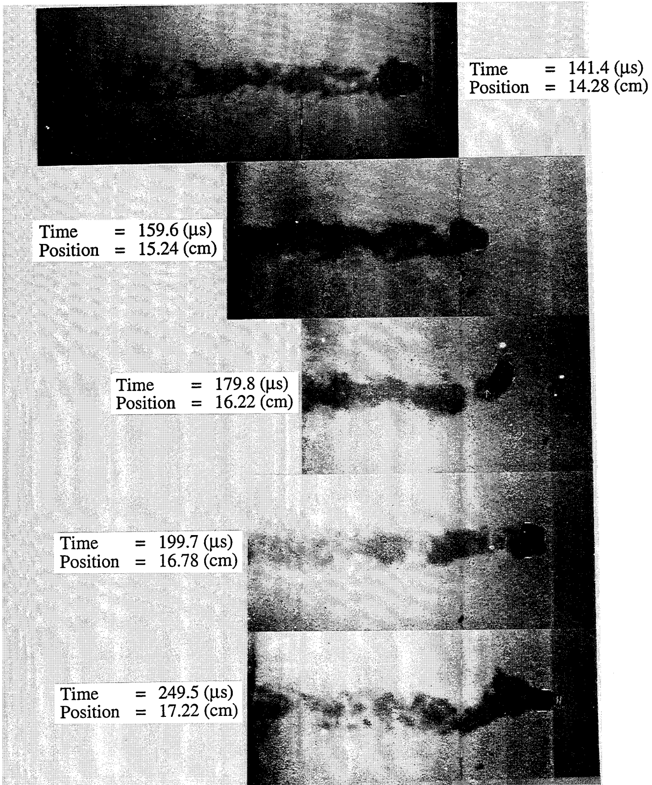
Figure 28. Flash X-rays of tungsten-alloy projectile penetrating glass targets ( V_p = 1.70 km/s) (Cont'd)
