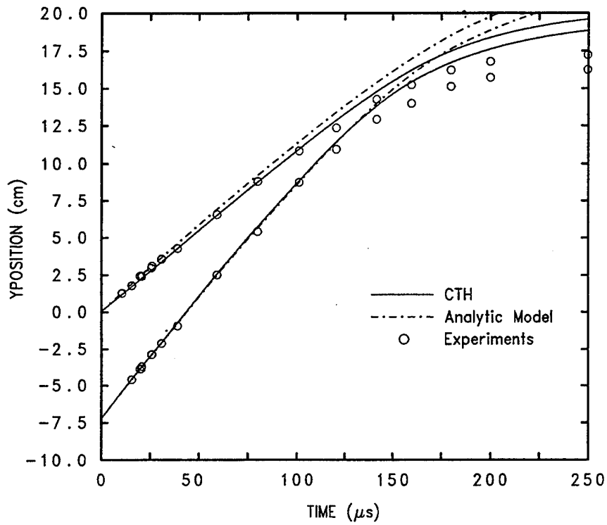
Figure 38. Mohr-Coulomb glass model ( Y_o = 0 , \beta = 1.0 ): V_p = 1.70 km/s
