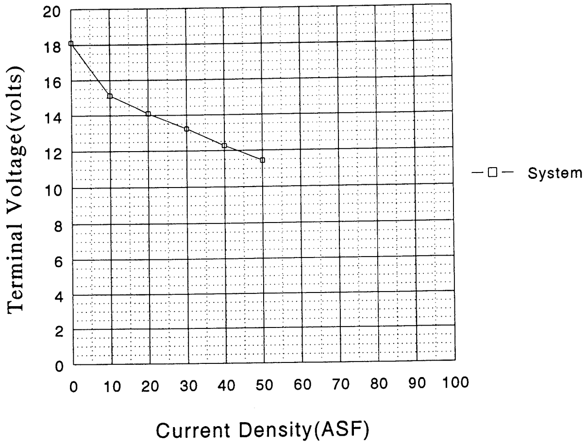
Figure B-8. Performance of H 2 /Air PEM Fuel Cell (9322-1435, 19-Cell Stack)
