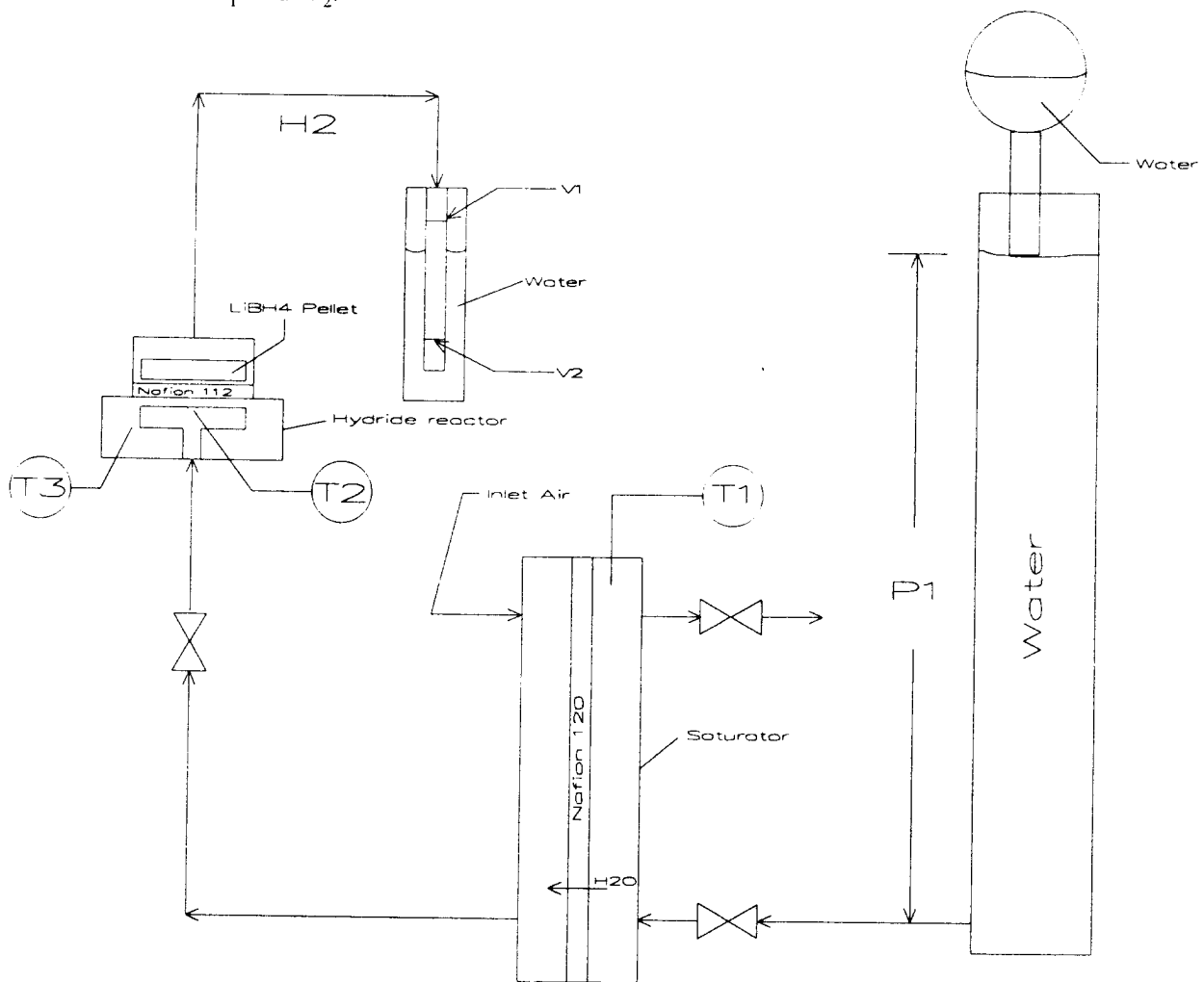
Figure 4. Experimental Setup
