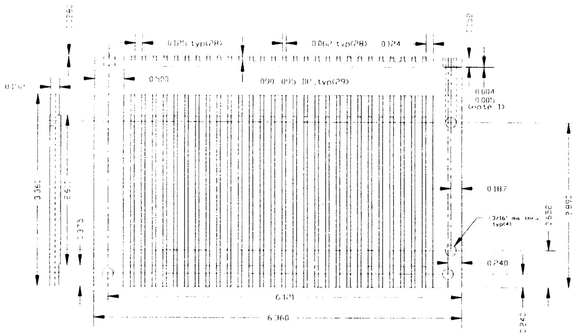
Figure 18. Cathode Collector
