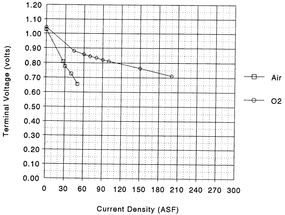
Figure B-1. H 2 /Air, O 2 PEMFC Performance (Cell #3, 9322-2294)
