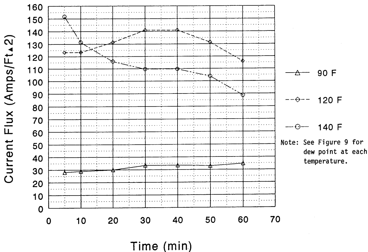
Figure 8. Effect of Dew Point on a 1.0-g LiBH 4 Reactor System
