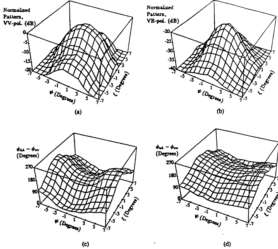
Fig. 5. Polarimetric response of a metallic sphere over the entire mainlobe of X -band scatterometer; normalized \sigma_{vv} (a) corresponds to G_v^2 and normalized \sigma_{vh} (b) corresponds to G_v G_h ; phase difference between copolarized (c) and cross-polarized (d) components of the sphere response correspond to phase variation of the co- and cross-polarized patterns of the antenna.
