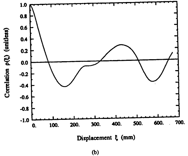
Fig. 3. Typical results of surface characterization of one of the surfaces measured in this study: (a) Histogram of measured heights for a slightly rough surface and the Gaussian probability distribution used to model it; a total of 4353 height measurements were made, from which the rms height was calculated to be s = 6.9 mm. (b) Measured autocorrelation function of the same surface.
