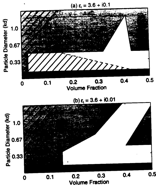
Figure 14: TM polarization validity regions based on 20% differences between imaginary \epsilon_{\text{eff}} for the numerical method of determining \epsilon_{\text{eff}} (NUM-PY) and the theoretical methods of QCA-PY (light gray), EFA (hatched) and PVS (dark gray) for (a) \epsilon_i = 3.6 + i0.1 and (b) \epsilon_i = 3.6 + i0.01 .
