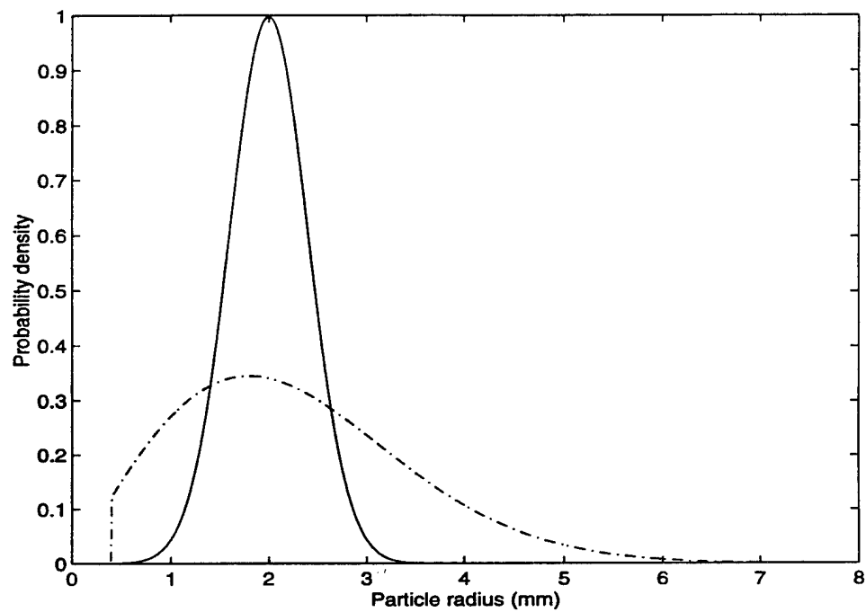
Figure 10: Gaussian (solid line, - ) and truncated Rayleigh (dot dashed line, .- ) Probability distribution functions of particle radii used in the packing algorithm. Both distributions have the same mean.
