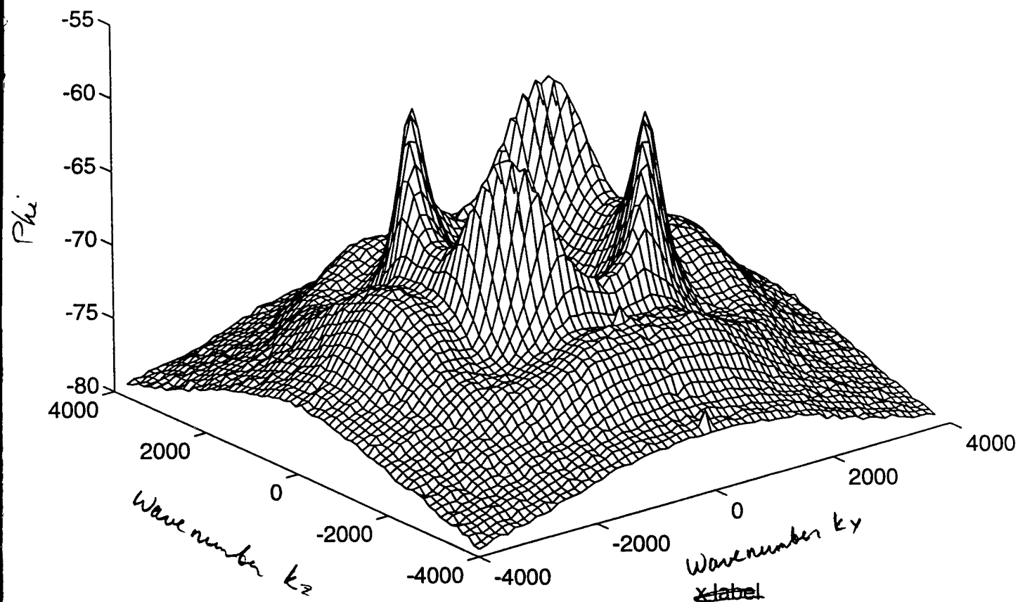
Figure 9: The power spectral density derived from data shown in Fig. 4. Strong peaks along the diagonal highlight the periodicity in the correlation function seen along this axis. Arcs drawn along a constant radius are proportional to the backscatter intensity as a function of incidence angle.
