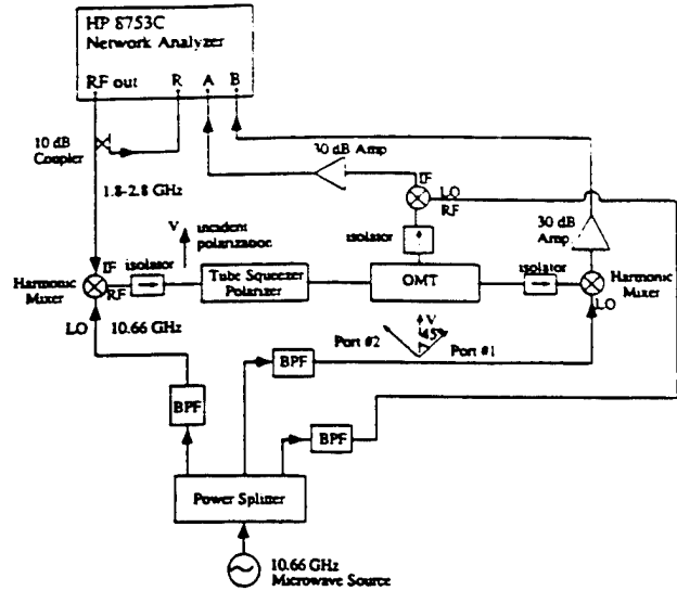
Fig. 3. Experimental setup for tuning and characterizing the prototype K -band squeezed waveguide polarizer.
