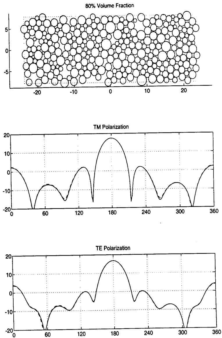
Figure 3: Algorithm results for 80% volume fraction. See Fig. 2 for description of individual sub-figures.
