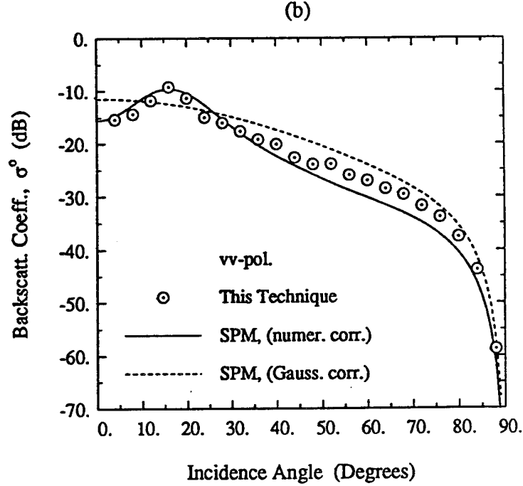
Figure 5: Backscattering coefficient \sigma^\circ of the random surface with ks = 0.12 , kl = 2.13 , and \epsilon_1 = \epsilon_2 = 15 + i3 as computed by the SPM and the numerical technique; (a) hh -polarization and (b) vv -polarization.
