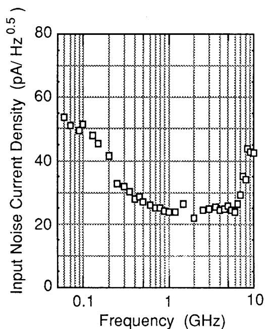
Fig. 5. Input noise current density of the WGPD-HEMT.
