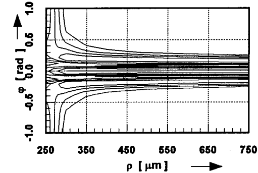
Fig. 4b 3rd mode (cylindrical coordinates)
