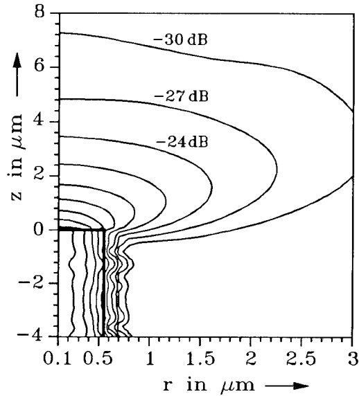
Figure 1: Norm of the Poynting vector in dB
