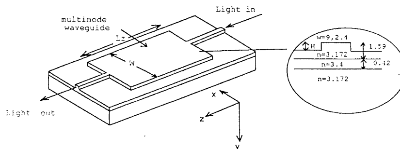
Fig. 1 Schematic diagram of a MMI recombiner. [The insert shows the waveguide cross-section and all dimensions are in \mu\text{m} .]
