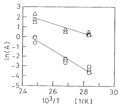
Fig.4 Arrhenius' plots of the drift rates ( A_s ) against the logarithmic time scales of Fig. 3 ; i.e. Applied Voltage = A \log(\text{Time} / \text{hr}) + B . The circles denotes the rates below the 100-hr-operations, and the triangles for the rates beyond 100 hr.
