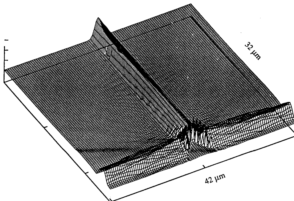
Fig. 2. Beam splitting symmetrically into two guides. Two 45° angled mirrors are used at the joint.
