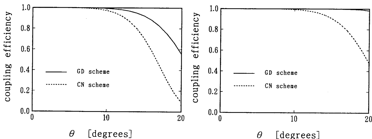
Fig.2 Coupling efficiency as a function of tilt angle \theta
