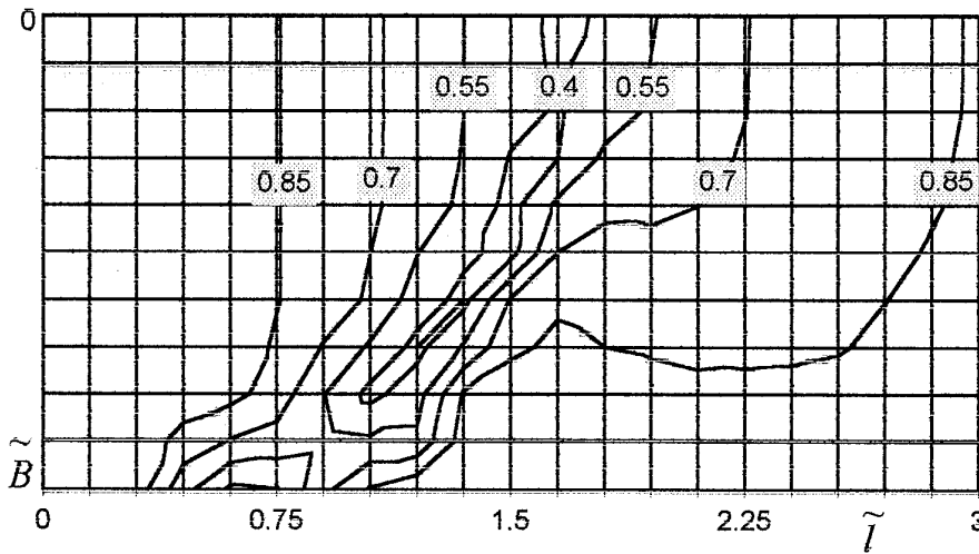
Fig. 7. Bottom deformations along and across the estuary area (the flow plan model). (k_T = 0.6, a_I = 1.0, E = 1.0, t = 1.8)
