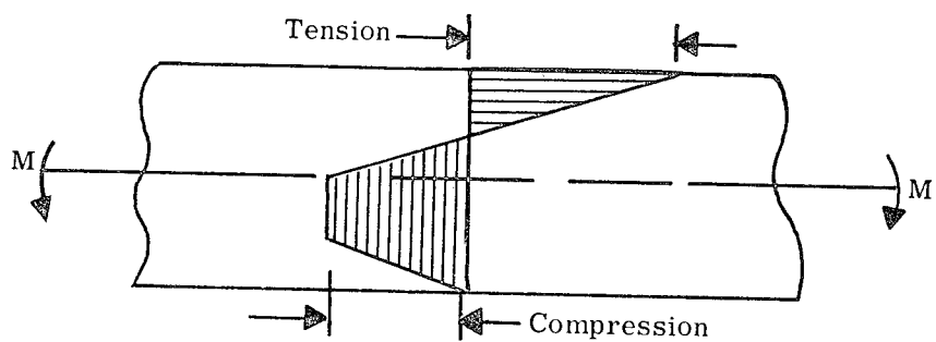
Superimposed stress
