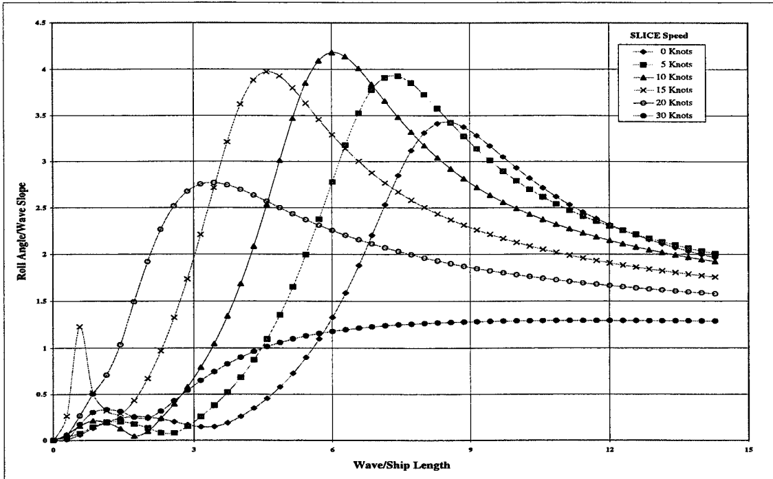
Figure (92). Roll Characteristics as a Function of SLICE Speed, 60 Degree Wave Angle.
