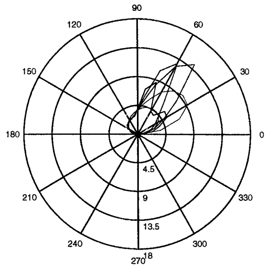
Figure(126). Roll Characteristics, Sea State 5.
