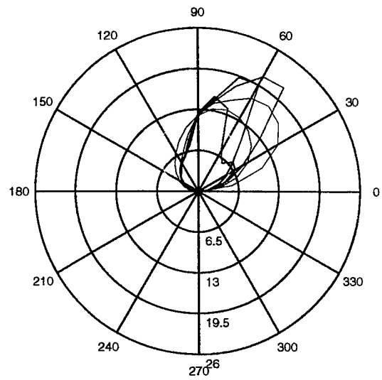
Figure(128). Roll Characteristics, Sea State 7.
