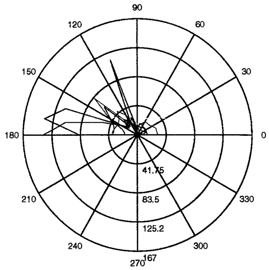
Figure(121). Pitch Characteristics, Sea State 6.
