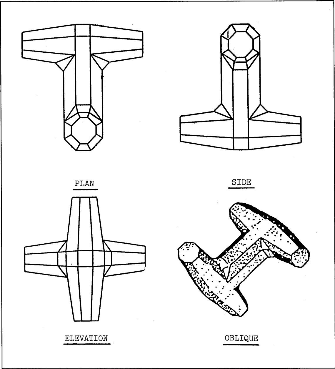
Figure 6. Various views of a dolos armor unit
