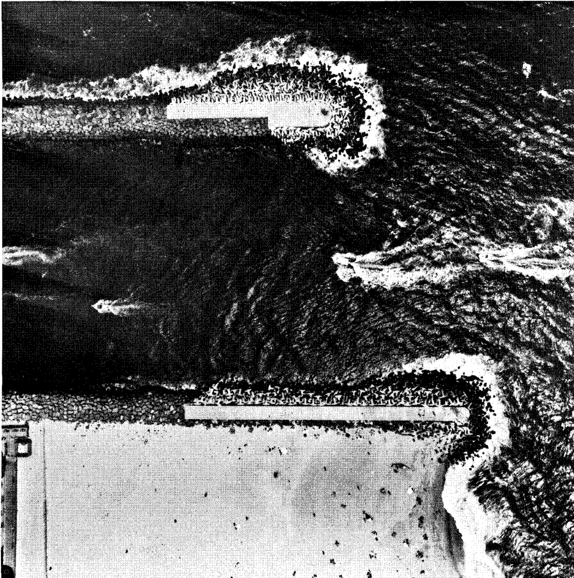
Figure 17. Stereo pair photograph for Manasquan Inlet jetties (middle photo image)
