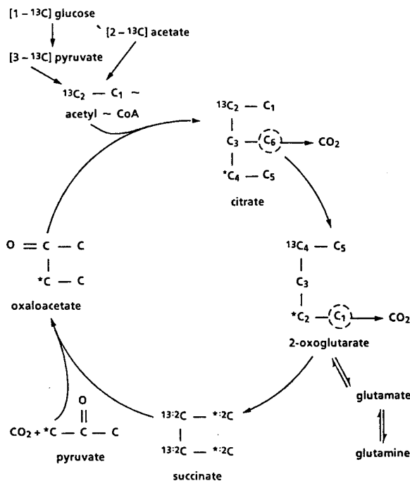
FIG. 1. A simplified scheme of the TCA cycle shows the conversion of [1- ^{13}\text{C} ] glucose and [2- ^{13}\text{C} ] acetate to [2- ^{13}\text{C} ] acetyl-CoA and hence the labeling of the C-2 position in citrate and the C-4 position in 2-oxoglutarate. Because succinate is symmetrical, the label is distributed equally between the C-2 and the C-3 positions (symbolically 13:2) before formation of oxaloacetate. [1- ^{13}\text{C} ] Glucose yields [3- ^{13}\text{C} ] pyruvate, which also may form oxaloacetate after carboxylation. This produces C-2-labeled oxaloacetate (asterisk represents ^{13}\text{C} ). In succinate this label is distributed equally (*:2) between the C-1 and C-4 positions.
