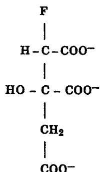
Figure 2.3 Fluorocitrate
