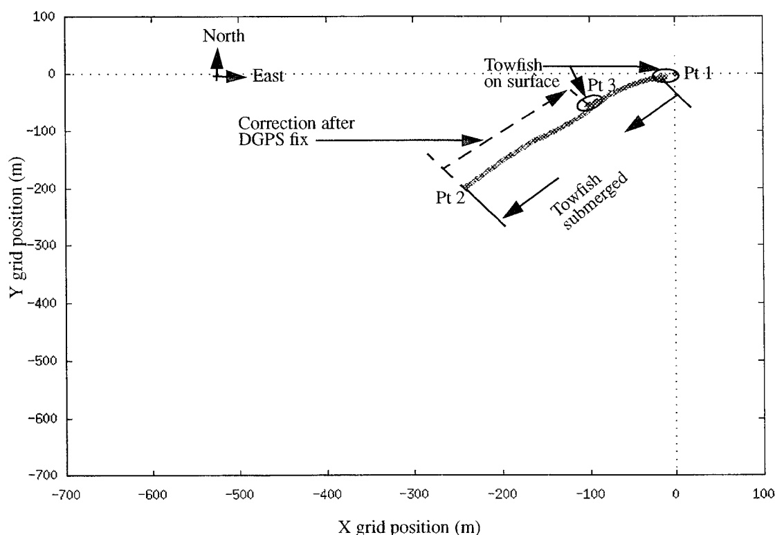
Figure 22: Sea test results of first two DGPS fixes
