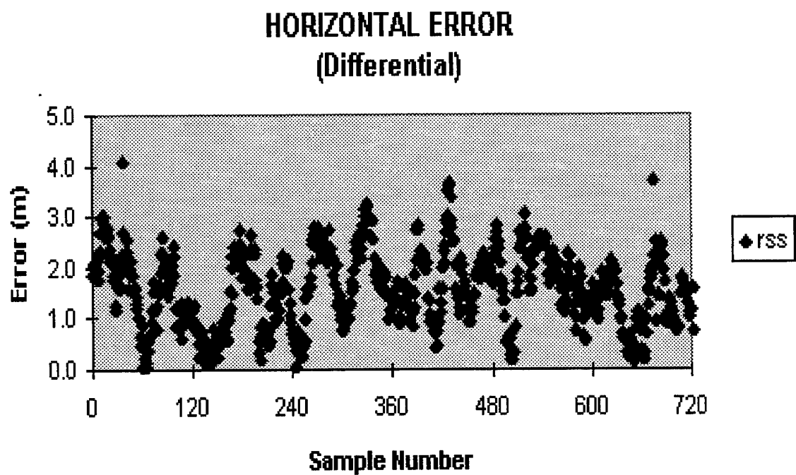
Figure 9: GPS bench test results(1 hour at 5 second intervals)
