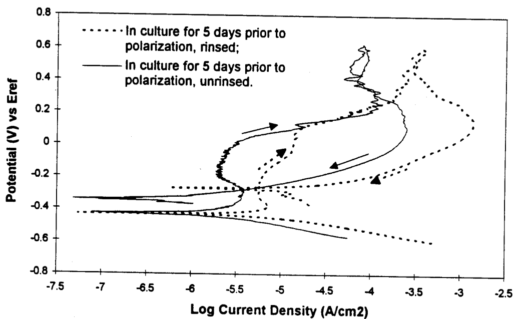
Figure 4b. The role of biofilm in the passivation performance of the SRB exposed 317L SS shown in the polarization diagrams in 0.1 M HCl.
