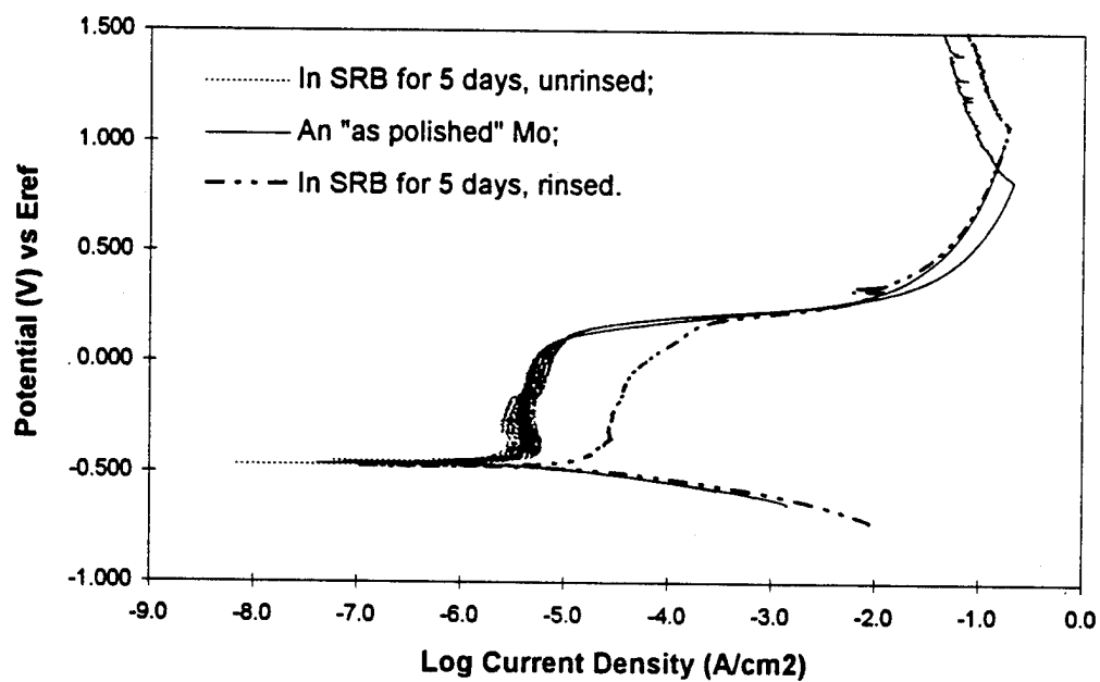
Figure 37. Potentiodynamic polarization diagrams of the SRB-exposed pure Mo coupons in deaerated 0.1 M HCl.
