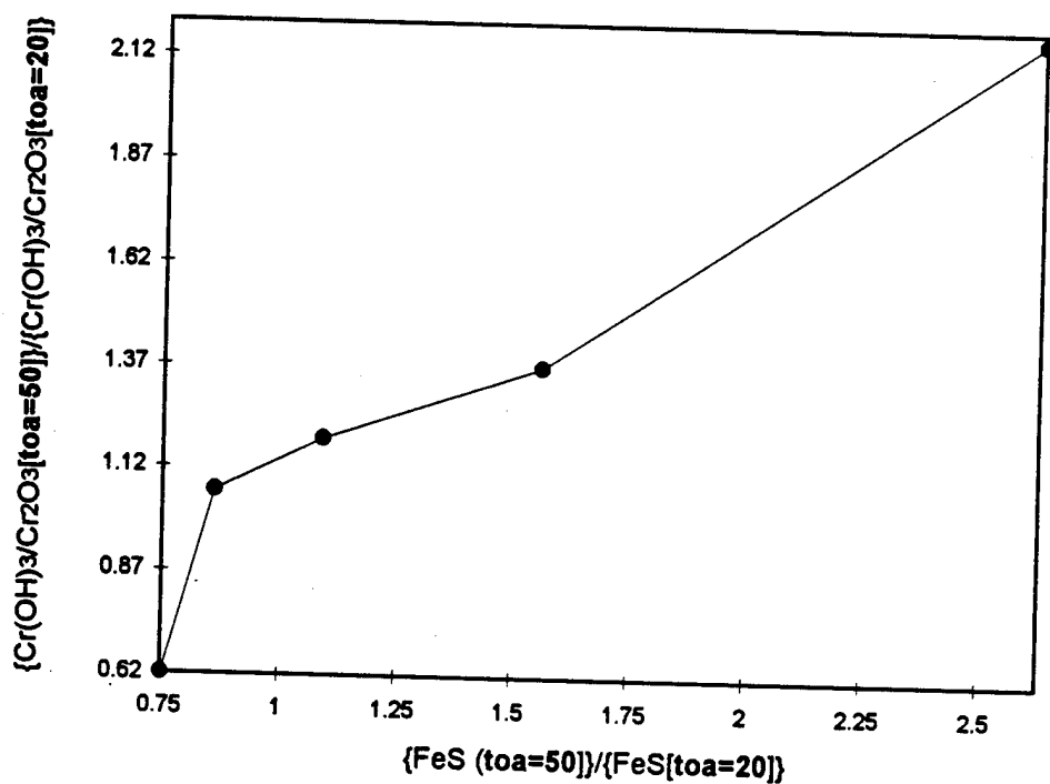
Figure 21. The ratios of the relative proportion of Cr(OH)_3 to Cr_2O_3 in the inner region to the one in the outer region vs the variable sulfidation with the depth of the surface films of SRB-exposed 304 SS coupons determined by variable angle XPS after the potentiostatic polarization in the hydrochloric solution.
