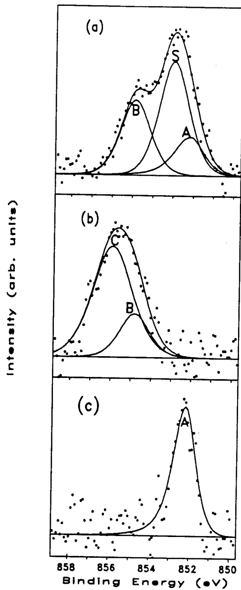
Figure 10. Ni 2 p spectra from the surfaces of 304 SS, TOA: 20°. (a) In SRB for 5 days, rinsed; (b) A control sample; (c) "As polished"
